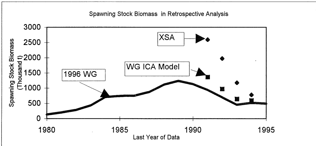
Figure 1.5.1. North Sea Herring. Estimates of spawning stock size and fishing mortality estimated by the 1996 Working Group (Bold Line). Square markers, estimates of fishing mortality and stock size in the last years of retrospective analyses made using the Working Group's assessment model. Diamond markers, estimates of fishing mortality and stock size in the last years of retrospective analyses made using the 'XSA' method. No shrinkage used in either method.
