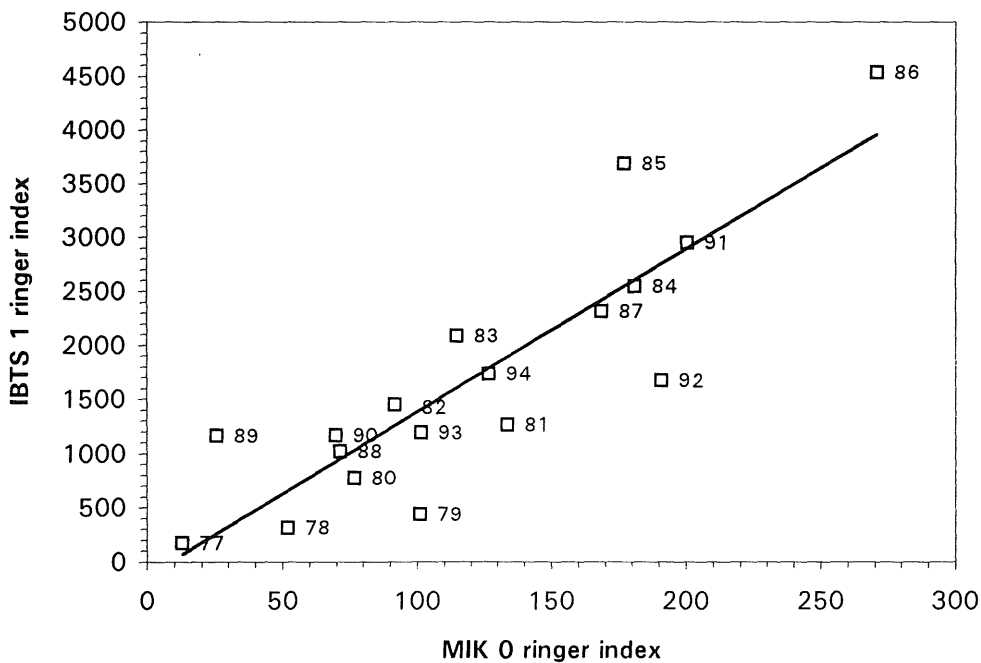
Figure 2.3.5 The IBTS 1-ringer index regressed against the MIK 0-ringer index. Year classes 1977 to 1994.
