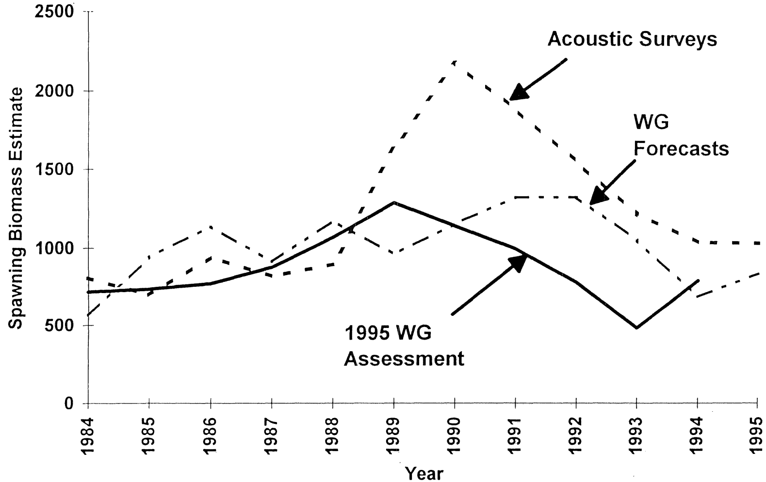
Figure 2.14.1 Discrepancy between the predicted and estimated spawning stock biomass. Solid line represents the spawning stock biomasses estimated at the 1995 Working Group meeting. The broken line 'WG Forecasts' represent the forecasts made by the Herring Assessment Working Group from 1982 - 1993. The 'Acoustic Surveys' have indicated a spawning stock biomasses over the period 1989 - 1995, which are double those calculated than those calculated by the assessment.
