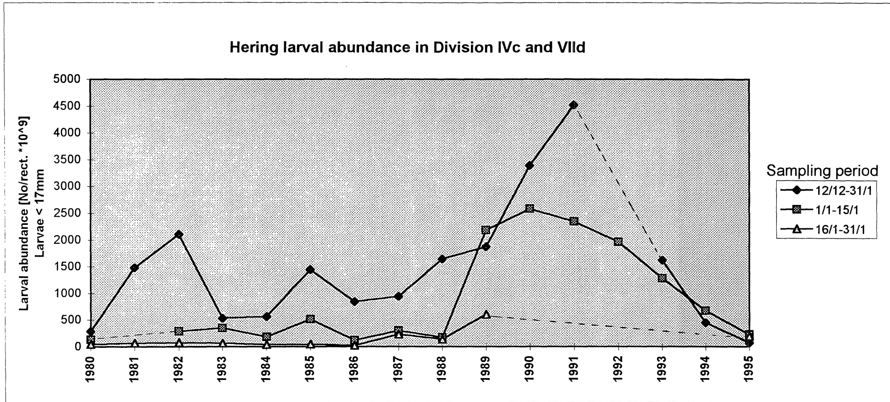
Figure 2.8.21 Herring larval abundance in Divisions IVc and VIId during the period 1980 - 1995
