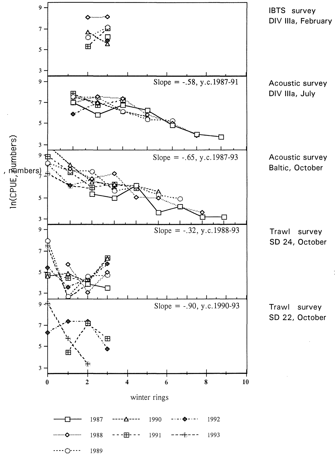
Figure 3.9.1. Age disaggregated indices in ln(numbers) by age and yearclass for spring spawning herring in Div. IIIa and SD 22,23 and 24 .
