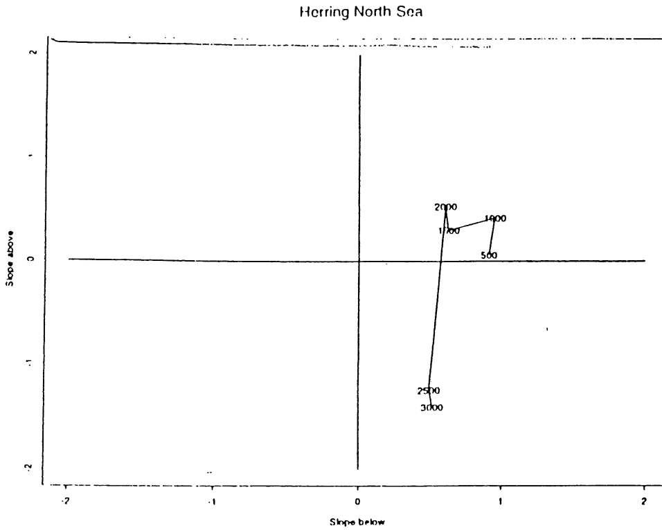
Figure 2.9.3. Diagnostic sheet for estimating MBAL. The slope of the stock-recruitment data above and below the MBAL estimate (from Anon 1993).
