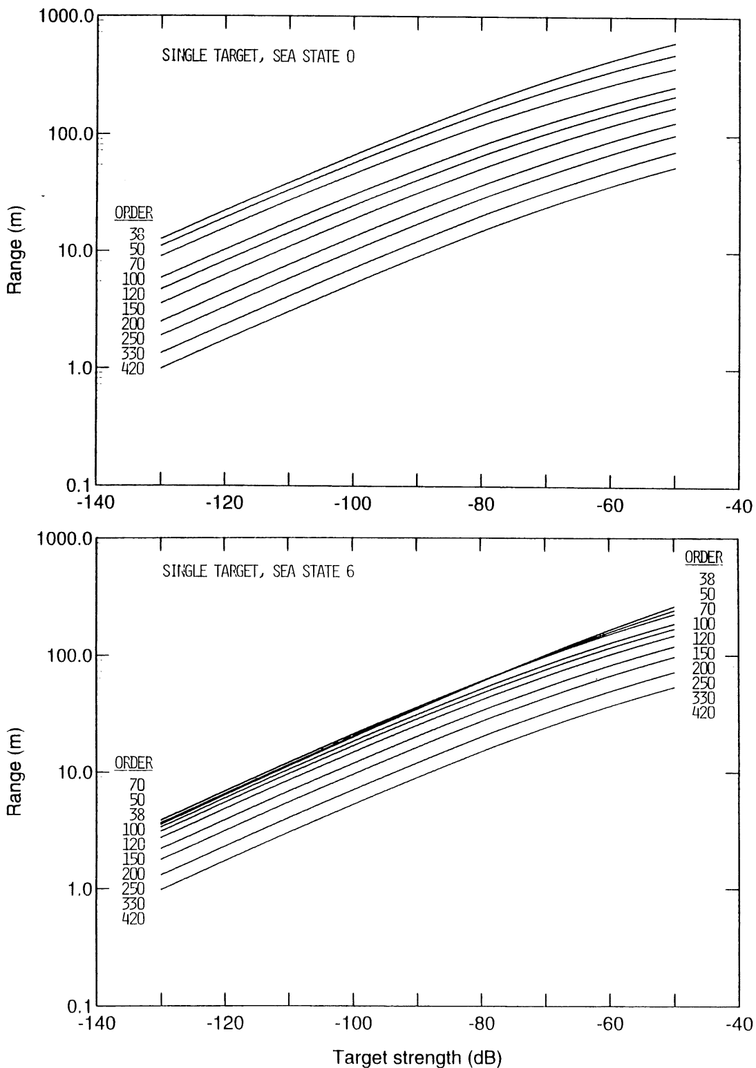
Figure 1. Maximum detection ranges of single targets for the described system design, assuming detection threshold of 20 dB.
