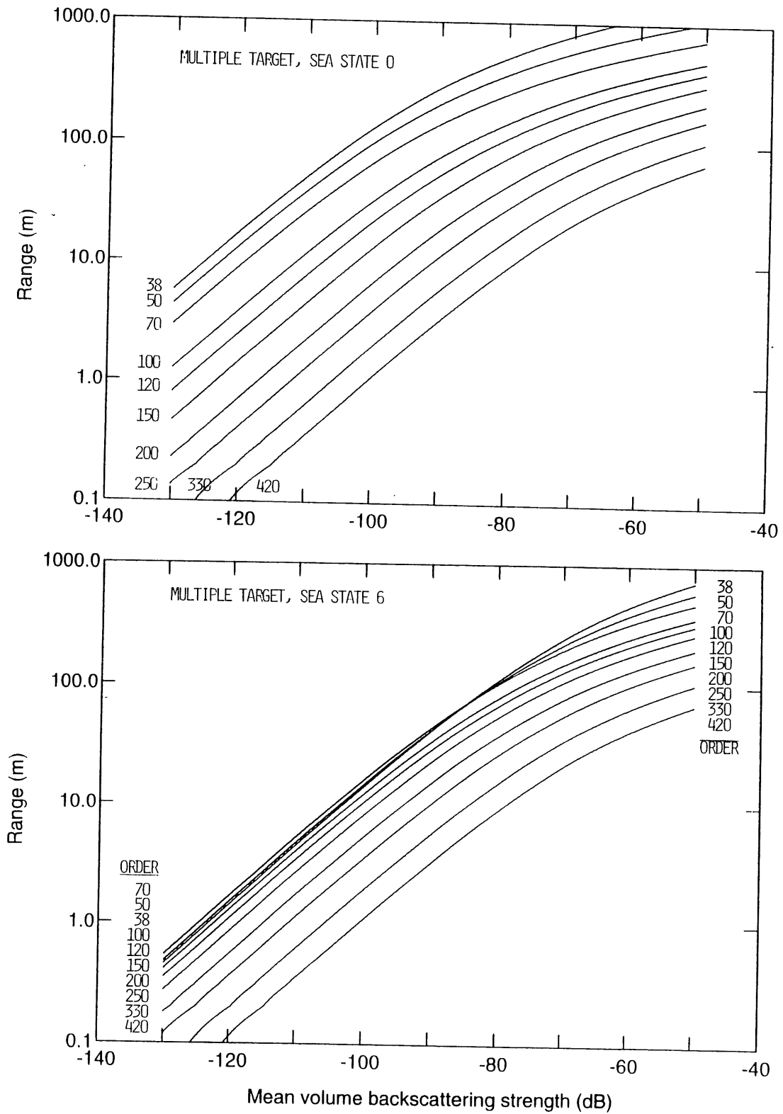
Figure 2. Maximum detection ranges of multiple targets for the described system design, assuming detection threshold of 20 dB.
