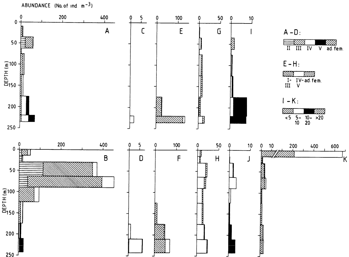
Fig. 9. Vertical profiles of dominating zooplankton species from station 829 (above) and 878 (below). A-B: Calanus finmarchicus ; C-D: C. hyperboreus ; E-F: Metridia longa ; G-H: Pseudocalanus sp.; I-J: Chaetognats; K: Euphausiids. Key to copepodite stages and length (mm) groups at upper right.
