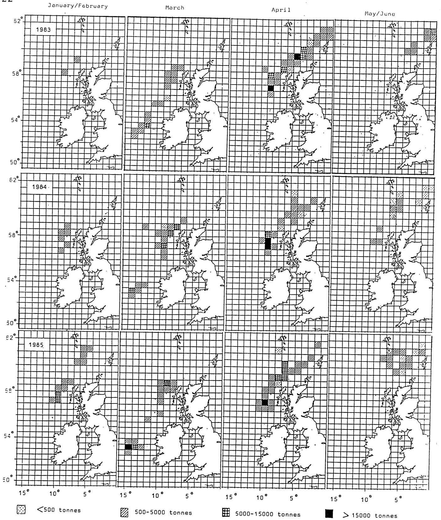
Fig. 3B. Progress of the Norwegian blue whiting fishery in the spawning area, 1983 - 1985.
