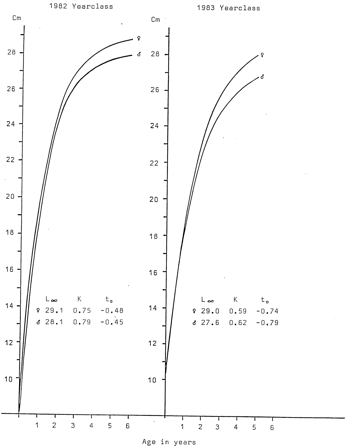
Fig. 17. von Bertalanffy's growth curves and parameters based on backcalculated lengths of the 1982- and 1983-yearclasses in their 6 and 5 first years of life respectively as appearing in the Hebrides area.
