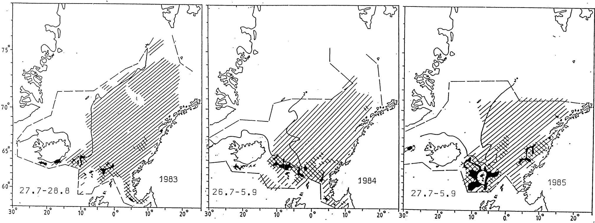
Fig. 6B. Distribution and densities of blue whiting with 2 o C - isoline at 200 m depth, during summer 1983-1985. Symbols as in Fig. 6A.
