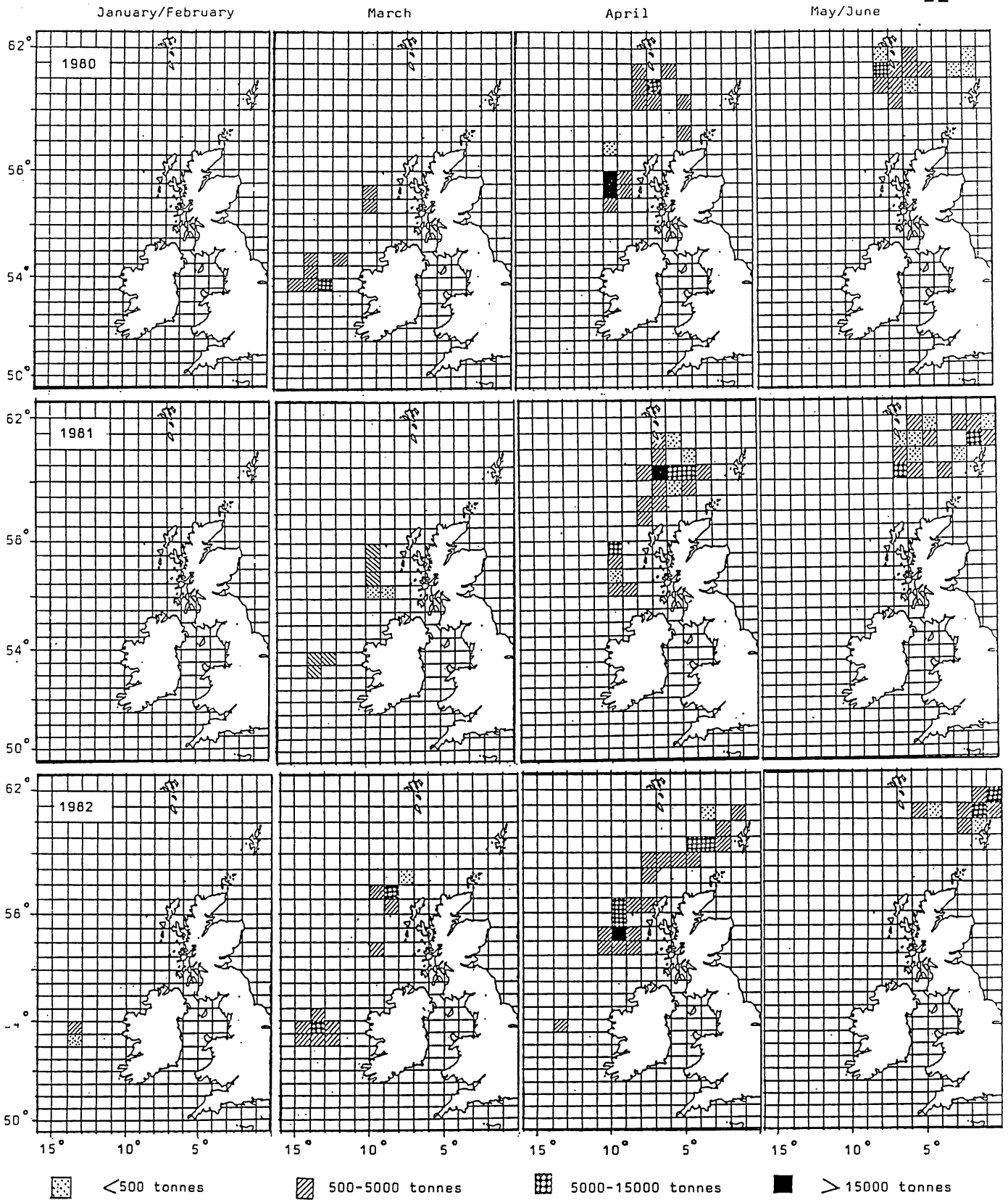
Fig. 3A. Progress of the Norwegian blue whiting fishery in the spawning area, 1980- 1982.
