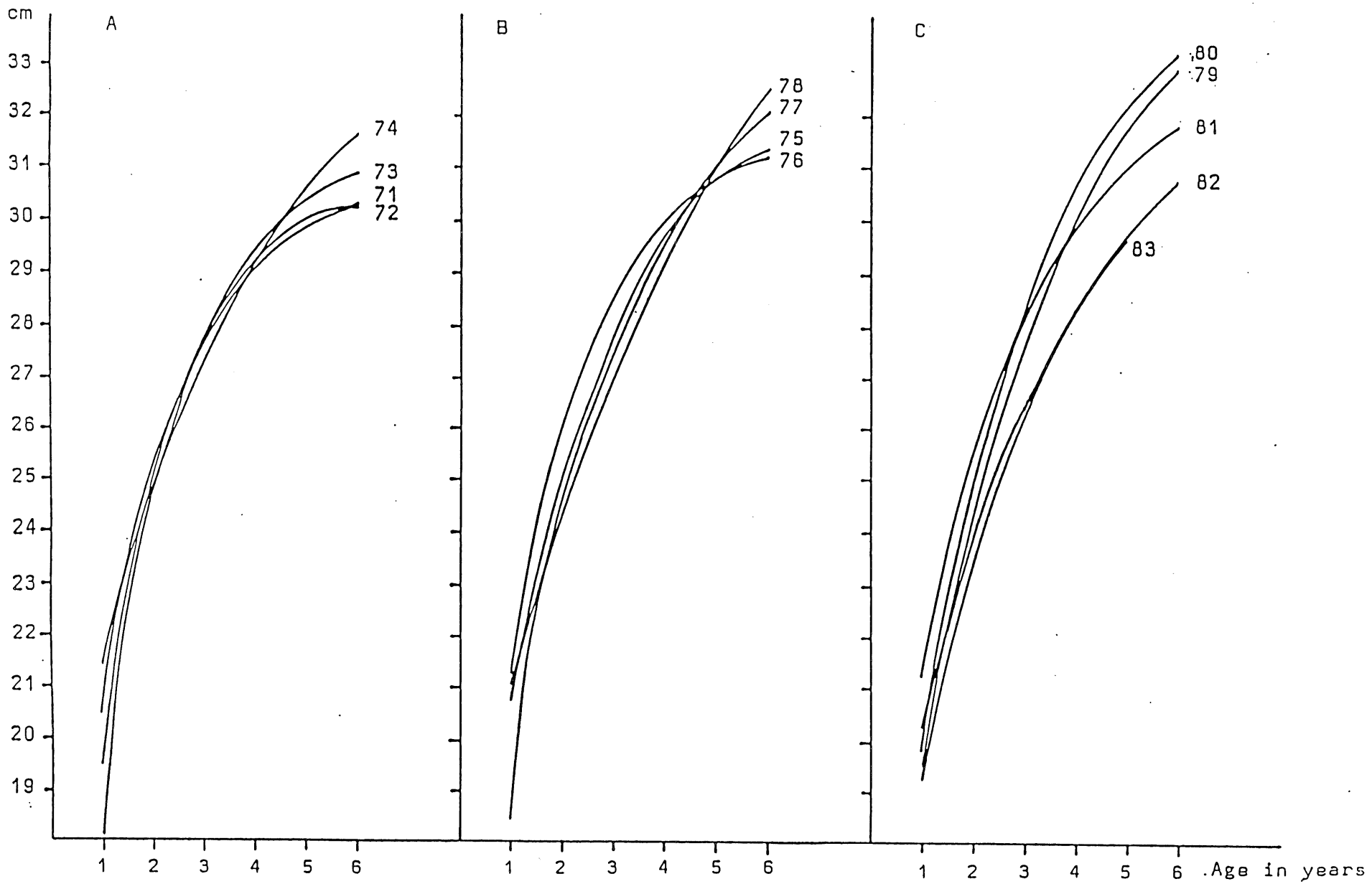
Fig. 11. von Bertalanffy's growth curves of blue whiting, combined sexes, for the six first years of life as appearing in the Hebrides area for A) the 1971-1974, B) the 1975-1978, and C) the 1979-1983 yearclasses.
