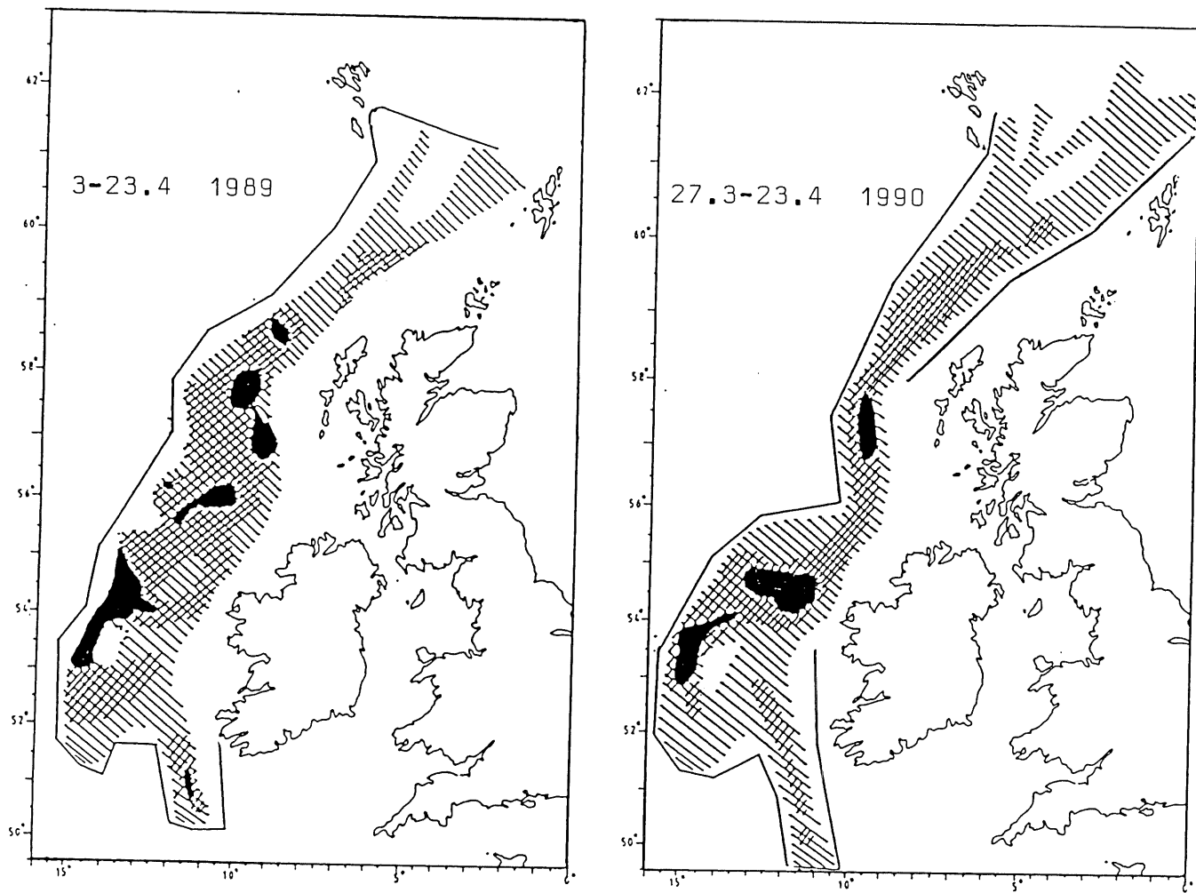
Fig.4D. Distribution and densities of blue whiting during spring 1989 and 1990. Symbols as in Fig. 4A.
