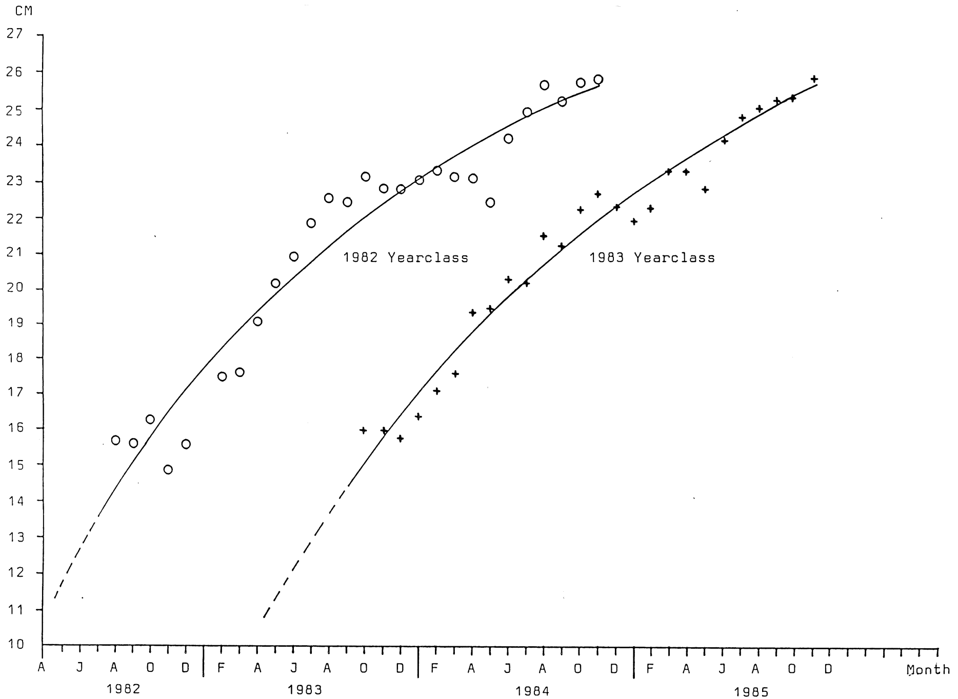
Fig. 14. von Bertalanffy's growth curves for the three first years of life of the 1982- and 1983-yearclasses, based on samples from the mixed industrial fishery in the North Sea.
