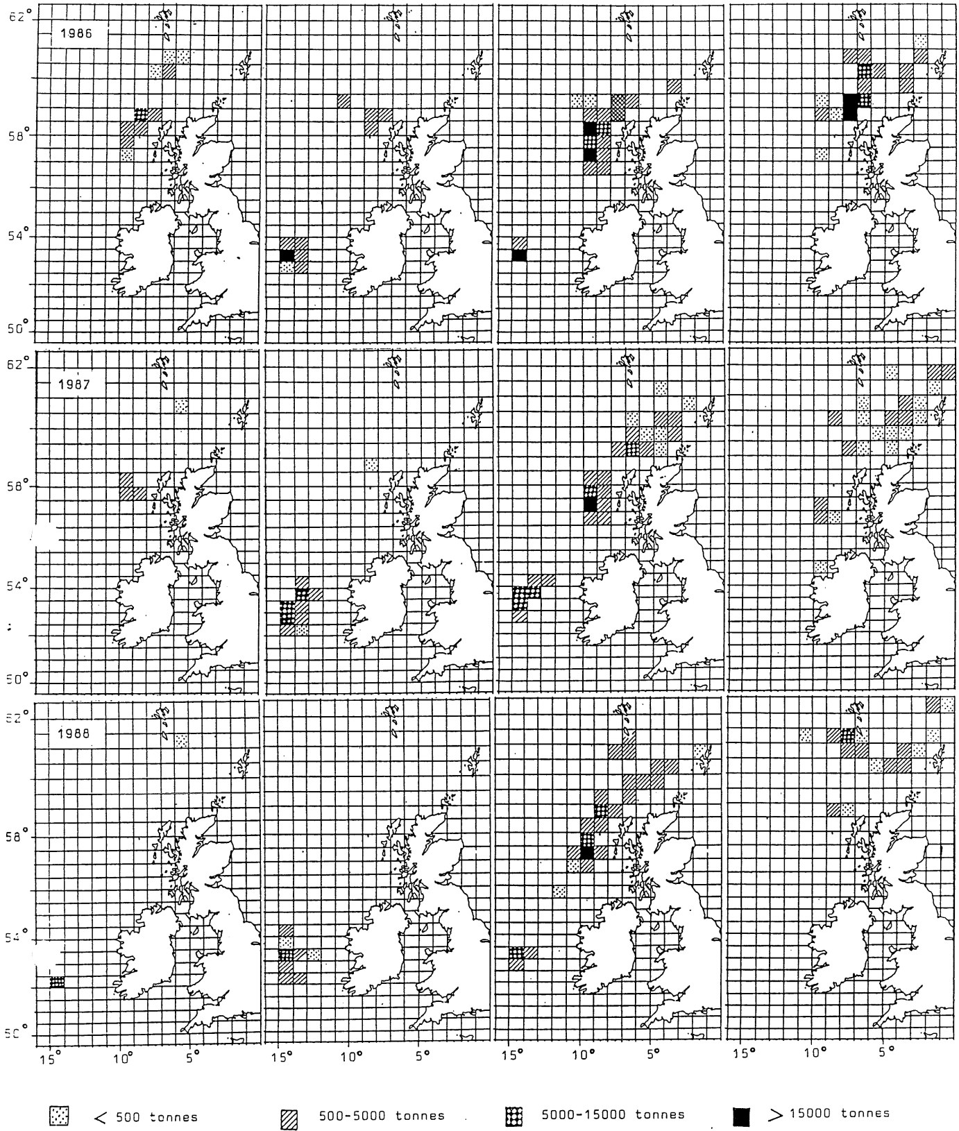
Fig. 3C. Progress of the Norwegian blue whiting fishery in the spawning area, 1986 - 1988.
