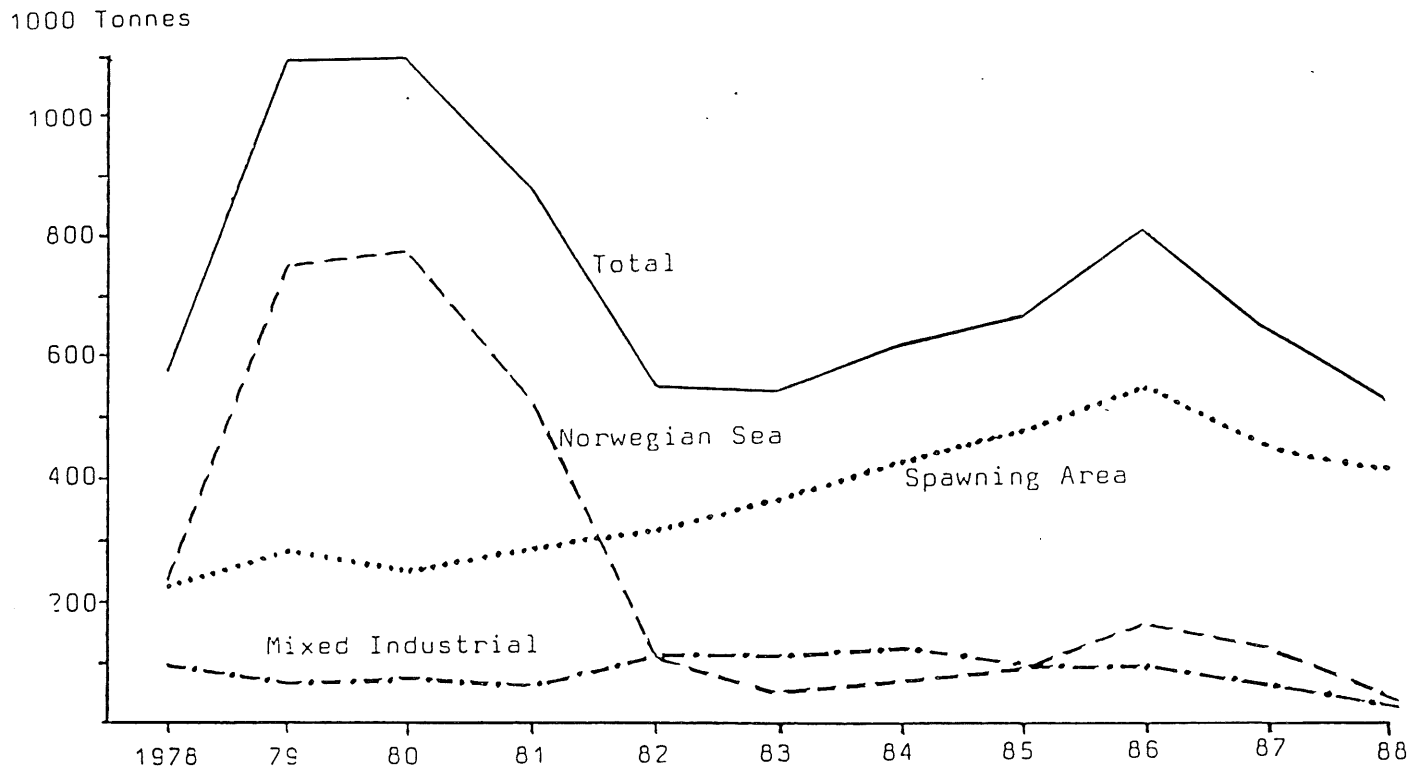
Fig. 1. Annual landings of blue whiting, from the main fisheries and total, of the northern stock, 1978-1987.
