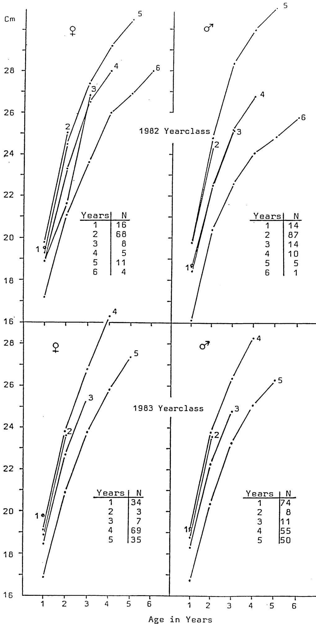
Fig. 18. Backcalculated fishlengths of blue whiting, males and females in the Hebrides area, separate for the 1 - 6 years age groups of the 1982-yearclass (upper half) and the 1 - 5 years age groups of the 1983-yearclass (lower half).
