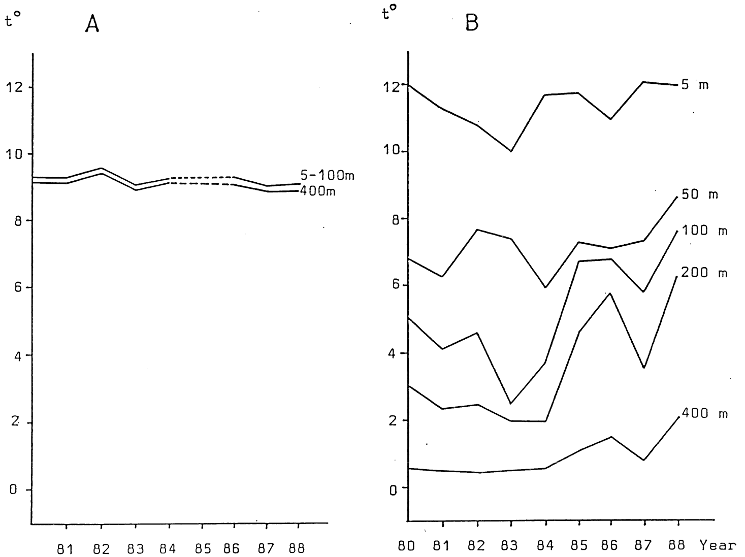
Fig. 5. Temperature trends at 5, 50, 100, 200 and 400 m depth for the period 1980 - 1988. A) In the spawning area west of the Hebrides in March/April near the position: 58° N 10° W. B) In the Norwegian sea in August at the outer station of the Svinøy-NW section, position: 64° 40' N 00° 00' E/W.
