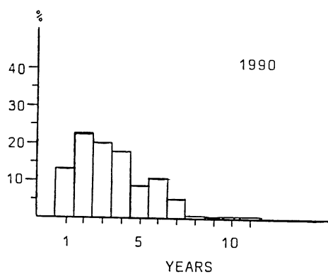
Fig. 7B. Age composition of the blue whiting stock in the spawning area, spring 1989 and 1990.
