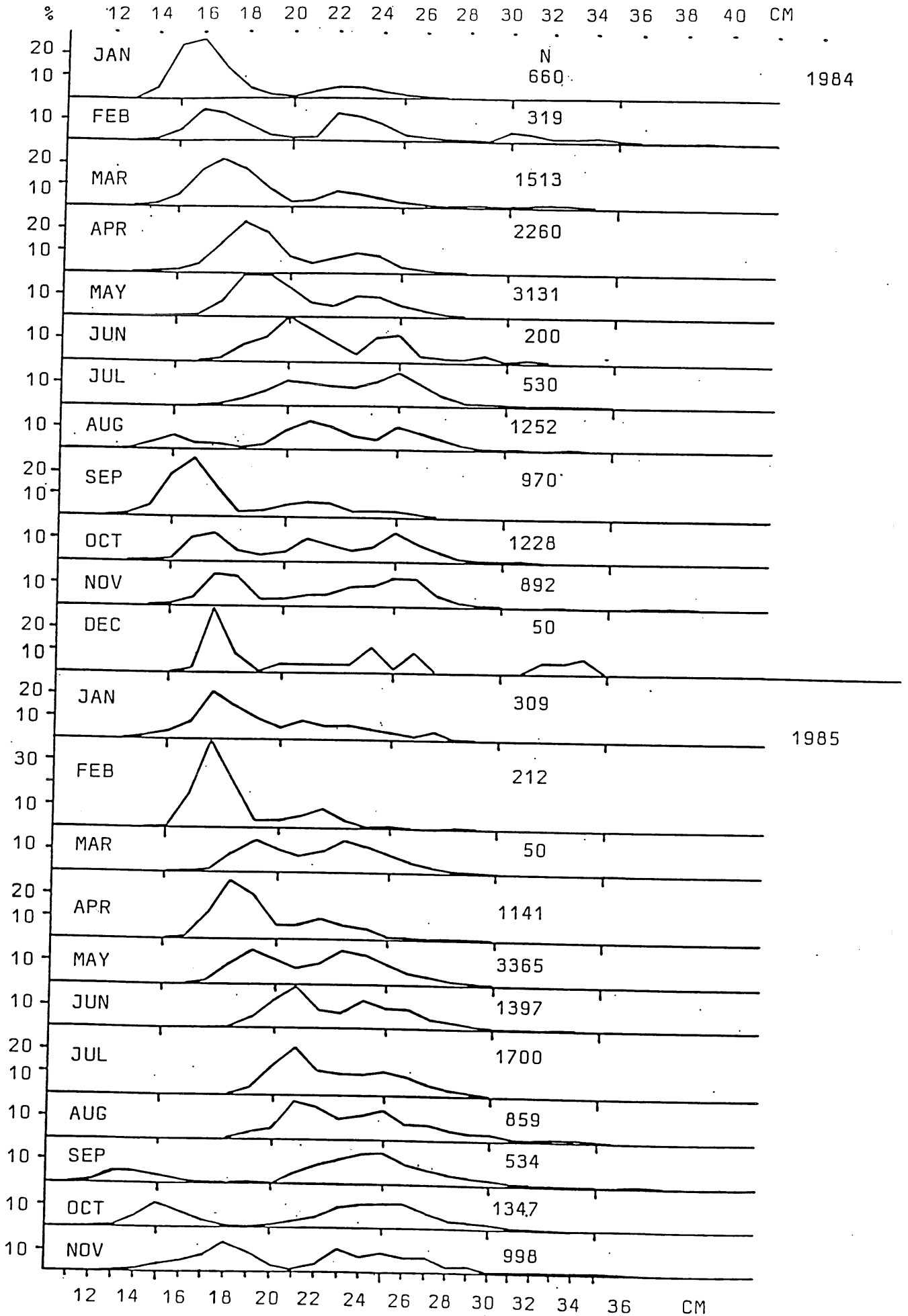
Fig. 13B. Length distribution (n%) by month of blue whiting in samples from the mixed industrial fishery in the North Sea, 1984 and 1985.
