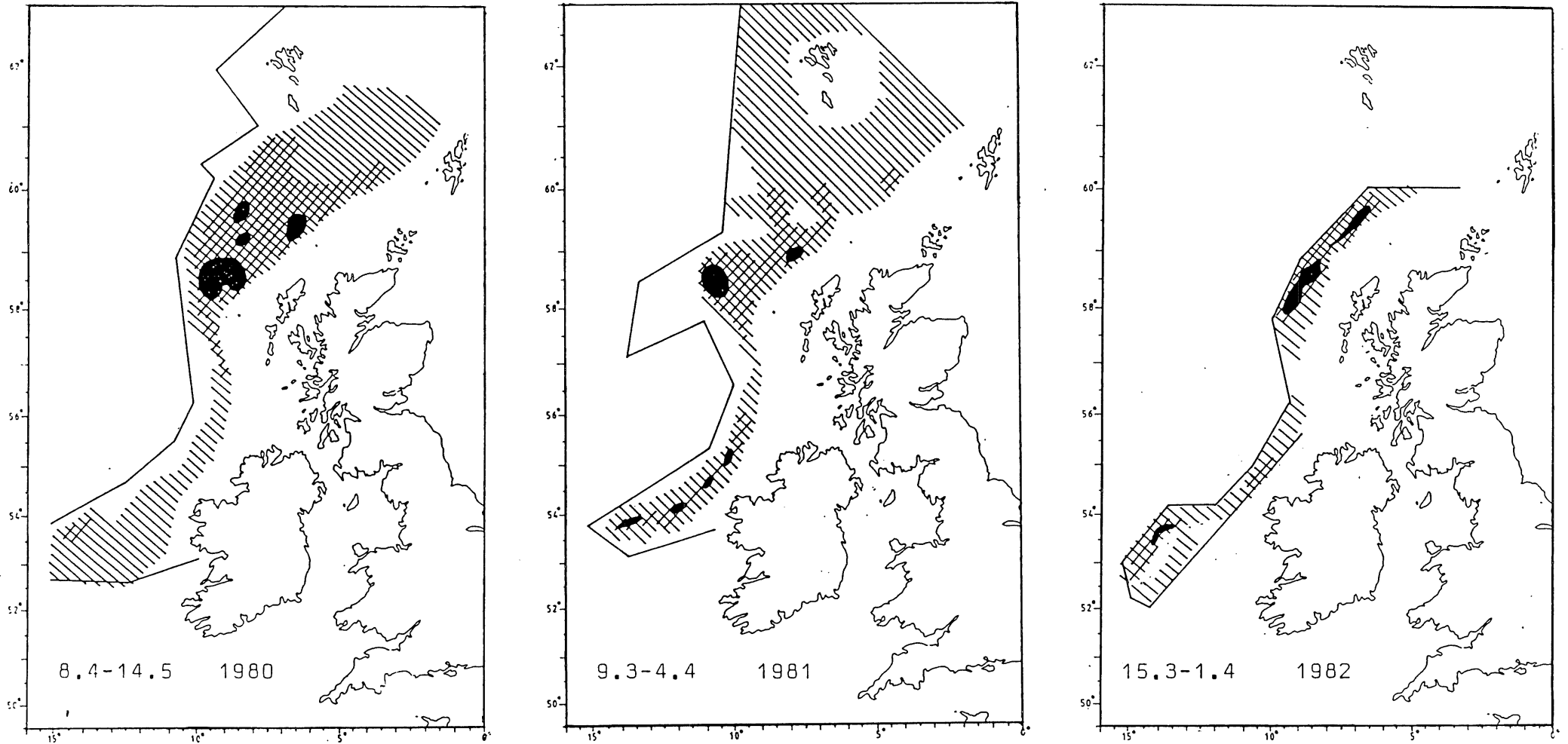
Fig. 4A. Distribution and densities of blue whiting during spring 1980-1982. Single hatch: area with scattered recordings, double hatch: dense recordings, black: very dense recordings. Full line indicates the area surveyed.
