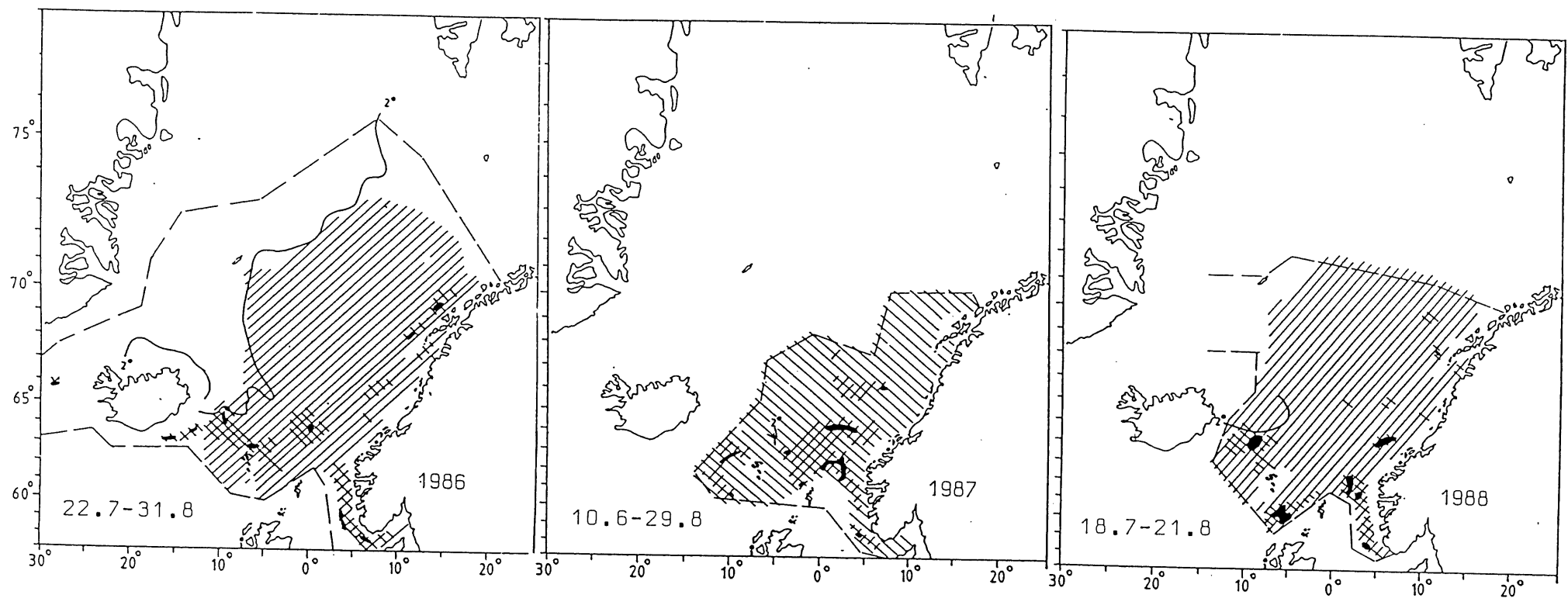
Fig. 6C. Distribution and densities of blue whiting with 2° C - isoline at 200 m depth, during summer 1984-1988. Symbols as in Fig. 6A.
