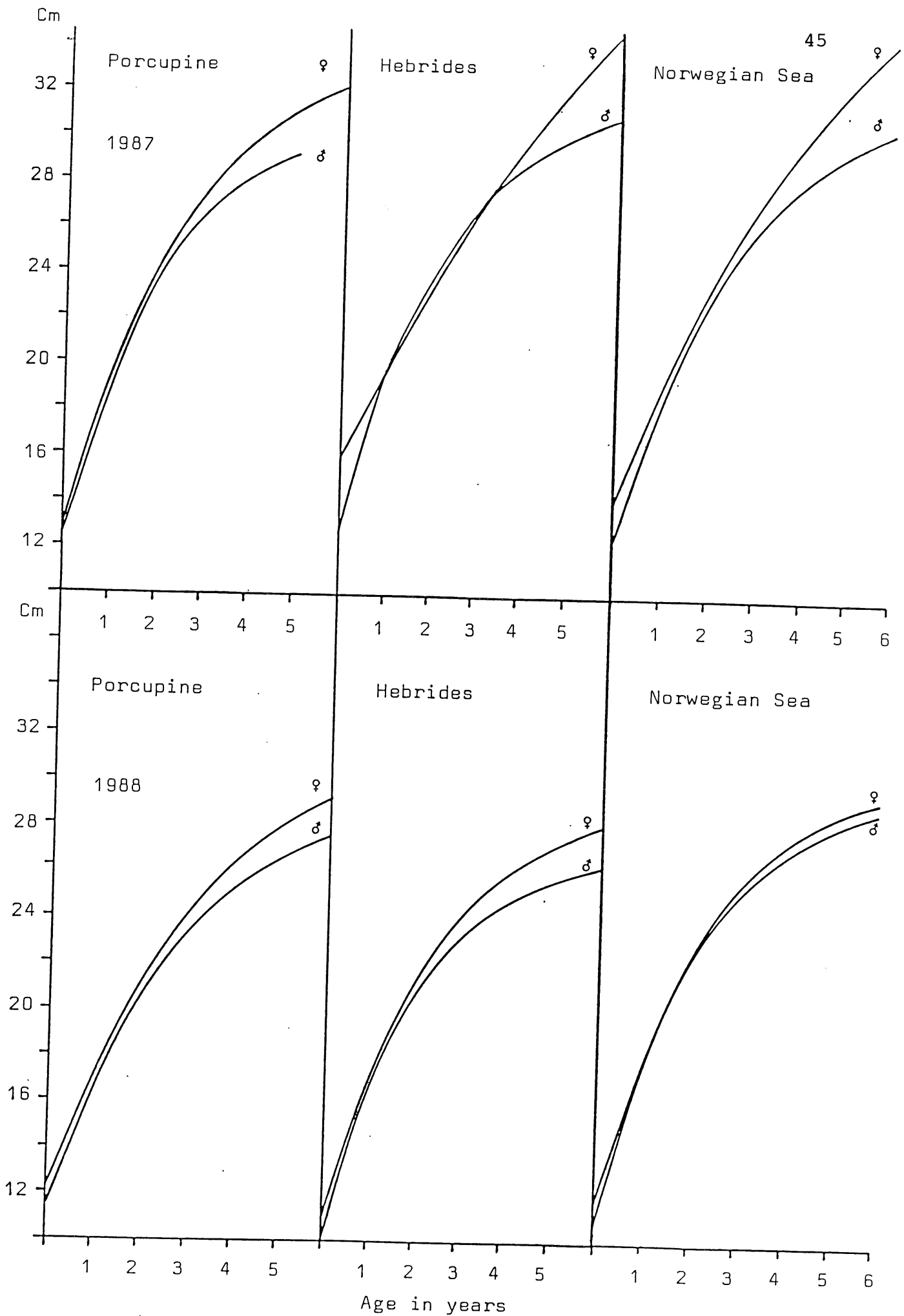
Fig. 16. von Bertalanffy's growth curves based on backcalculated lengths of blue whiting for the six first years of life, males and females, as appearing in three different areas in 1987, upper half and in 1988, lower half.
