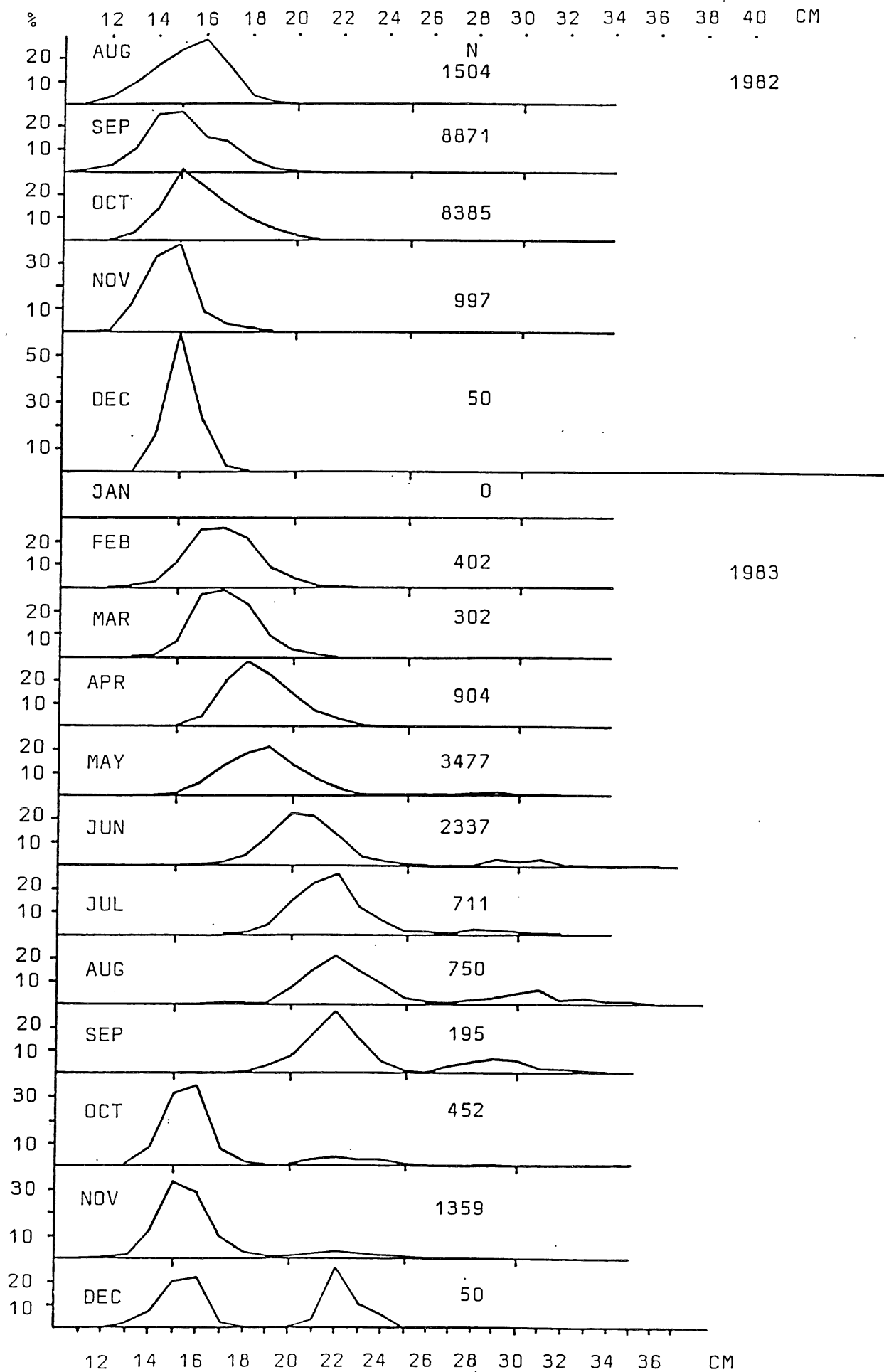
Fig. 13A. Length distribution (n%) by month of blue whiting in samples from the mixed industrial fishery in the North Sea, 1982 and 1983.
