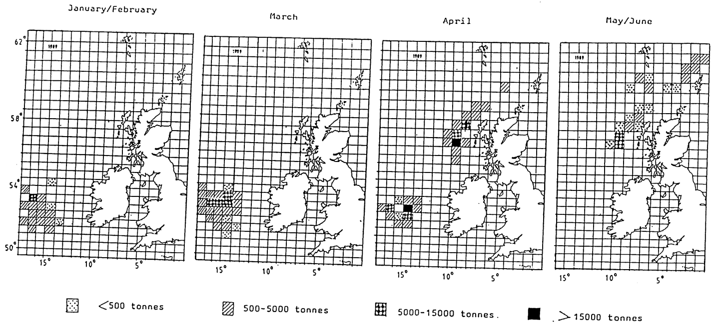
Fig. 3D. Progress of the Norwegian Blue Whiting fishery in the spawning area 1989.
