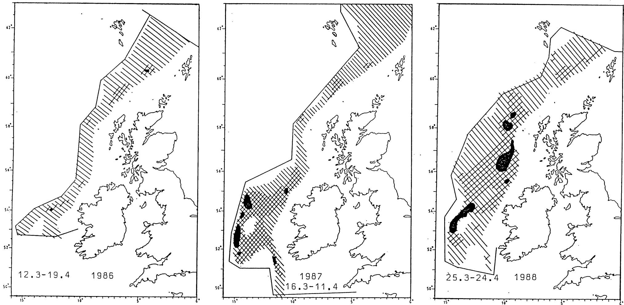
Fig. 4C. Distribution and densities of blue whiting during spring 1986-1988. Symbols as in Fig. 4A.
