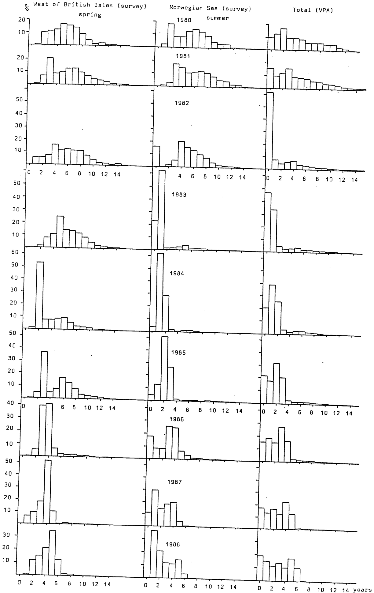
Fig. 7A. Age composition (N%) of blue whiting in the period 1980 - 1988, in the spawning stock west of the British Isles during spring, in the stock recorded in the Norwegian Sea during summer and in the total stock as calculated by VPA.
