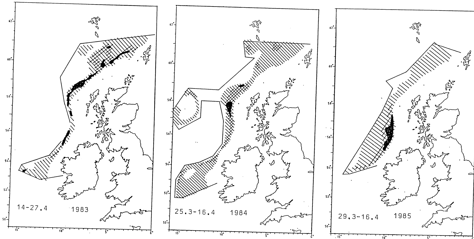
Fig: 4B. Distribution and densities of blue whiting during spring 1983-1985. Symbols as in Fig.4A.
