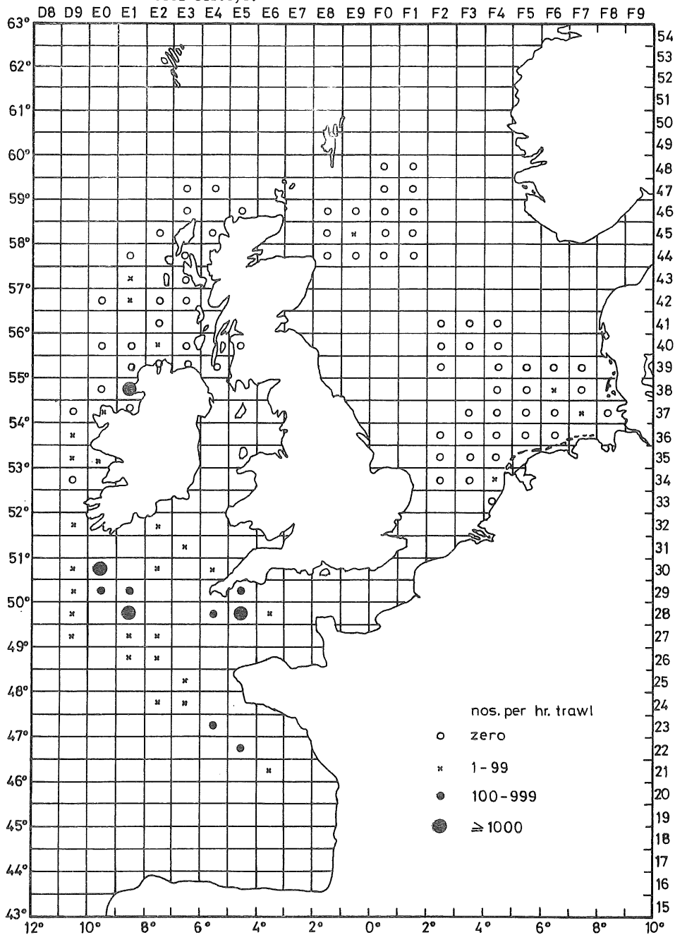
Figure 4.4 Distribution and abundance of the 1985 year class in the winter of 1985-86 from Dutch, English, Irish and Scottish research vessel surveys. 61
