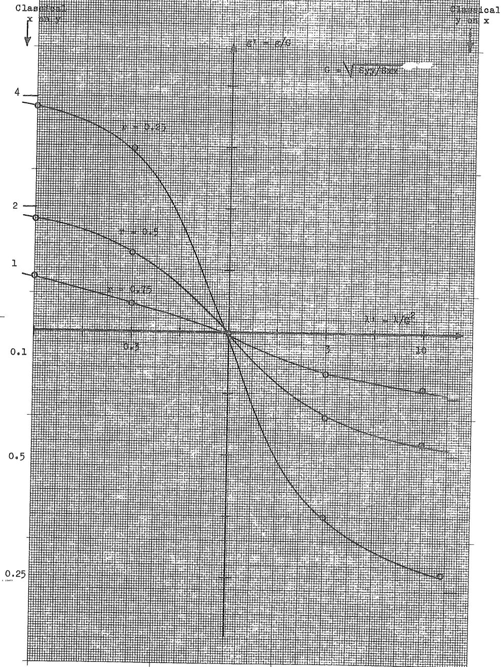
Figure 3.1 Regression analysis. (For a detailed explanation, see p.16.)
