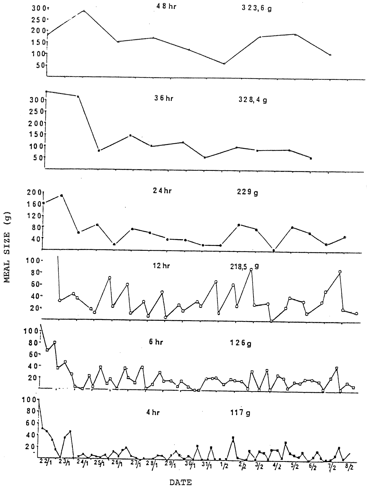
Fig. 1. Continuous feeding experiment with cod of various size groups, at time intervals from 4 to 48 hours. (experiment nr.1).
