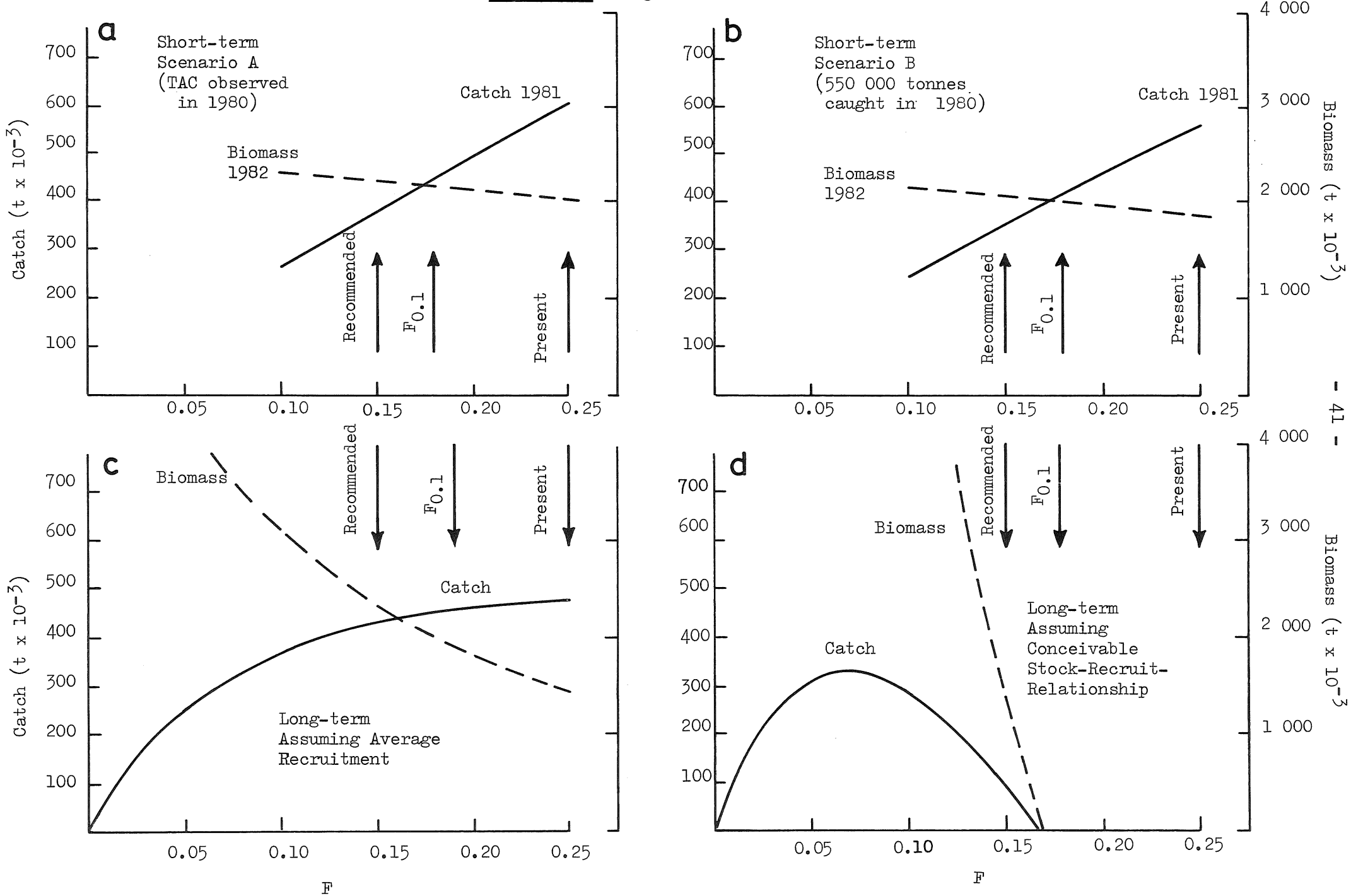
Figure 7.1 Prognoses for Western Macrarel Stock: Catch and Biomass
