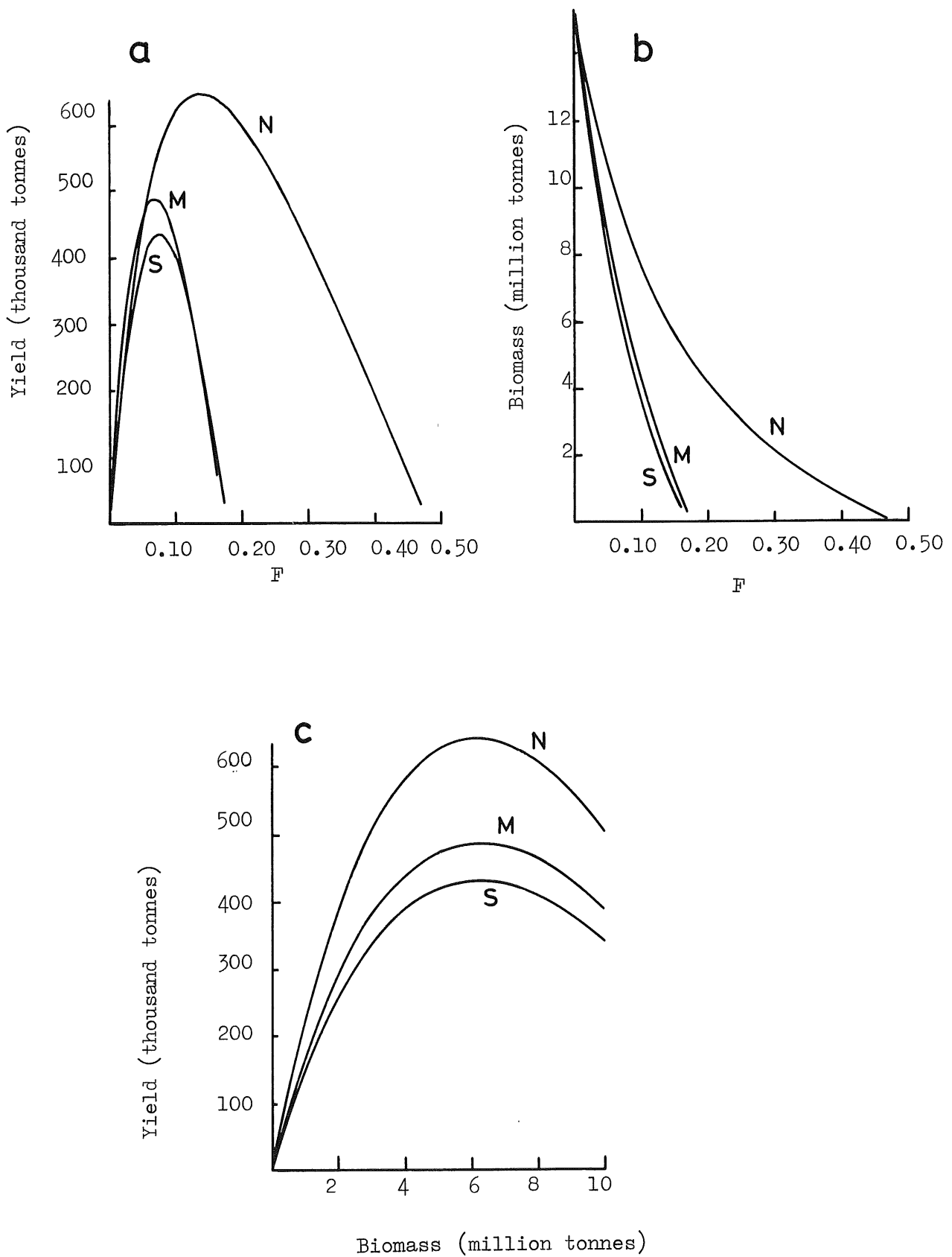
Figure 8.5. Total yield and total biomass for the present mixed (M) a northern fishery (N) limited to VIa and VIIa-c and a southern fishery (S) limited to VIIId-k and VIII.
