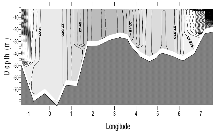
Figure 10-5: Vertical section of water density (sigma-t) along longitude 55.15 N.
