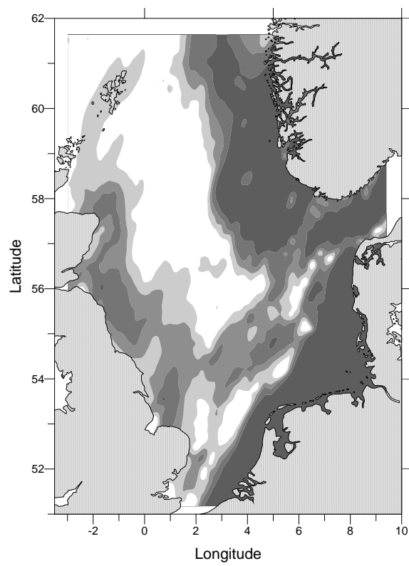
Figure 10-4: Rate of change in water density (relative).
