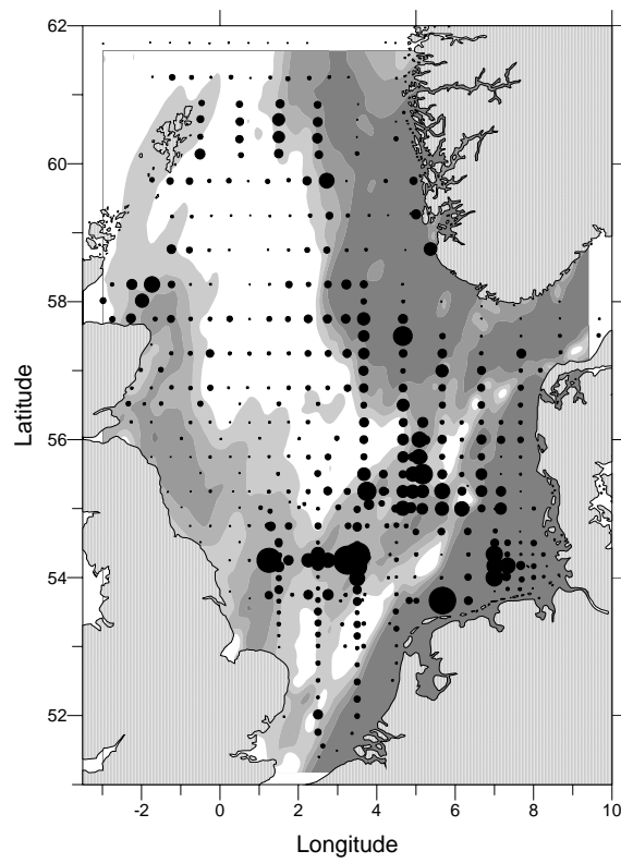
Figure 10-6: Relative abundance of cod eggs against rate of change in sigma-t (area of circles indicates \text{no m}^{-2} ).
