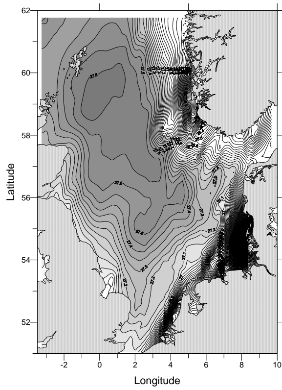
Figure 10-3: Surface density ( \sigma_t ).
