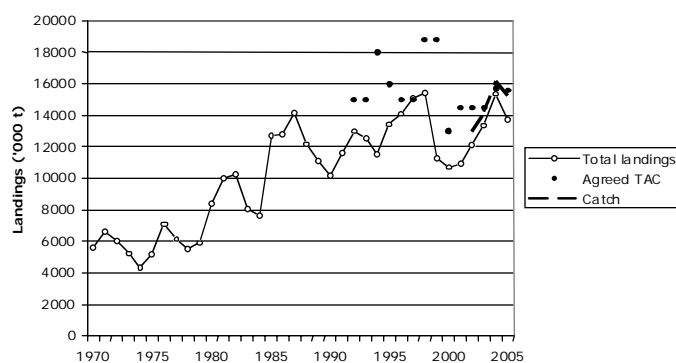
Fig. 5.1. Agreed TAC, total landings by all fleets, and total catch including estimated Swedish high-grading for 2002-2005.
