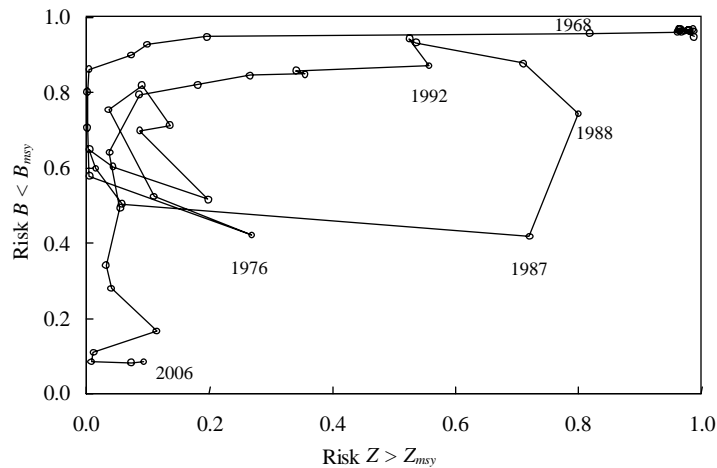
Fig. 3.9. Shrimp in Subareas 0 and 1: risk of annual biomass being below B_{msy} and of mortality caused by fishing and cod predation being above Z_{msy} 1956-2006.
