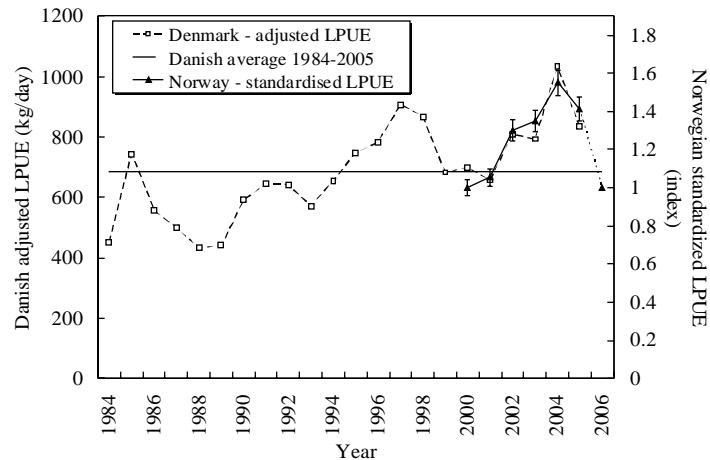
Fig. 5.2. Long-term adjusted LPUE for Denmark (whole period) and standardized LPUE for Norway (2000-2006) with SE.
