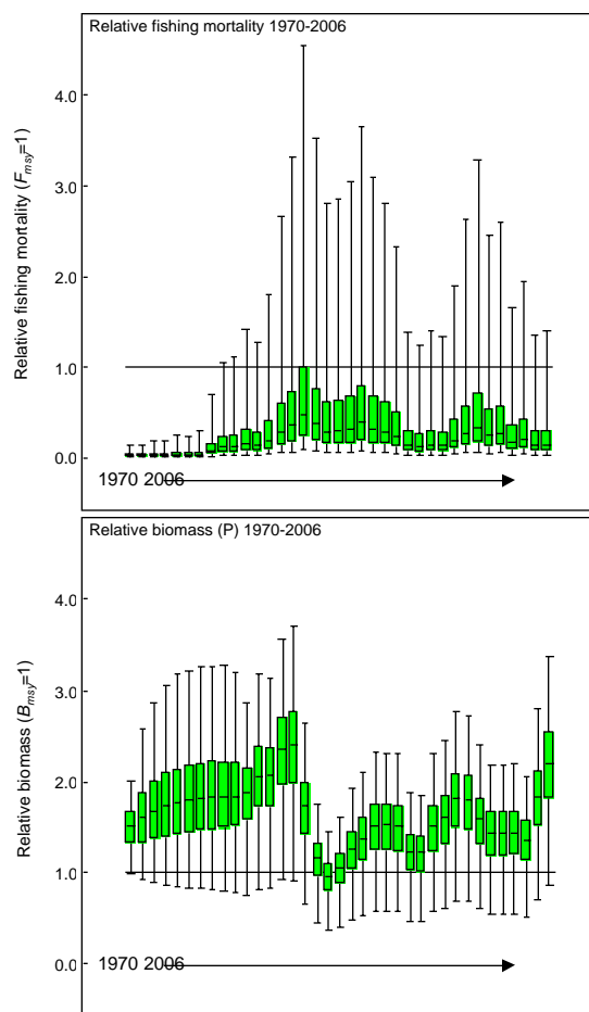
Fig. 6.5. Shrimp in the Barents Sea: estimated relative biomass ( B_t/B_{msy} ) and fishing mortality ( F_t/F_{msy} ) 1970-2006. Boxes represent inter-quartile ranges and the solid black line at the (approximate) centre of each box is the median; the arms of each box extend to cover the central 95 per cent of the distribution.
