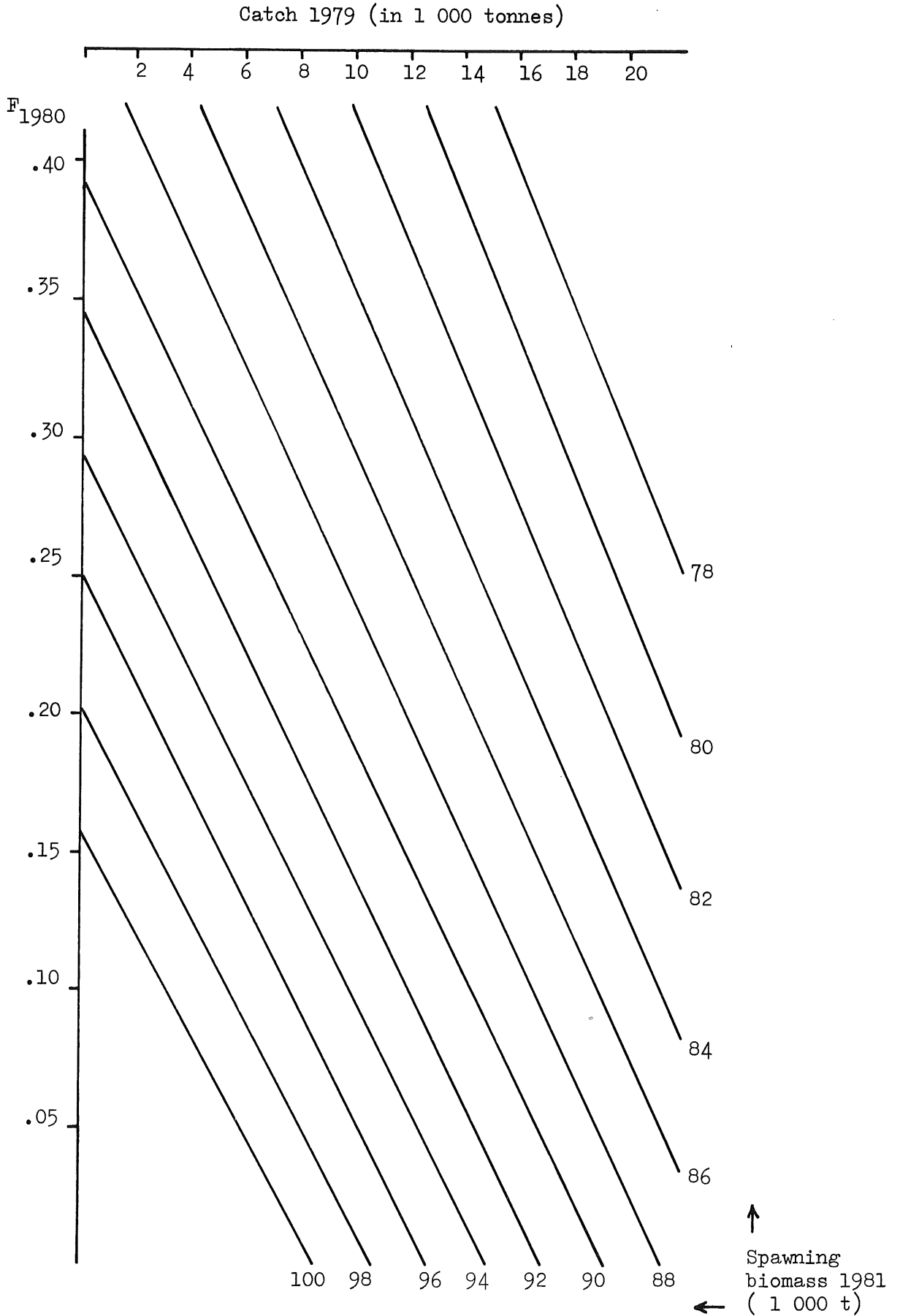
Fig. 12 Sebastes mentella Sub-areas V and XIV. Spawning stock biomass in 1981 at different levels of F in 1980 and different catch levels in 1979
