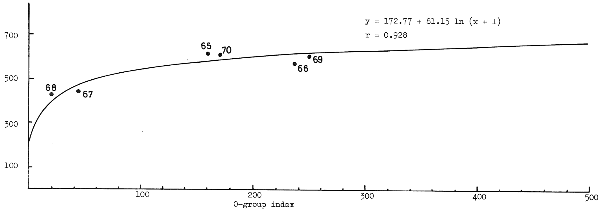
Figure 3. Sebastes mentella in Division IIa and IIb. Relation of year class strength at age 6 (from VPA) to corresponding O-group survey abundance indices.
