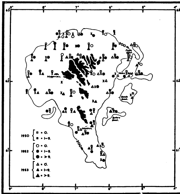
Figure 6. Distribution of haddock larvae at Faroe in June 1950-53. The symbols represent the catches of a 2-metre ring net hauled vertically from bottom to surface.
