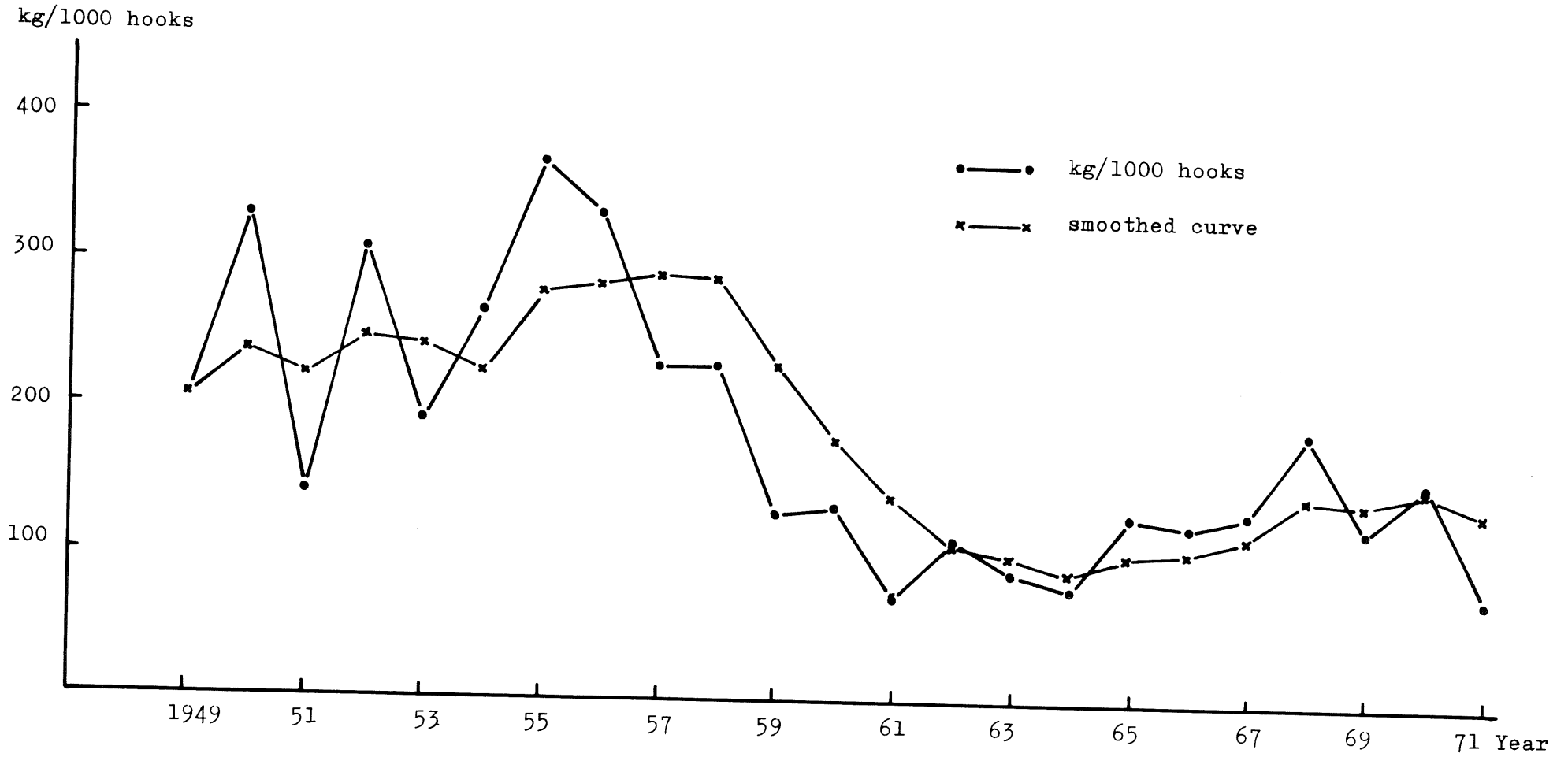
Figure 3. Cod. Faroese long-line catch per unit effort. (Source: K Hoydal, unpubl.)
