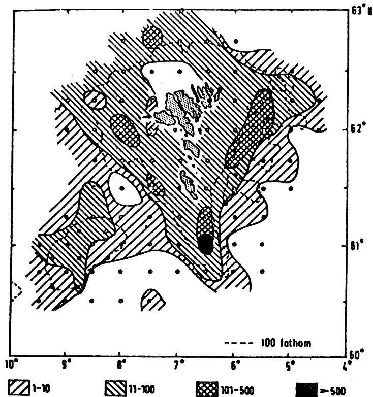
Figure 7. Distribution of 0-group haddock (numbers per half-hour tow). ("Cirolana", 1975).
