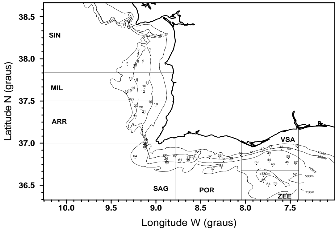
Figure 1. Stratification of SW and S Portugal used in Portuguese Crustacean Trawl survey in the period 1997–2004.
