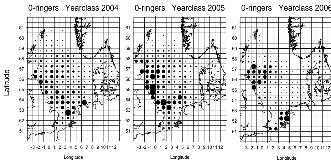
Figure 4.1.2.2. North Sea herring. Distribution of 0-ringer herring, year classes 2004–2006. Abundance estimates of 0-ringers within each statistical rectangle are based on MIK catches during IBTS in February 2005–2007. Areas of filled circles illustrate densities in no m -2 , the area of a circle extending to the border of a rectangle represents 1 m 2 .
