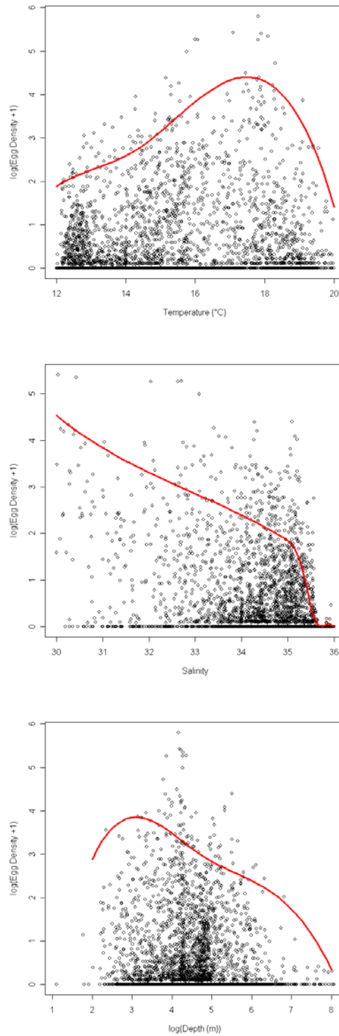
Figure 2.3.1. Modelled 95% quantiles of anchovy egg abundance as a function of surface temperature, surface salinity and log(Bottom Depth). The models are fitted to data collected from southern Spain to the West of Brittany for the period 2000–2005. Egg data were collected with the Continuous Underway Fish Egg Sampler (CUFES) by IPIMAR, IEO and Ifremer institutes.
