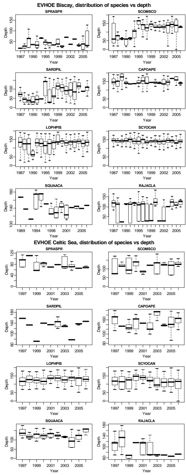
Figure 4.9. continued. Depth distribution by species (from top left: Sprattus sprattus , Scomber scombrus , Sardina pilchardus , Capros aper , Lophius piscatorius , Seyllorhinus canicula , Squalus acanthias and Raja clavata ) from the western IBTS survey in the Bay of Biscay and Celtic Sea. For this analysis each caught individual was assigned the depth of the given haul.
