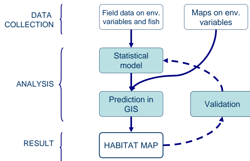
Figure 4.5. Principal steps in mapping of essential fish habitats, as applied within the Interreg IIB project Balance.
