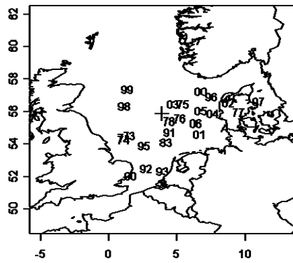
gravity centres - ENGRAULIS_ENCRASICOLUS - Q1 gravity centres - ENGRAULIS_ENCRASICOLUS - Q3
