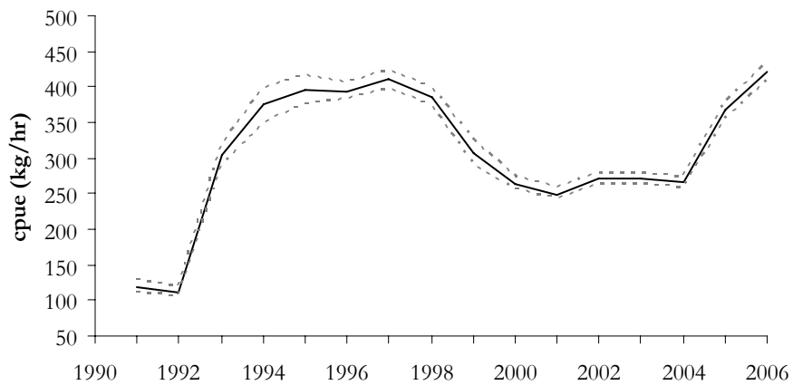
Figure 6.11. Standardised CPUE from trawler fleets in XIVb. 95% CI indicated
