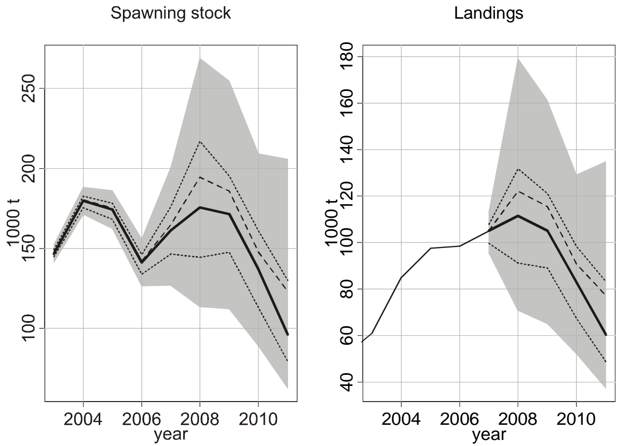
Figure 3.4.7.10 Haddock in division Va. Cumulative probability profiles of landings, and SSB according to the SPALY run based on the March survey. F=0.47 and 15%CV in assessment.
