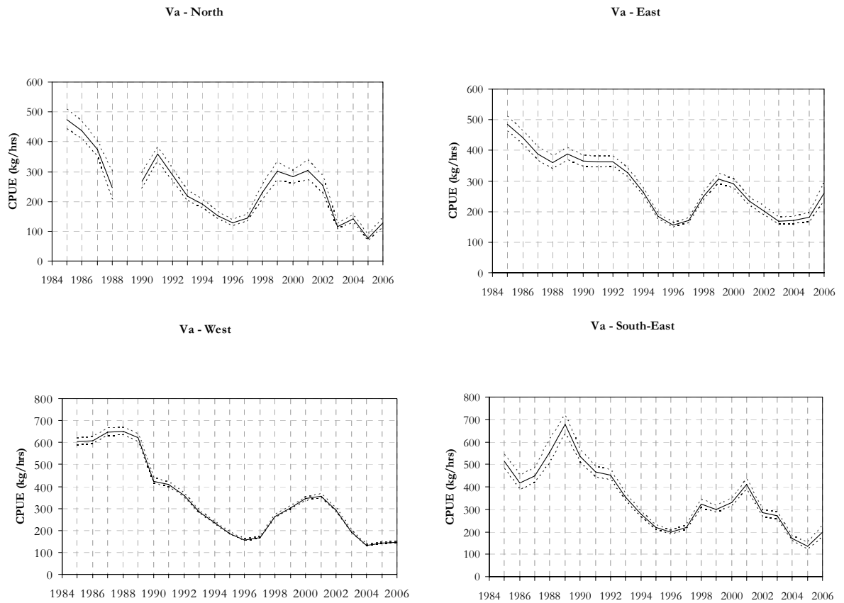
Figure 6.9. Standardised CPUE from the Faroese trawler fleet. 95% CI indicated
