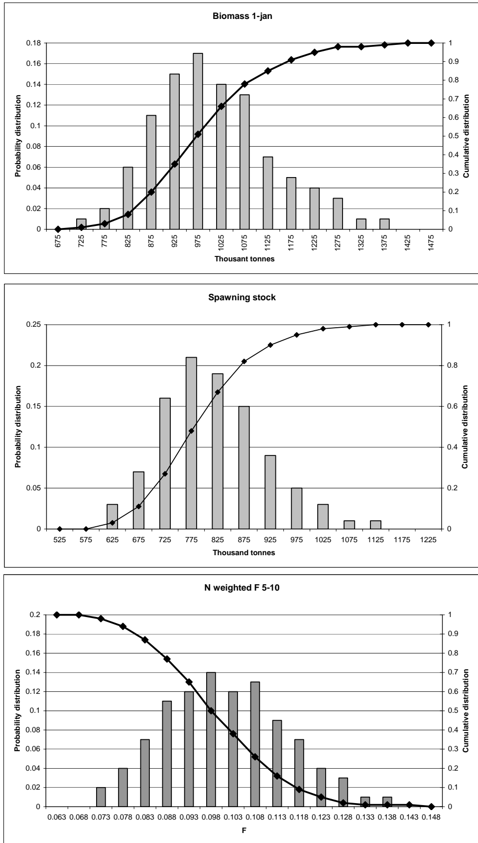
Figure 3.5.5.2.6. Probabilities plot for a bootstrap run with 1000 replicates of the final Adapt run for Icelandic summer-spawning herring.
