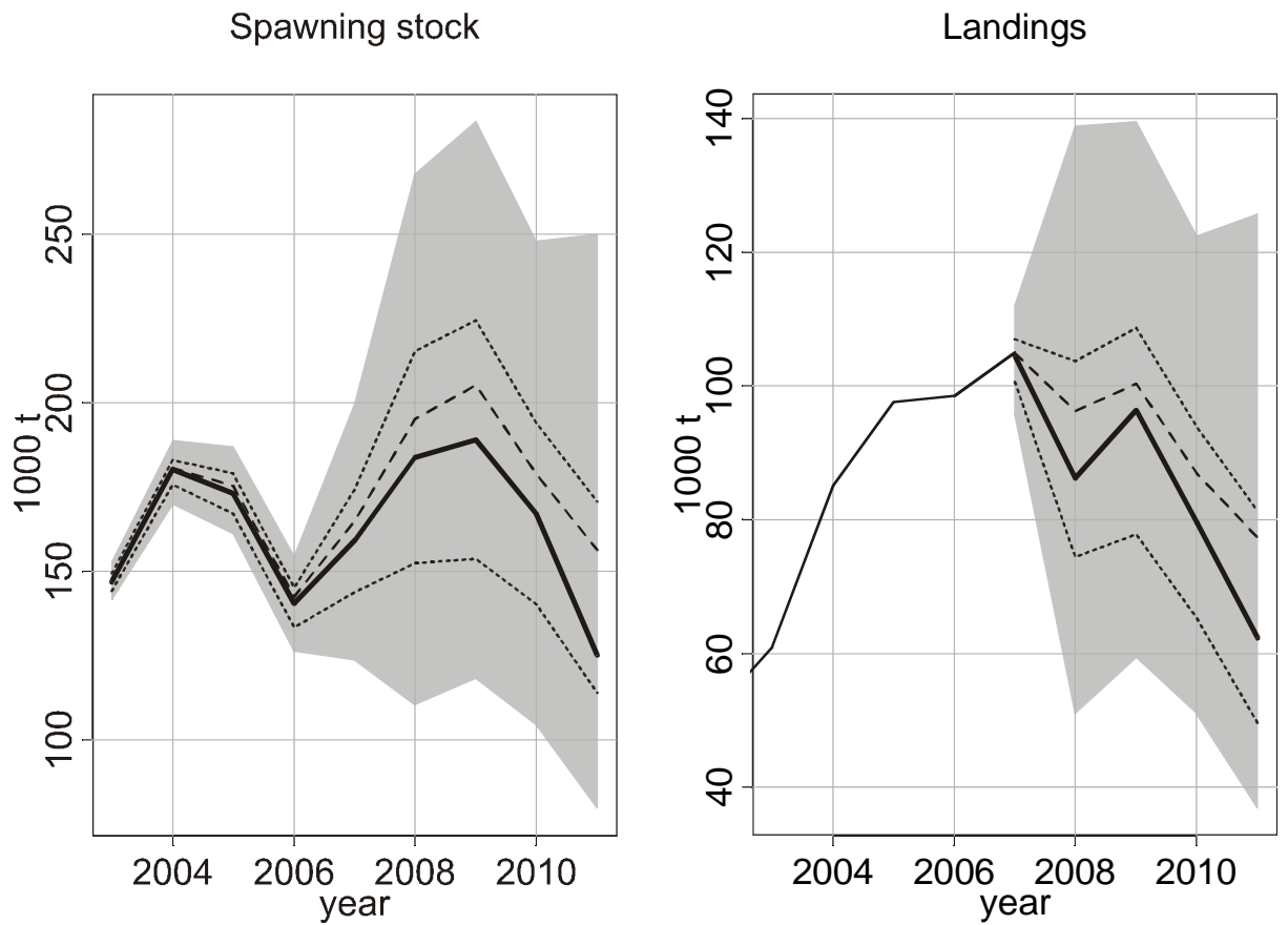
Figure 3.4.7.9 Haddock in division Va. Cumulative probability profiles of landings, and SSB according to the SPALY run based on the March survey. F=0.35 and 15%CV in assessment.
