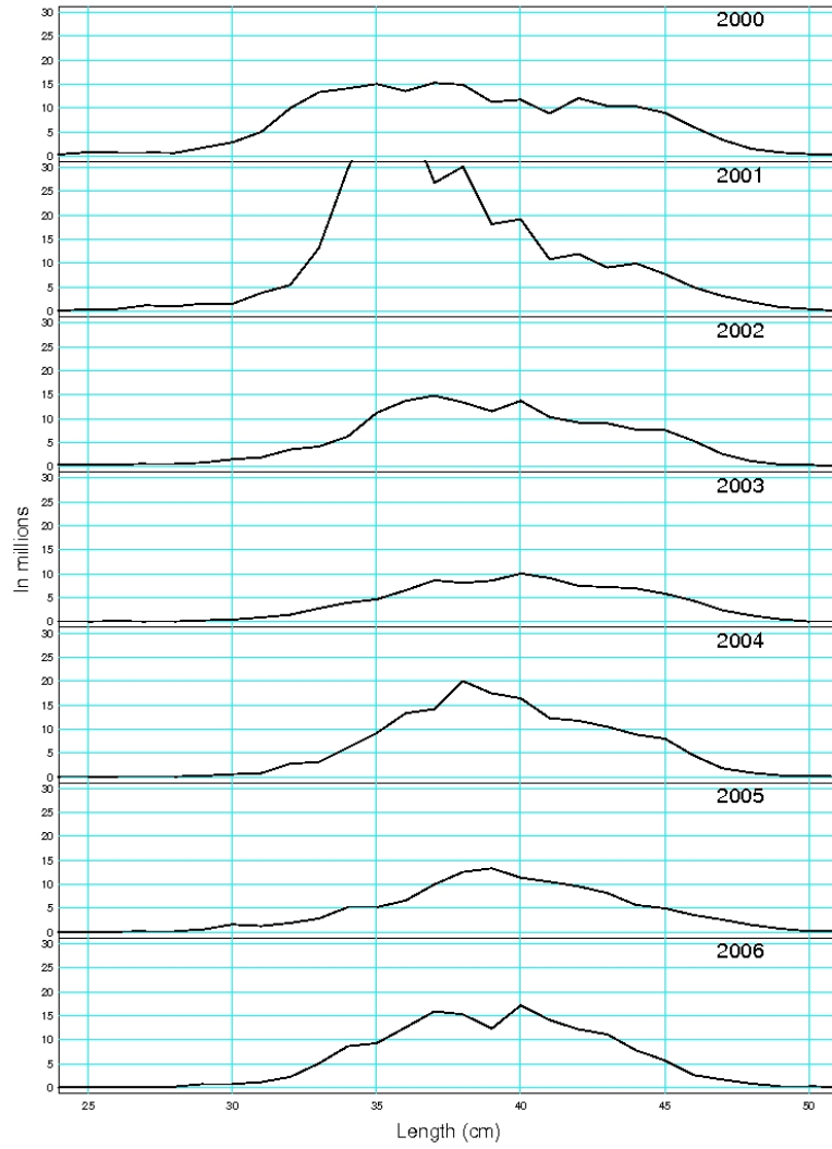
Figure 9.2.6 Length distribution of demersal S. mentella in the bottom trawl surveys in October 2000-2006 in ICES Division Va.
