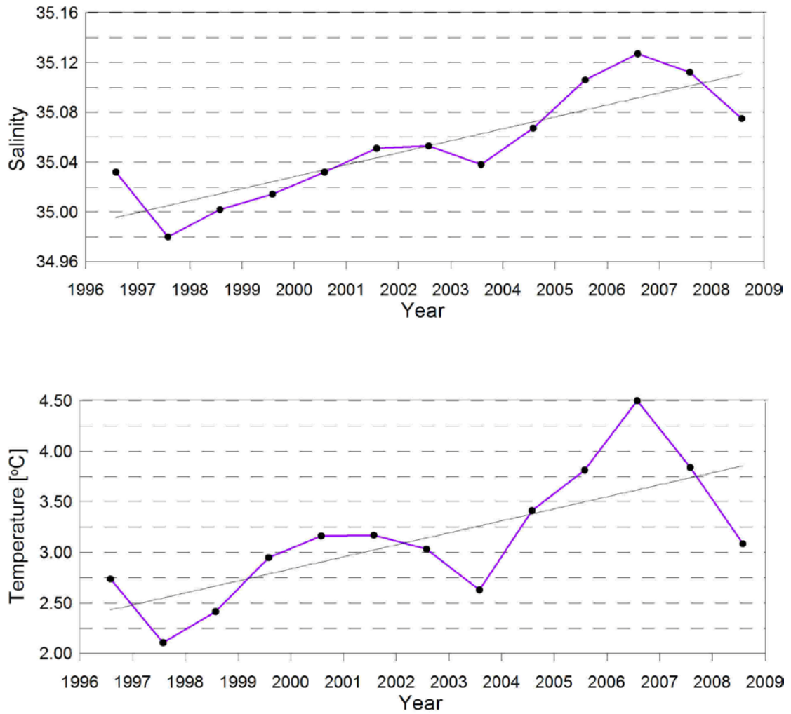
Figure 2. Mean salinity (upper panel) and mean temperature in summer (July) at section 'N' (76°30' N) at 200 m, between 009°– 012° E. Linear trends are marked.
