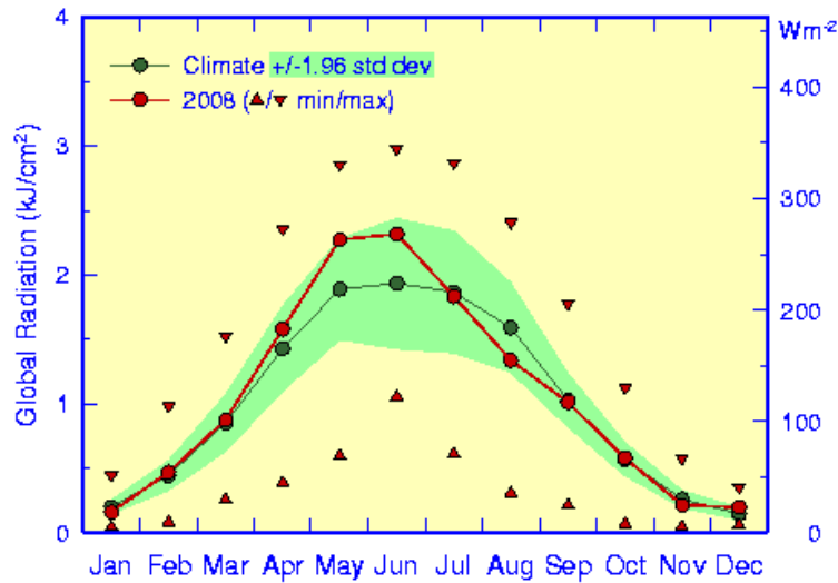
Figure 1. Monthly averaged global radiation at Norderney in 2008 [kJ/cm 2 ]. Data kindly provided by the German Weather Service (DWD).
