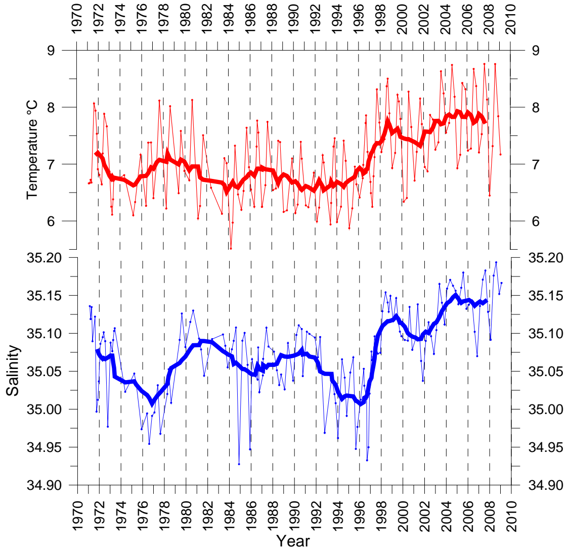
Figure 5. Mean temperature 0–200 m at the shelf brake west of Iceland, 1971–2009. Combined data from stations RE8 (1971–1984) and FX9 (1984–2009), 20 nm apart. Thick line is approx. 3 years running mean.
