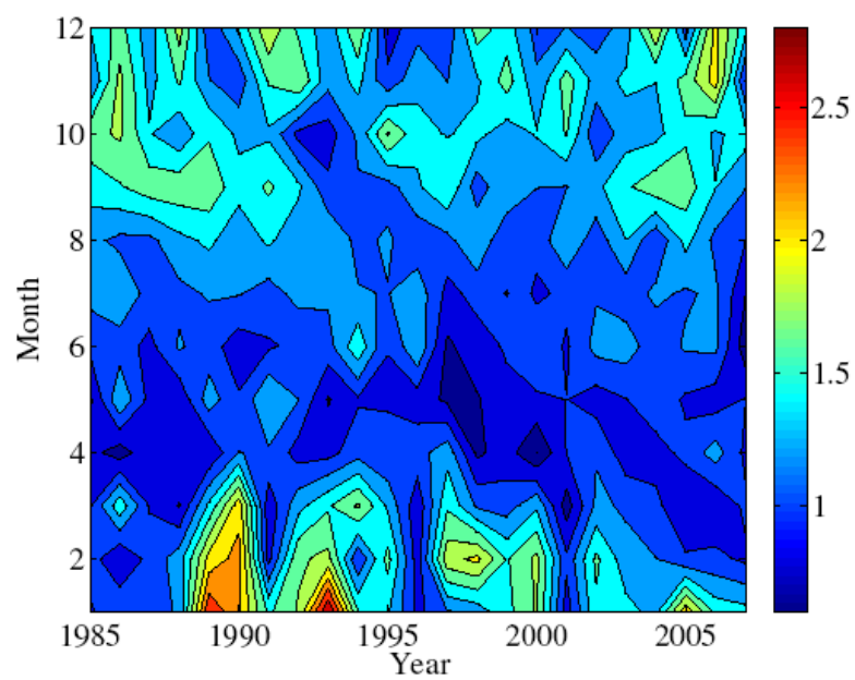
Figure 9. Time-series (1985–2007) of modelled monthly mean volume transport of Atlantic water into the northern and central North Sea southward between the Orkney Islands and Utsira Norway. 1 \text{ Sv} = 10^6 \text{ m}^3 \text{ s}^{-1} . (ANON. 2007)
