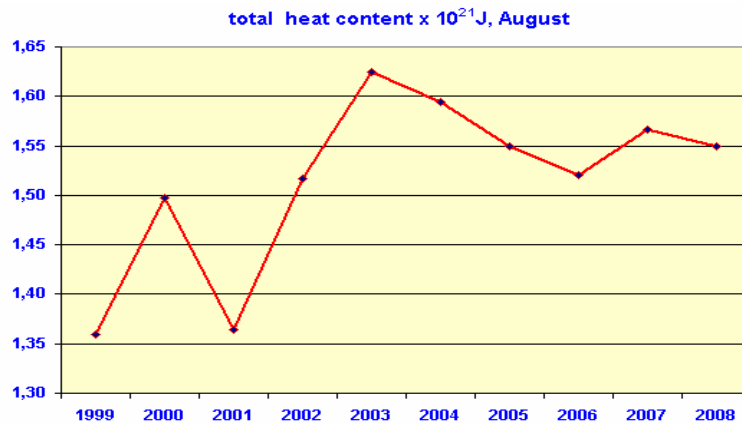
Figure 10. Total heat content in J \times 10^{12} , 1999–2008.
