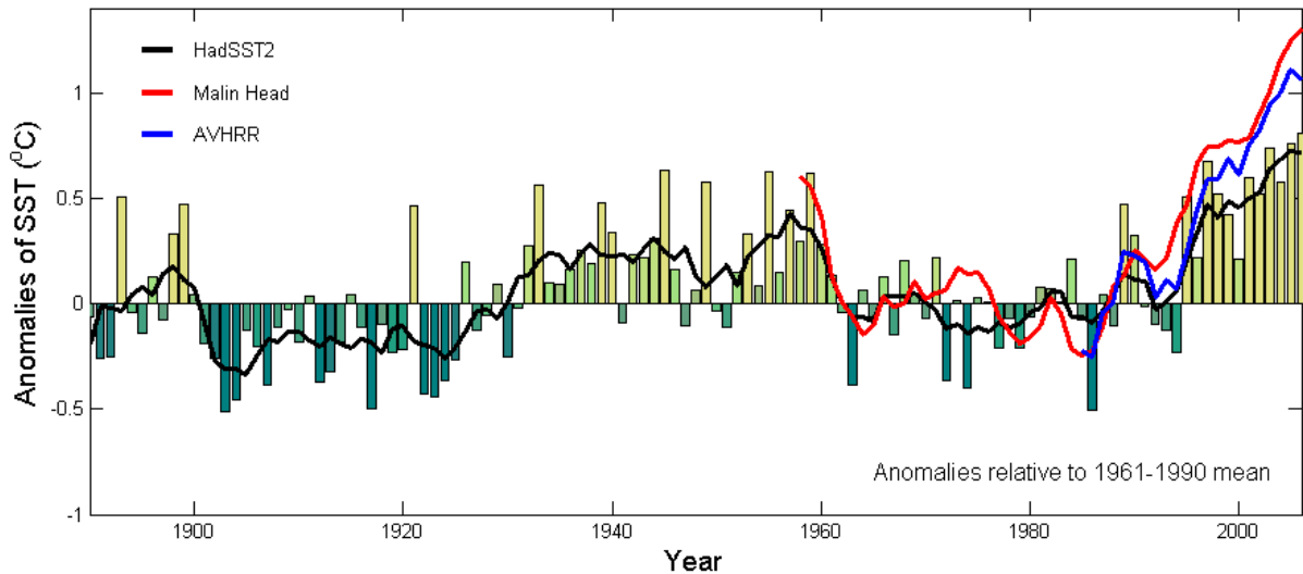
Figure 2. Sea surface temperature from Malin Head (Ireland) 1960–2005 overlaid on the longer term HADSST data set and satellite derived AVHRR SST measurements (from Cannaby and Hurrevoglou (2009)).
