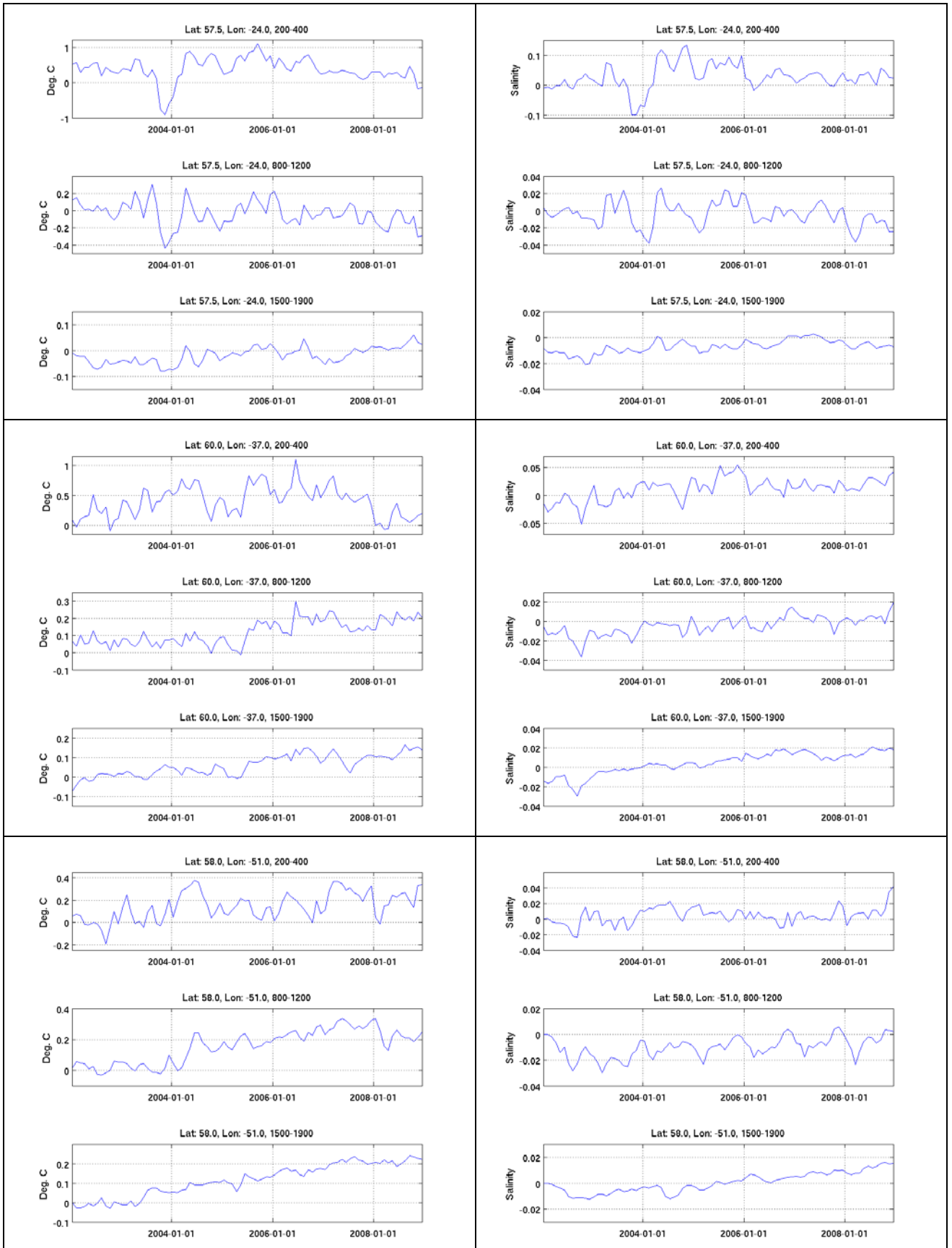
Figure 10. Time-series of temperature (left) and salinity (right) averaged over layers. 200–400m (top), 800–1200 (middle) and 1500–1900 (bottom). Points 6, 7, 8.
