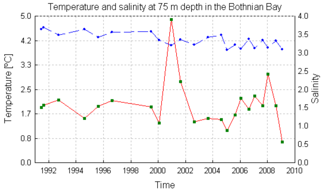
Figure 3. The temperature and salinity at 75m depth in the Bothnian Bay.
