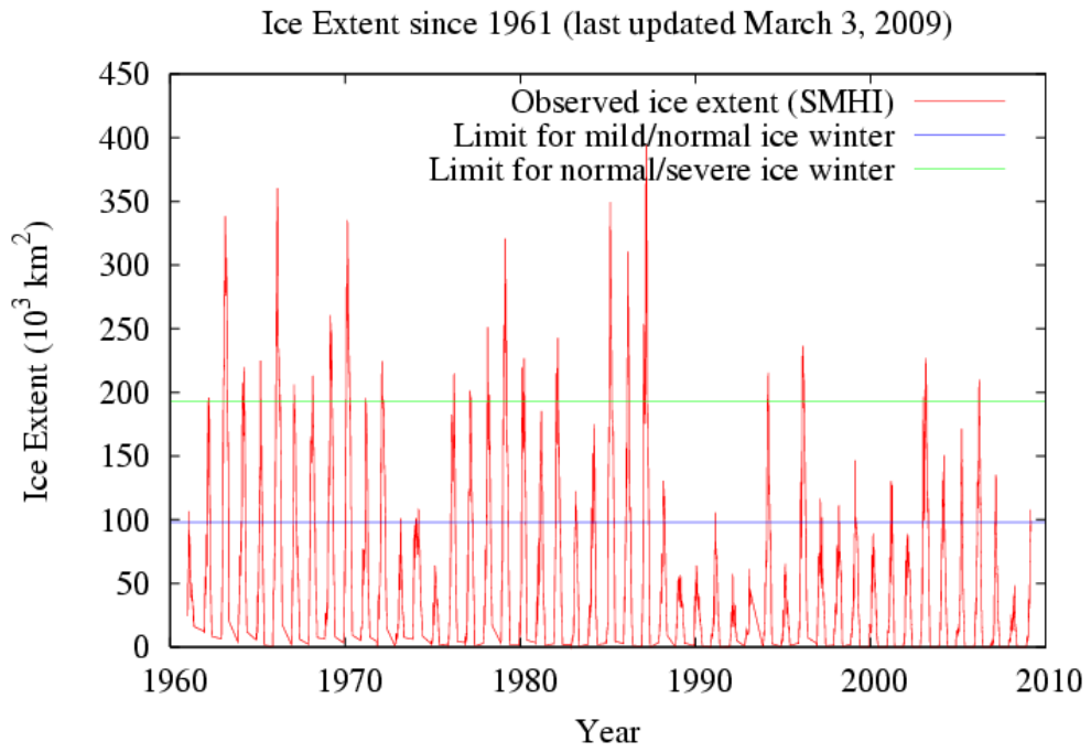
Figure 8. The ice extent in the Baltic starting from 1961. The last value is from 03 March 2009. Graph constructed by Lars Axell (SMHI).
