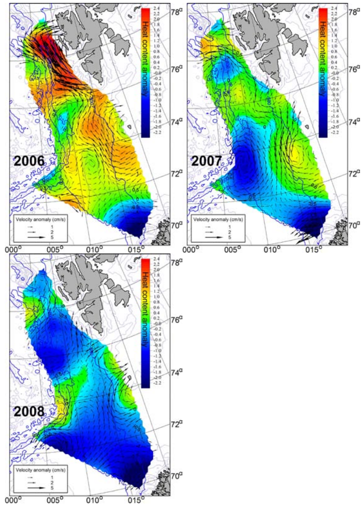
Figure 7. June/July 2000–2008. AW layer heat content anomaly ( GJ.m^2 ) – colour scale and baroclinic currents at 100 dbar anomaly. Reference level 1000 m.
