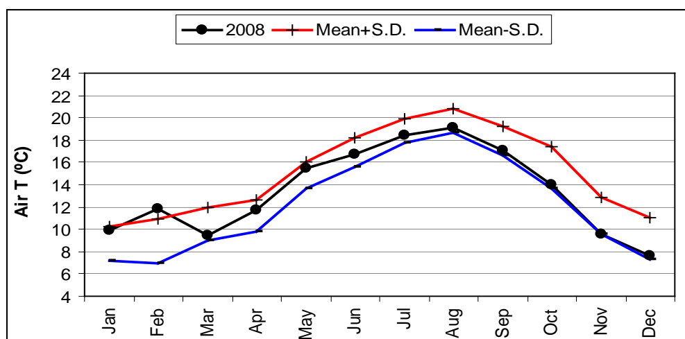
Figure 3b. Monthly mean air temperature ( ^{\circ}\text{C} ) in San Sebastián ( 43^{\circ}18.5'\text{N} , 02^{\circ}2.37'\text{W} ) in 2008 compared with the mean \pm standard deviation for the period 1986–2008. Courtesy of the 'Agencia Estatal de Meteorología'.
