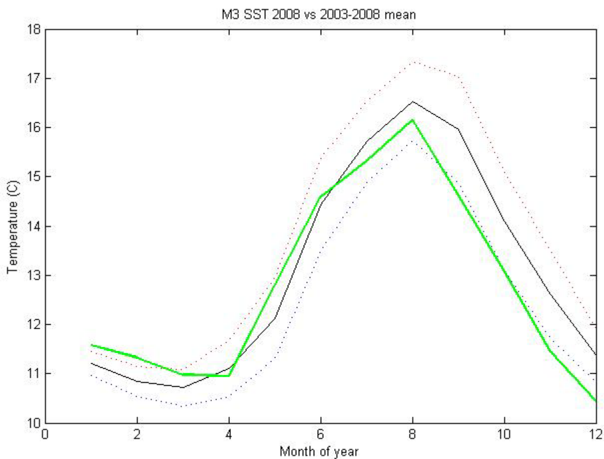
Figure 4. SST at the M3 weather buoy (green line) in 2008 compared with the time-series mean (black line).
