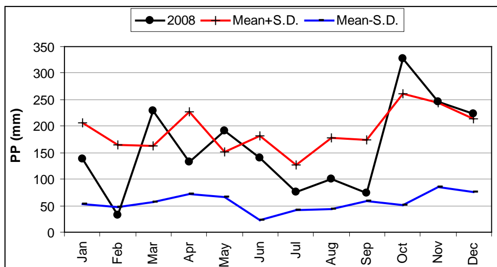
Figure 5c. Monthly precipitation (mm) in San Sebastián (43°18.5'N 02°2.37'W) in 2008 compared with the mean ± standard deviation for the period 1986-2007. Data Courtesy of the ‘Agencia Estatal de Meteorología’.
