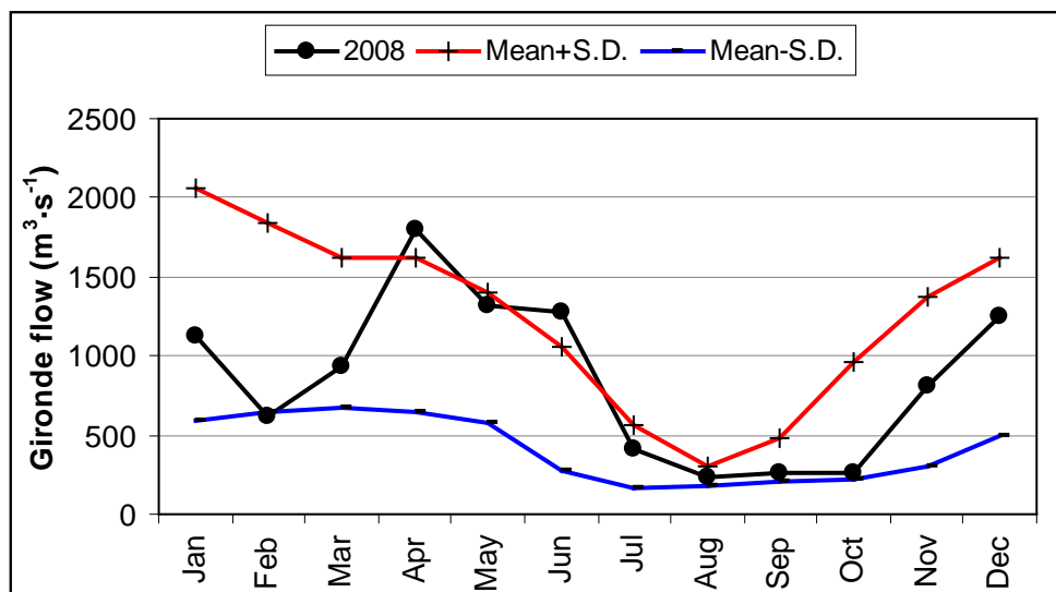
Figure 8. Monthly mean flow ( \text{m}^3 \text{ s}^{-1} ) of the Gironde River in 2008 compared with the mean \pm standard deviation for the period 1986–2008. Data Courtesy of the 'Bordeaux Harbour Authority'.
