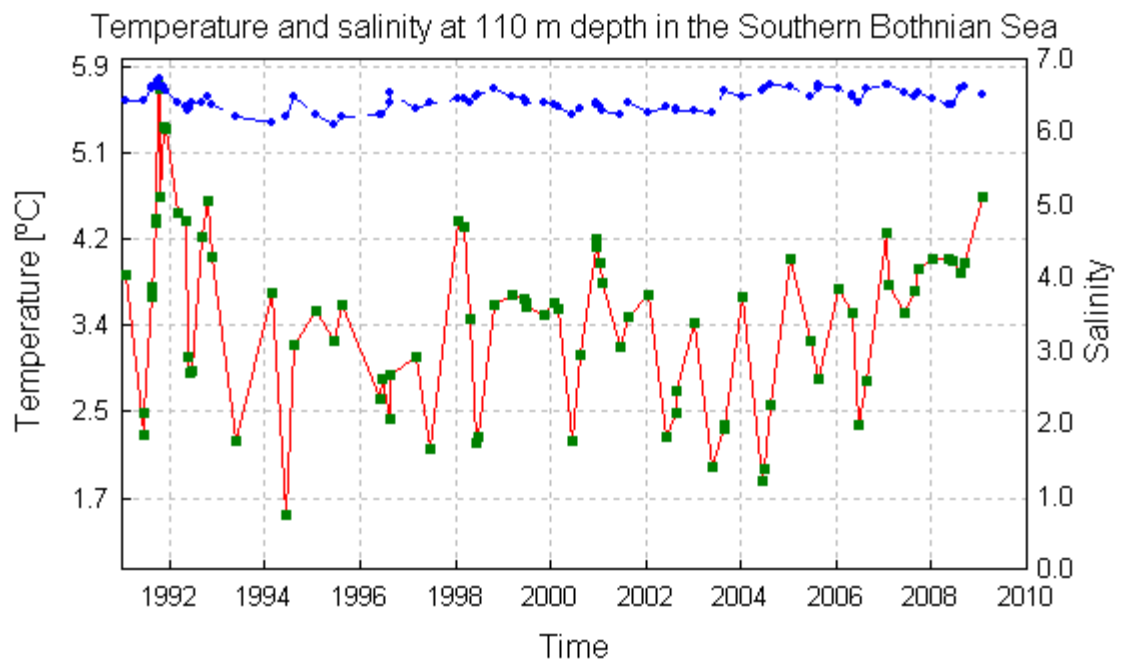
Figure 5. The temperature and salinity at 110m depth in the southern Bothnian Sea.
