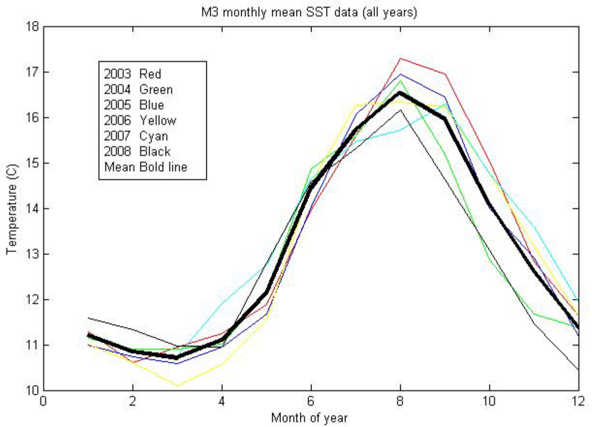
Figure 3. SST at the M3 weather buoy since its deployment in 2002 compared with the time-series mean (black line).
