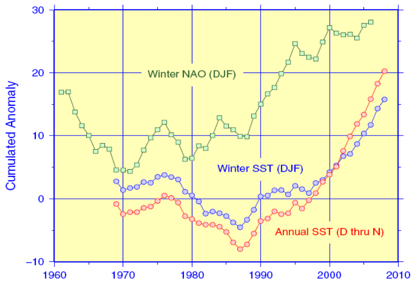
Figure 6. Time-series of cumulated standardised anomalies for winter (DJF) and annual (December through November) North Sea SST and of cumulated winter NAO index (Koslowski and Löwe, 1994).
