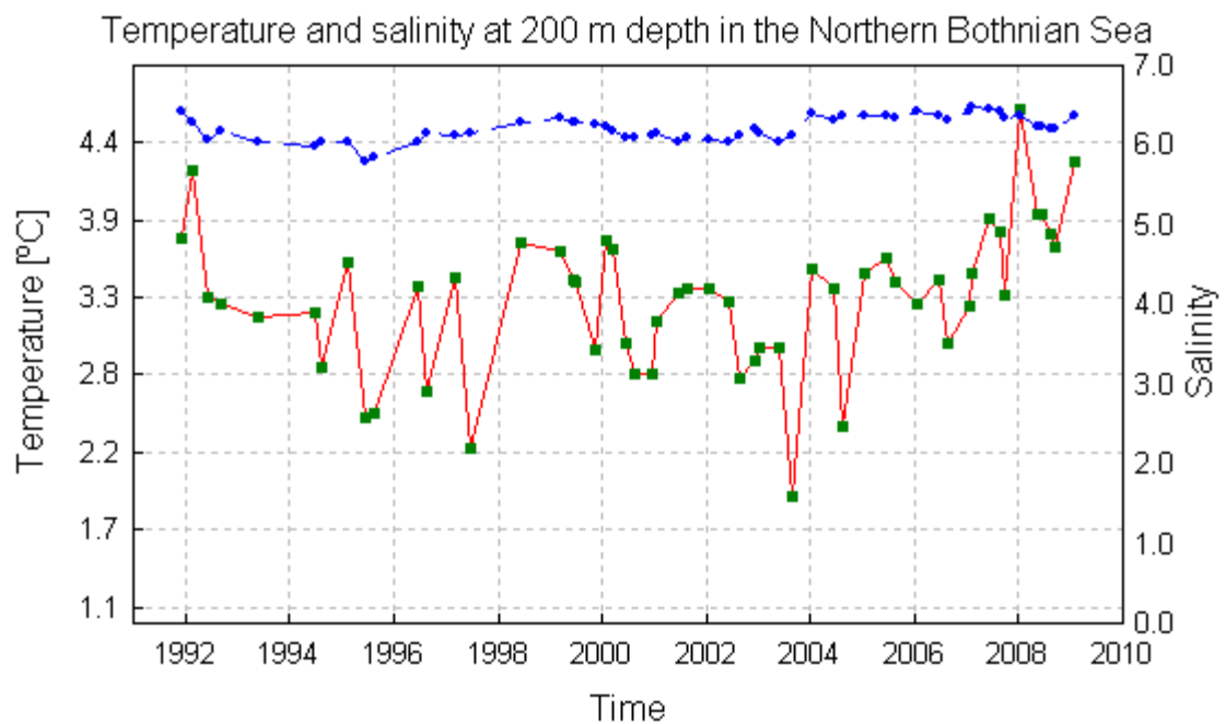
Figure 4. The temperature and salinity at 200m depth in the northern Bothnian Sea.
