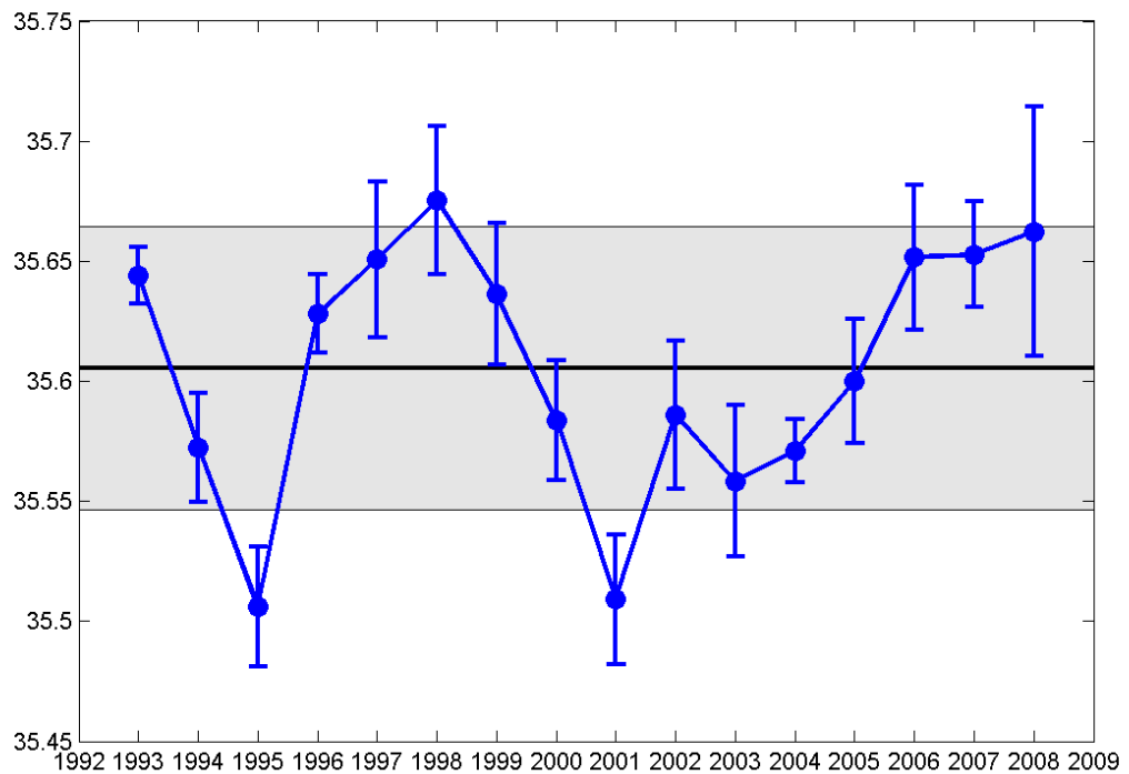
Figure 17. Annual average salinity (5-300m) at Santander station 6 (shelf-break).
