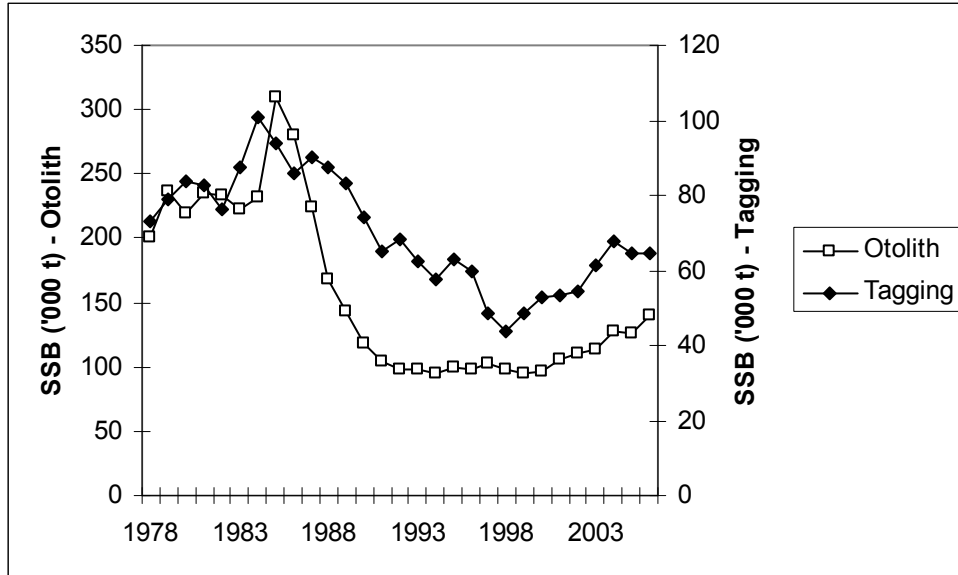
Figure 3.2.1.1. Comparison of trends in SSB from two assessments based on different growth rate.
