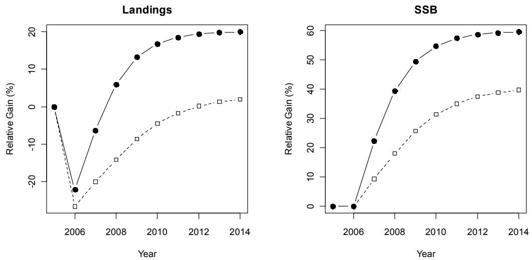
Figure 3.2.1.3. Short term projections under two hypothesis on growth rates. (otolith: white square and tagging : black circles).
