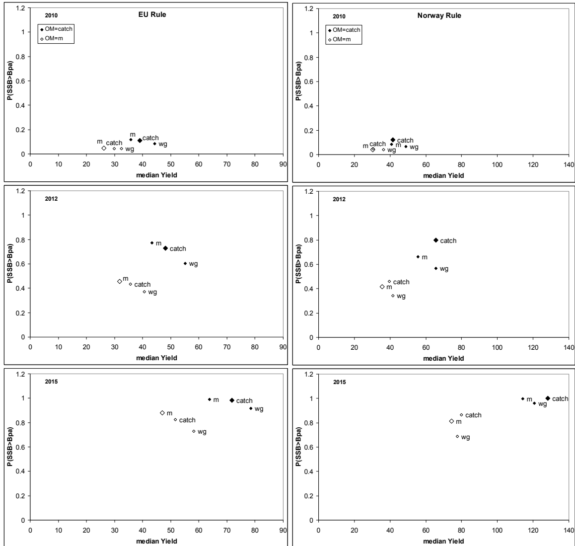
Figure 3.2.3.1. Comparing the performance of two cod recovery plans (EU proposal on the left, and Norwegian proposal on the right) in terms of summary statistics “P(SSB>Bpa)” (probability of SSB exceeding Bpa; vertical axis) and “median Yield” (horizontal axis) for the years 2010, 2012 and 2015, based on results from ICES-AGCREMP (2008). Solid diamonds indicate the operating model assumed additional mortality was due to catch misreporting (“catch”), and open diamonds due to additional natural mortality (“m”). The recovery plans either adjusted for catch misreporting (“catch”), or additional natural mortality (“m”), or made no adjustment (“wg”). Larger symbols indicate that the recovery plan makes the correct adjustment (i.e. consistent with the operating model).
