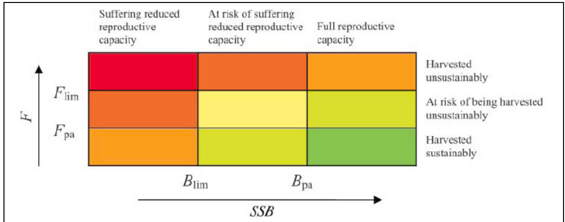
Figure 5.1.1. An overview of the status of fish stocks in relation to reference points, the basic idea being that, to have a high probability of avoiding a stock ending up in the red area (below B_{lim} and above F_{lim} ), decisions on management targets should be constrained within the green area (above B_{pa} and below F_{pa} ; from Hauge et al. , 2007).
