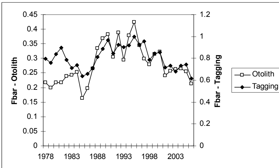
Figure 3.2.1.2. Comparison of trends in F from two assessments based on different growth rate.
