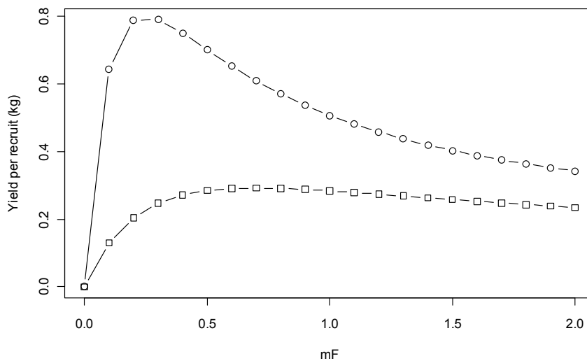
Figure 3.2.1.4. Yield per recruit less than two hypothesis on growth rates. (otolith: white square and tagging: white circles).
