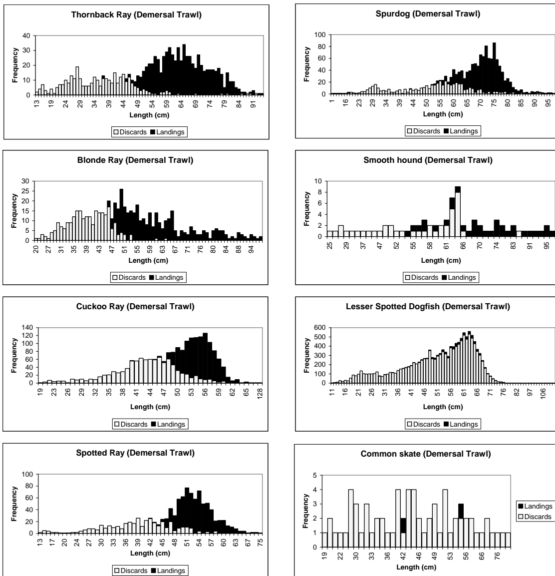
Figure 18.5. Demersal elasmobranchs in the Celtic Seas. Length distribution of elasmobranch species discarded and retained in Irish demersal trawl fisheries in the Celtic Seas. These data are aggregated across individual catch samples for all demersal gears and divisions combined. (Source: Irish Discard Observer Programme).
