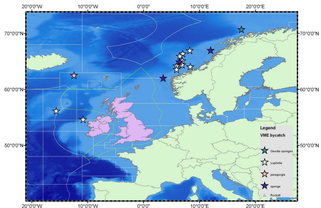
Figure 6. Confirmed cases where large quantities of VMEs have been observed in trawls by fishing and/or research vessels (see text and Table 1 for details).
