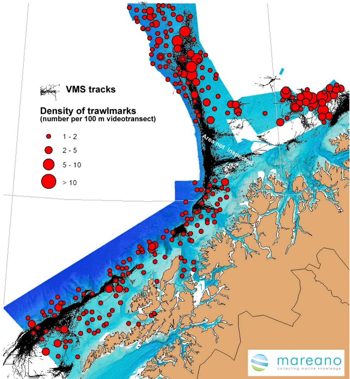
Figure 5. VMS tracks of Norwegian vessels in relation to observed trawl tarcks on the seabed (courtesy of Mareano project: www.mareano.no ).
