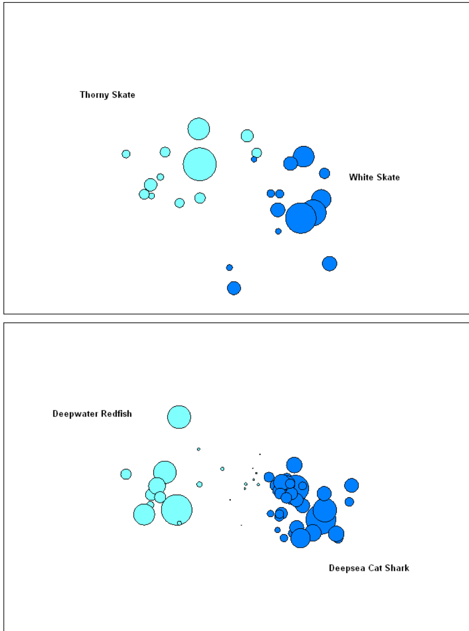
Figure 3. MDS configuration of the trawl catches (2001–2007) based on Bray–Curtis similarity matrix calculated from log 10 -transformed biomass data for each of 34 taxa. The proportional biomass of pairs of taxa which favour the sponge grounds (High Sponge Weight Class – dark blue) or areas with Low Sponge (light blue) are illustrated. Note that proportions are relative to each taxon.
