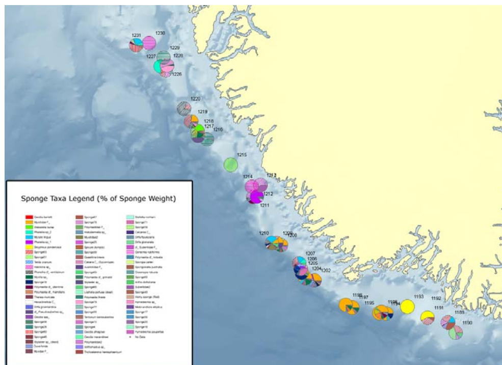
Figure 1. Relative proportions of sponge taxa by weight from research vessel survey tows along the west coast of Greenland. Numbers refer to tow stations.
