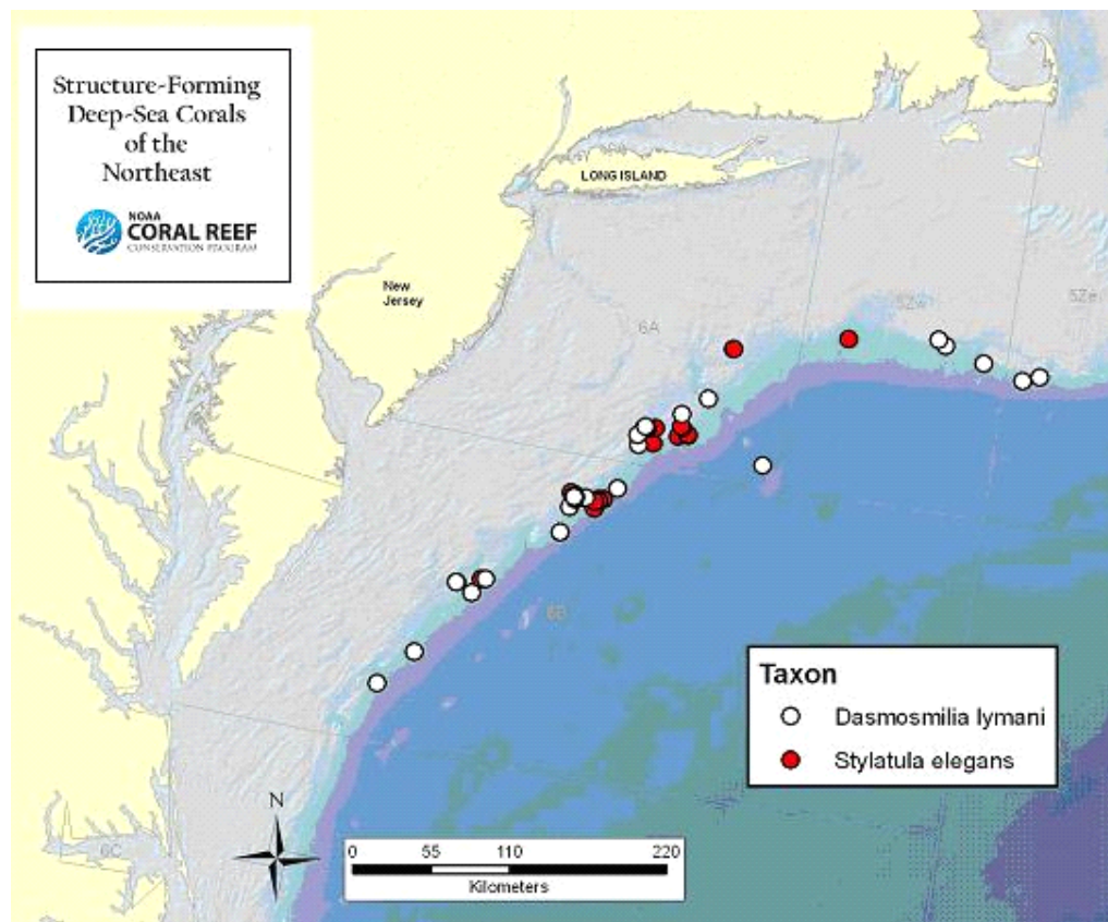
Figure 16. Location of the solitary cup coral Dasmosmilia lymani and the white sea pen coral Stylatula elegans as determined from museum records and other collections extracted from the Smithsonian Museum of Natural History online database http://www.nmnh.si.edu/iz .
