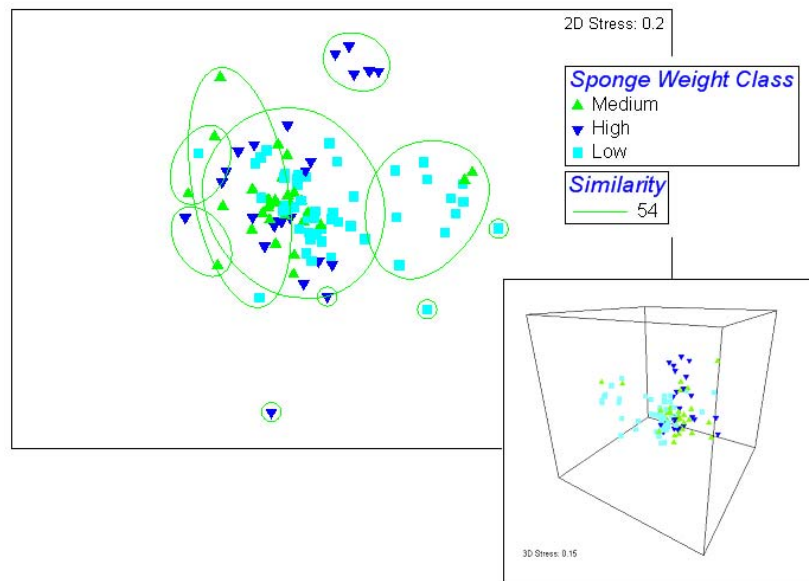
Figure 2. MDS configuration of the trawl catches (2001–2007) in 2D and 3D based on Bray–Curtis similarity matrix calculated from log 10 -transformed biomass data for each of 34 taxa. Trawl catches are labelled according to Sponge Weight Class. In the 2D representation stations with 54% similarity to each other are indicated. This is the average similarity level within each of the 3 classes.
