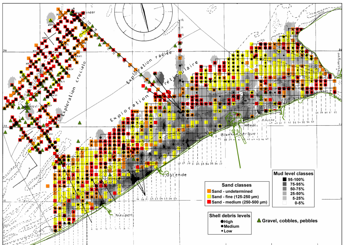
Figure: integrated map of raw sediment parameters extracted from sample descriptions and calibrated by means of grain size analysis. See Houziaux et al. in press for details.
