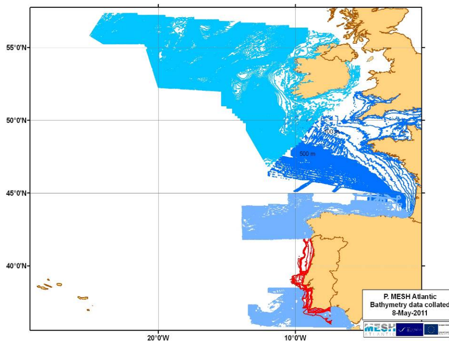
Collated bathymetry coverage as of April 2011.
