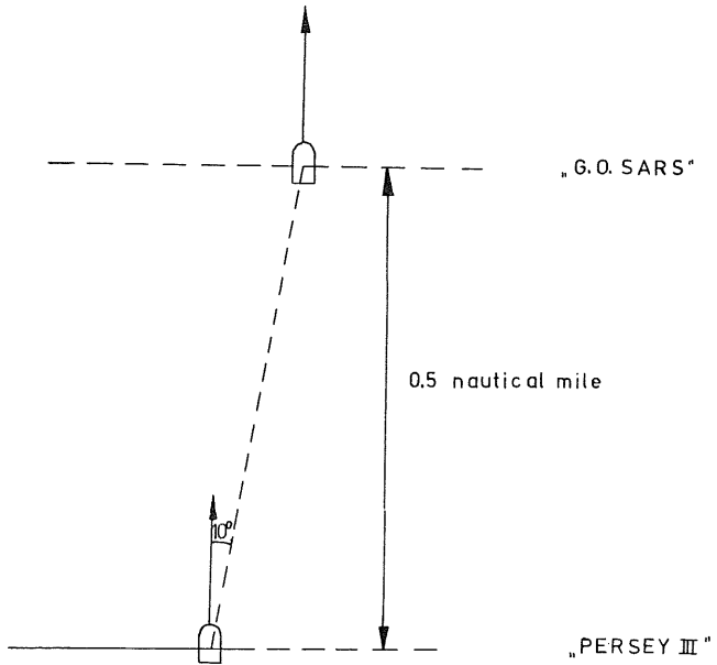
Annex Figure 1. Sailing positions during the intercalibration between "G. O. Sars" and "Persey III".
