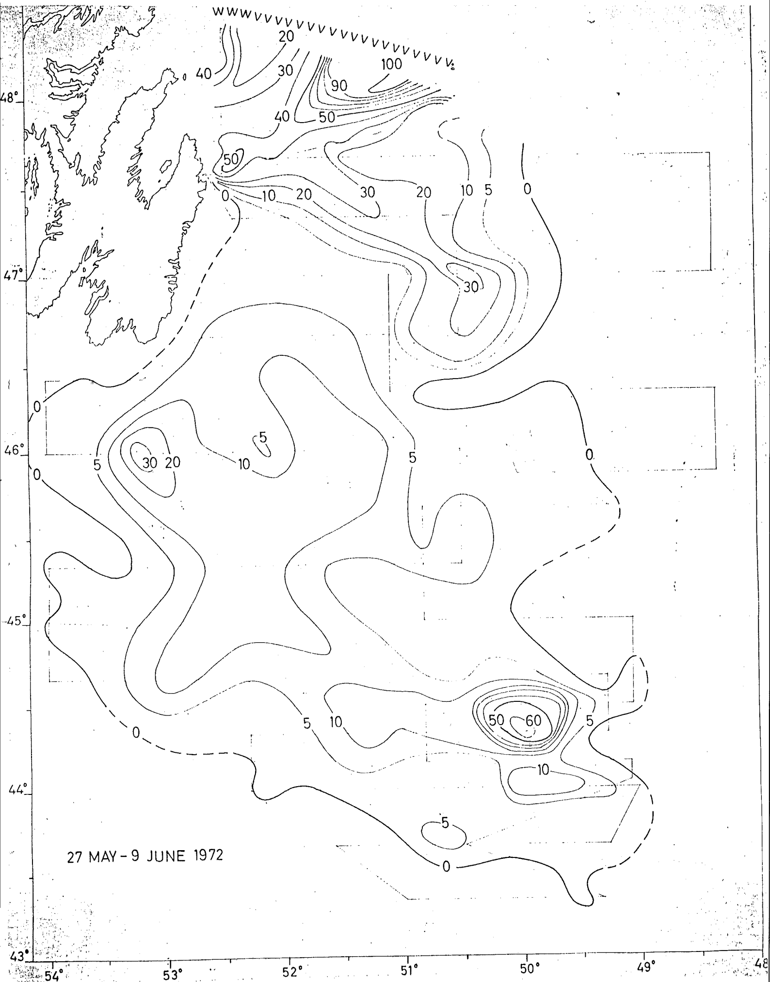
Fig. 4. Survey route and distribution of capelin 27 May - 9 June 1972. The isolines indicate echo integrator readings. The route taken from 7 to 9 June is the same as in Fig. 5.
