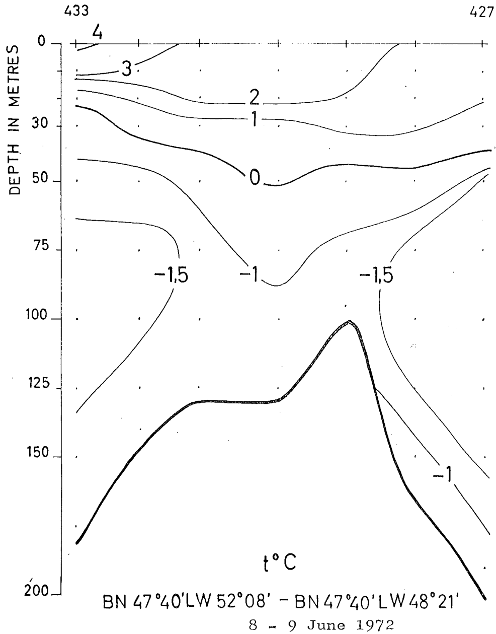
Fig. 8. Temperature in two sections on the Grand Banks in June 1972.
