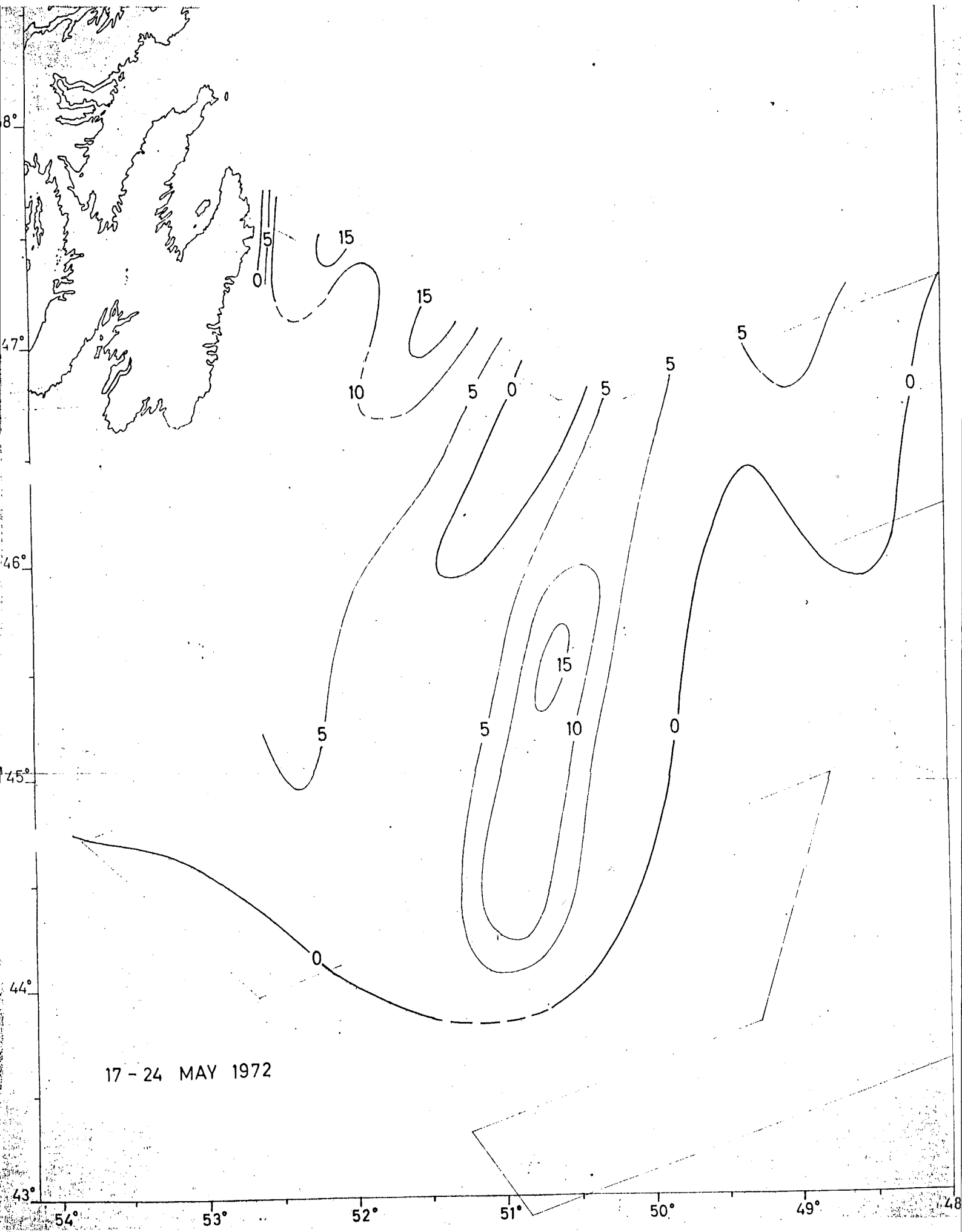
Fig. 3. Survey route and distribution of capelin 17-24 May 1972. The isolines indicate echo integrator readings.
