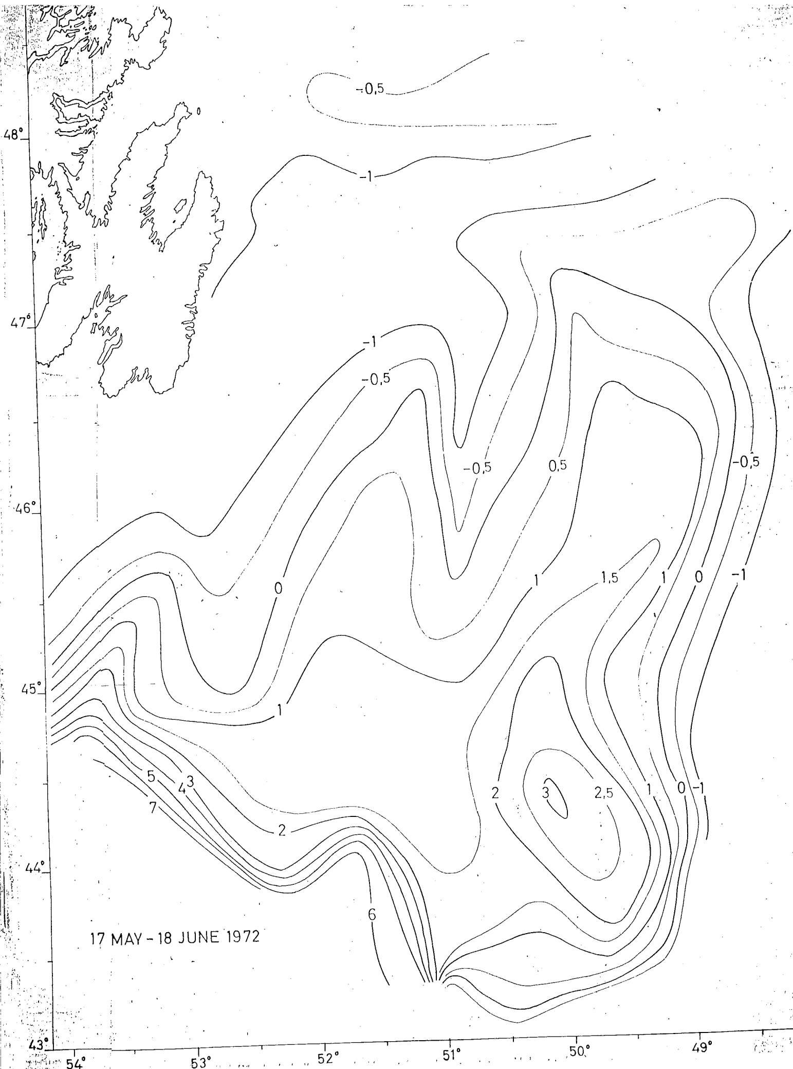
Fig. 7. Isotherms at the bottom 17 May - 18 June 1972.
