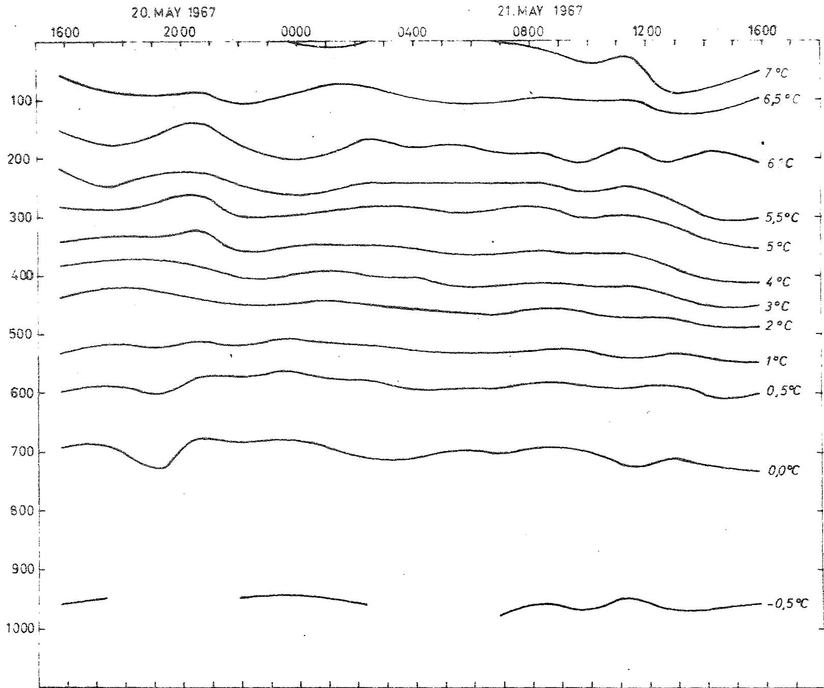
Fig. 26: Position 11. (Near buystation C) depth of isotherms.
