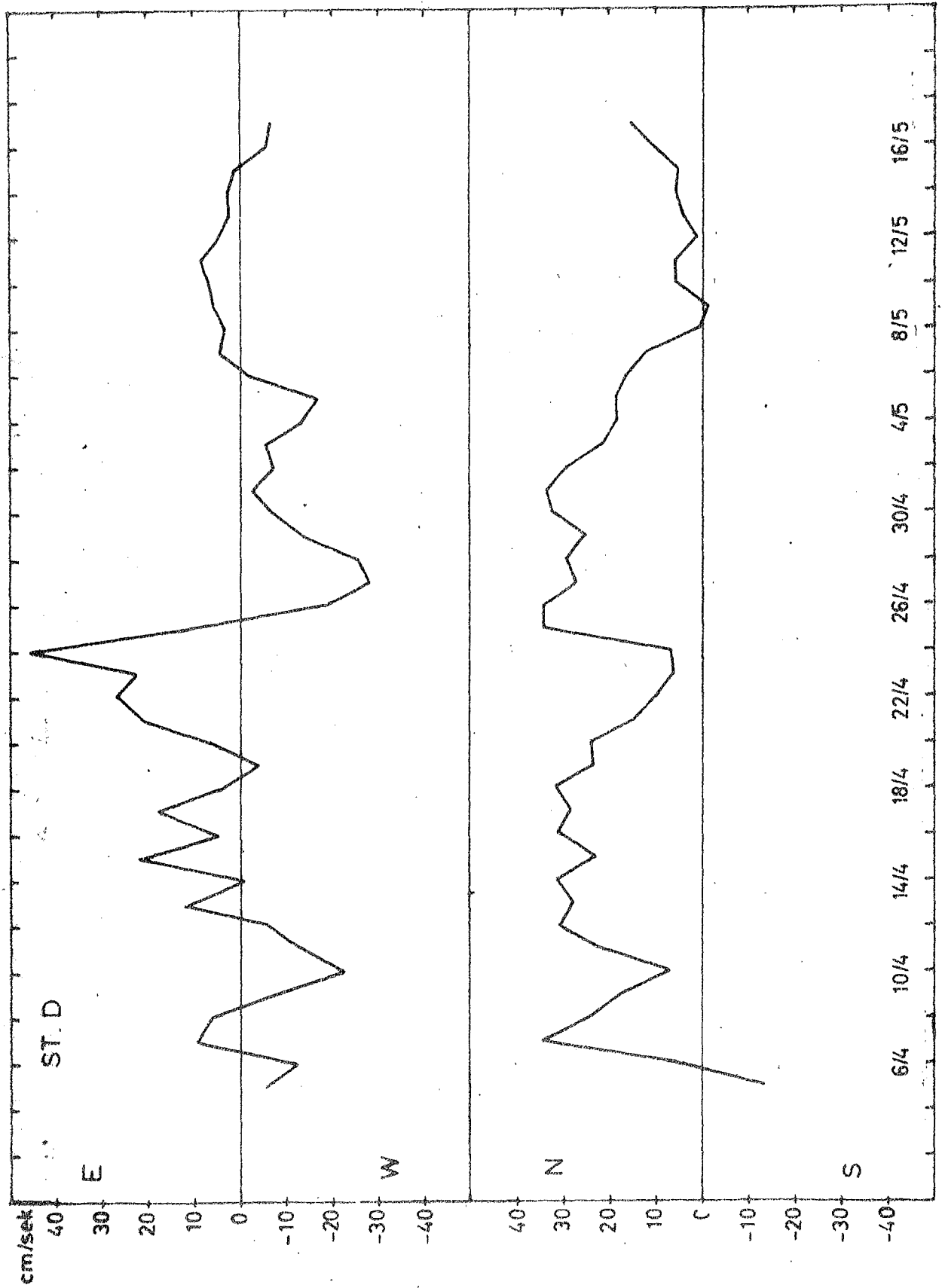
Fig. 17: Buoystation D. Daily mean current components
