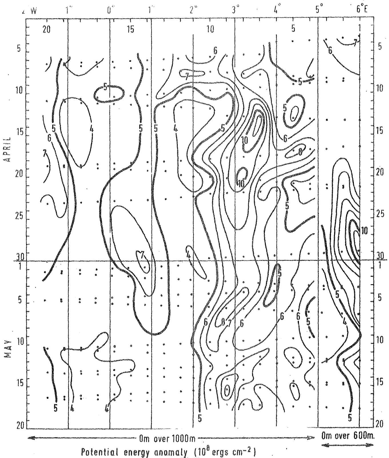
Fig. 24(a): 66^\circ\text{N} Section: 0m: Potential energy anomaly: 4 April-18 May 1967: The mass transport normal to the section between 0 and 1000 m depth and between successive isopleths equals 0.75 \times 10^6 tonnes \text{sec}^{-1} . If the isopleth with the higher number is to east the flow is north-going; if it is to the west the flow is south
