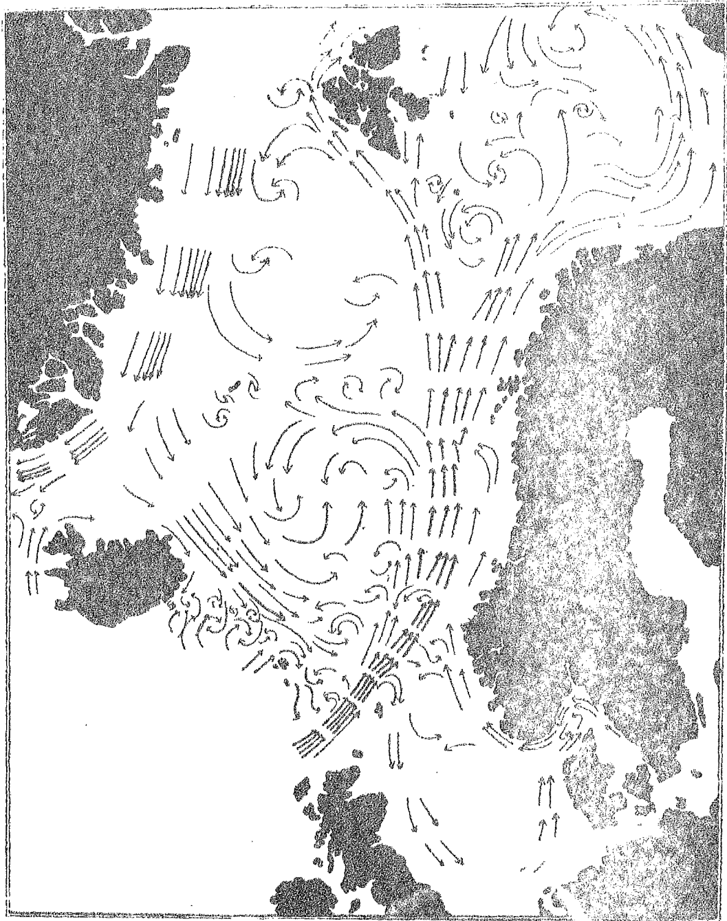
Fig. 9: General surface circulation in the southern part of the Norwegian Sea.
