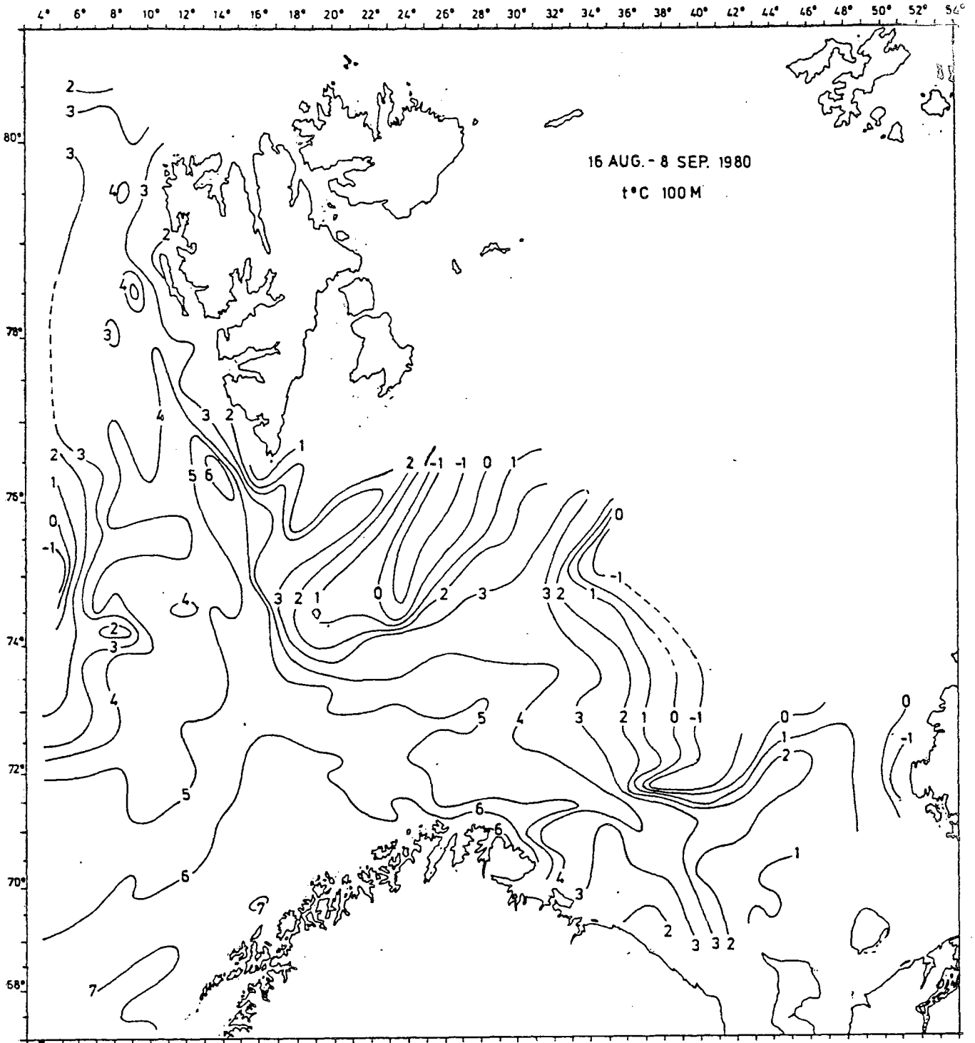
Fig. 4. Isotherms at 100 m.
