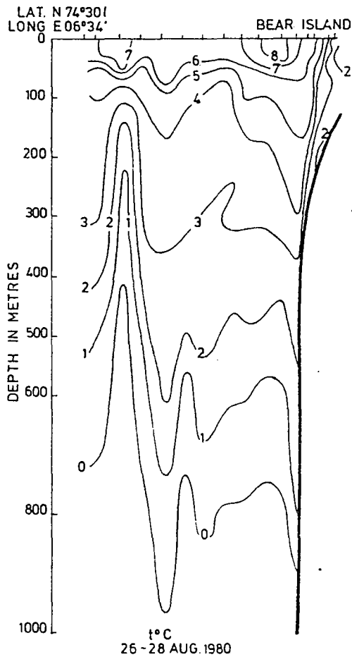
Fig. 8. Temperature section Bear Island - North Cape.
