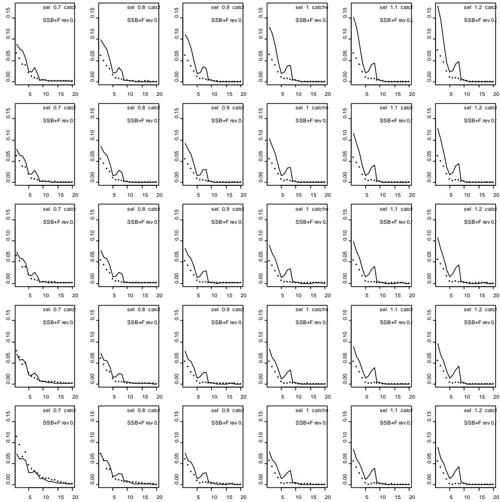
Figure 5.6.1.4. Herring in VIa (N). Mean squared deviation (y axis) between previous and current assessments for the 8 assessment years in the retrospective and years (x axis) previous to the terminal year in the assessment. 2009 WG data with varying weighting at age. SSB (dots) and F 3-6 (solid line). Across rows selection at oldest age ranging from 0.7 to 1.2, down columns weighting on catch from 2.0 to 0.5. Minimum is candidate for best settings (see text table section 5.6.1)
