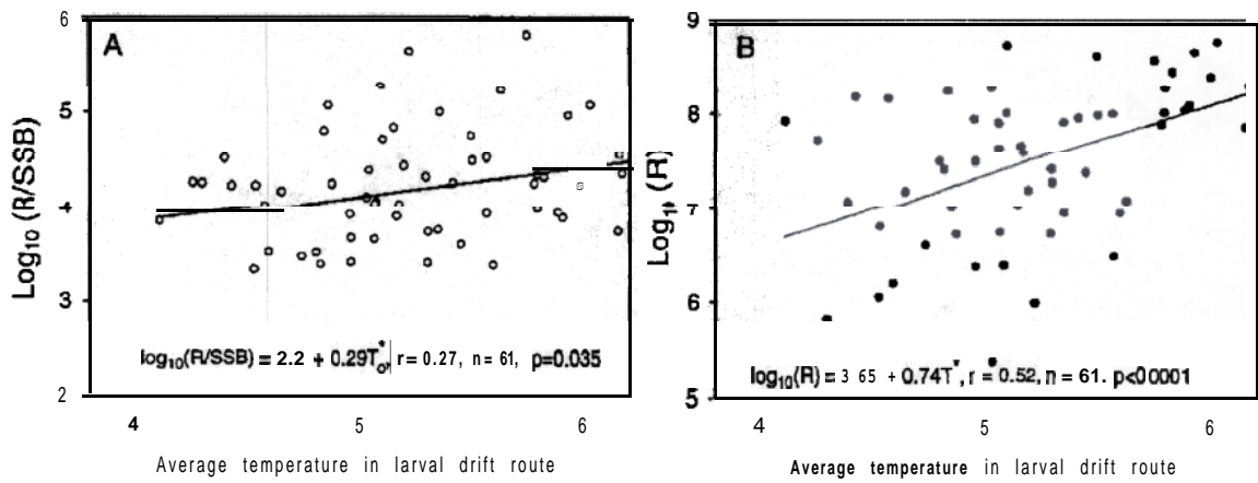
Fig. 4. This plot shows the average temperature in the drifting route of the larvae versus the recruitment (number of individuals 0 years old this year) for the period 1936-97. A : Recruits per spawner biomass. B : Total number of recruits.
