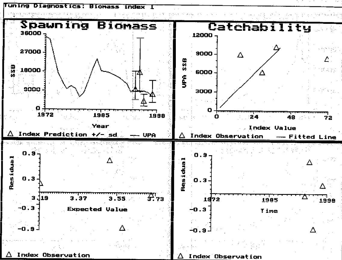
Figure 7.5.4. Herring in VIIa(N). Results of baseline assessment. Diagnostics of the fit of the larval abundance-index NINEL against the estimated spawning biomass. Top left, spawning biomass from the fitted populations (line), and predictions of spawning biomass in each year made from the index observations and estimated catchability (triangles =/ standard deviation), plotted by year. Top right, scatter plot and fitted relationship of spawning biomass from the fitted populations and larvae survey index observations. Bottom, residuals, as \ln(\text{observed index}) - \ln(\text{expected index}) plotted against expected values and against time.
