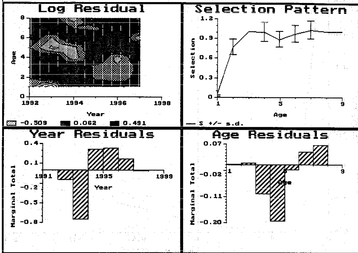
Figure 4.4.3. Herring in Celtic Sea and Div. VIIj Results of baseline assessment. Selection pattern diagnostics. Top left, contour plot of selection pattern residuals. Top right, estimated selection (relative to age 4) +/- standard deviation. Bottom, marginal totals of residuals by year and age.
