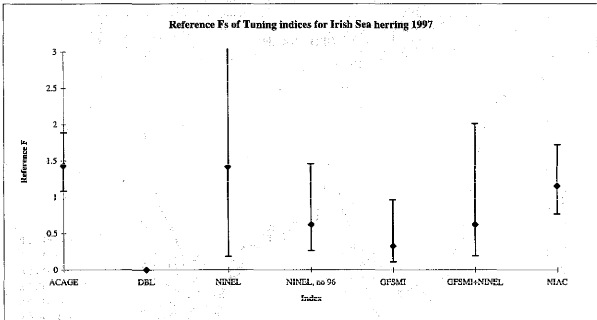
Figure 7.4.2. Herring Irish Sea VIIa(N): Tuning indices and reference F. 1 SD shown, see Table above for large confidence intervals.
