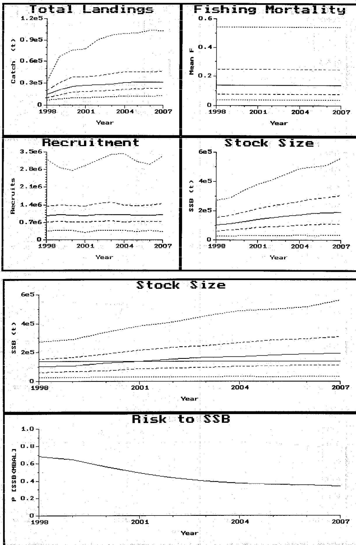
Figure 5.1.20 Herring in Division VIa(N). Medium-term projections based on the deterministic assessment assuming a constant fishing mortality at the level of 1996 ( F = 0.17 ). Dotted lines indicate the 5th and 95th percentiles, dashed lines indicate the 25th and 75th percentiles, unbroken line indicate median. Upper panel: Fishing mortality is the mean of ages 3 to 6. Recruitment is at age 0 and spawning stock biomass at spawning time. Lower panel: the trajectory of the spawning stock size and the risk that the spawning stock should fall below 140 000 t.
