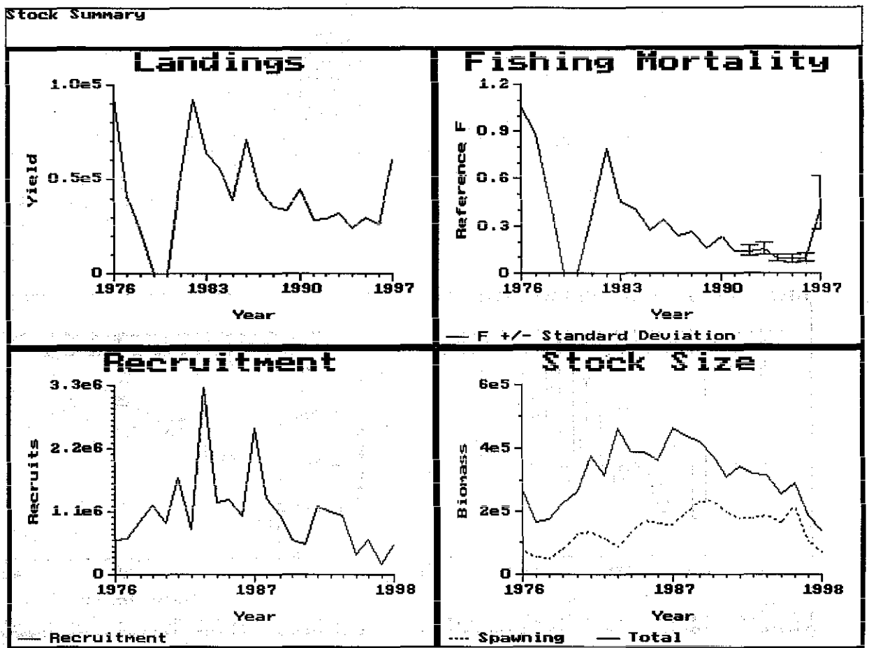
Figure 5.1.7. Herring in VIa(N). Results of deterministic assessment. Summary of estimates of landings, fishing mortality at age 4, recruitment at age 1, stock size on 1 January and spawning stock size at spawning time.
