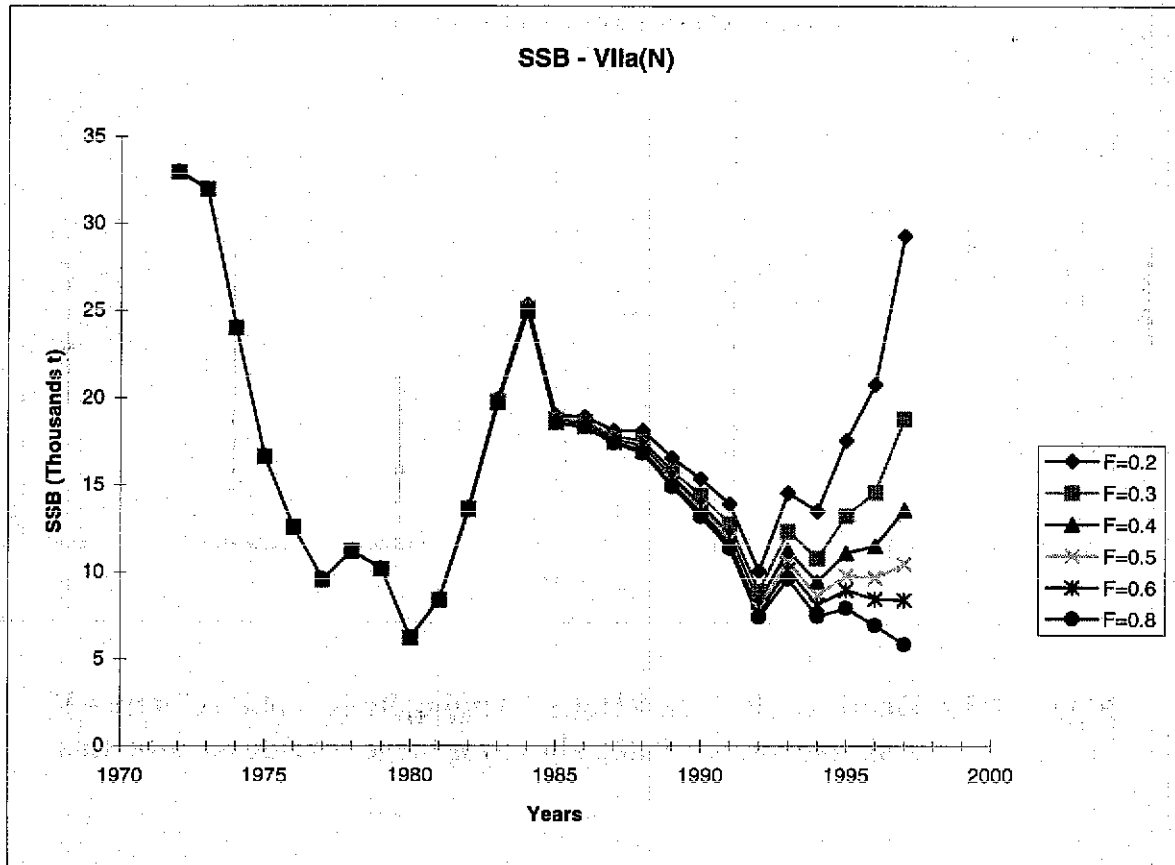
Figure 7.4.3. Herring Irish SEa Vila(N): SSB over a range of input F into a separable model.
