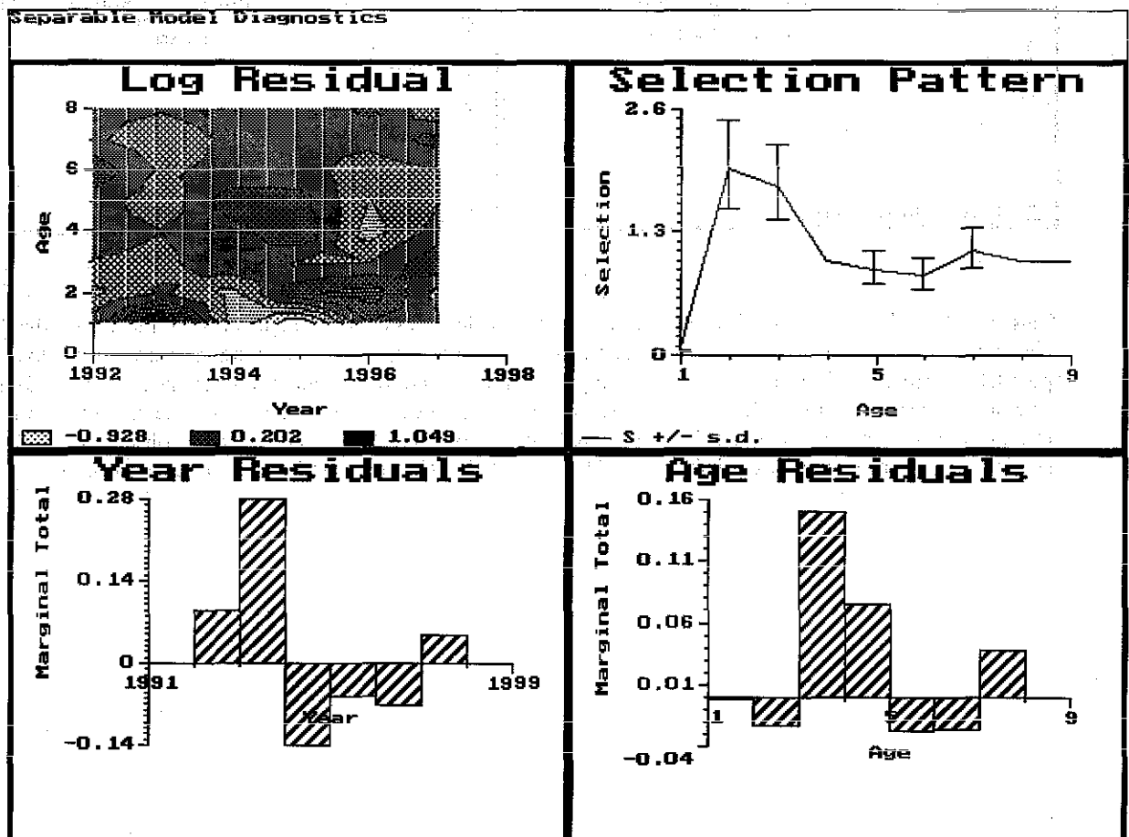
Figure 5.1.8. Herring in VIa(N). Results of deterministic assessment. Selection pattern diagnostics. Top left, contour plot of selection pattern residuals. Top right, estimated selection (relative to age 4) +/- standard deviation. Bottom, marginal totals of residuals by year and age.
