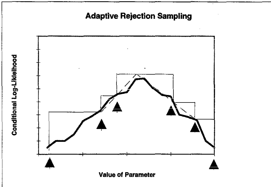
Appendix Figure 1. Construction of upper envelope function for adaptive rejection sampling. Bold line, conditional probability distribution of unknown form. Fine lines, constructed upper envelope function. Dashed line, construction lines. Arrows show the points at which the function has been evaluated. New points are added and the envelope readjusted until a sample has been taken from the conditional distribution, which typically takes 5 to 8 function evaluations.
