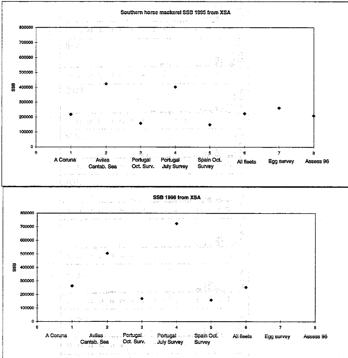
Figure 7.7.1.- SSB estimates in 1995 and 1996 by source of independent information and comparison with the last year assessment (Assess 96)
