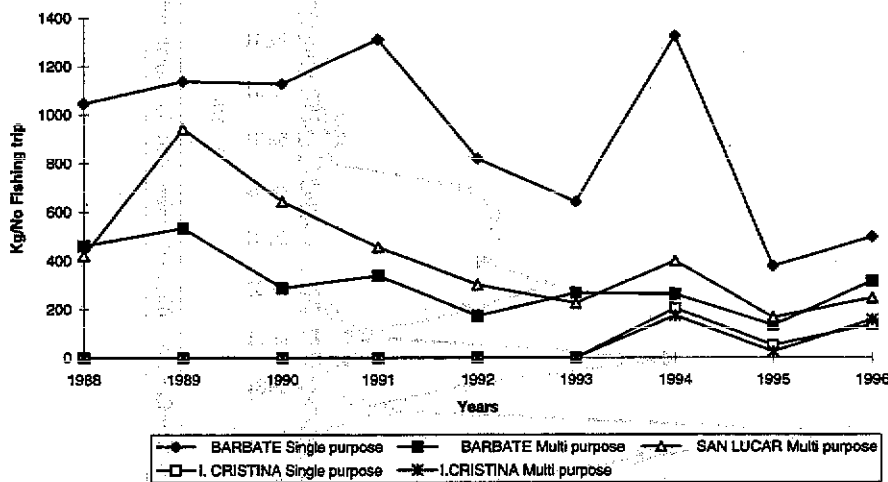
Figure 11.2.1 ANCHOVY in Division IXa. Spain IXa South (Bay of Cadiz) Effort and series in commercial fisheries.
