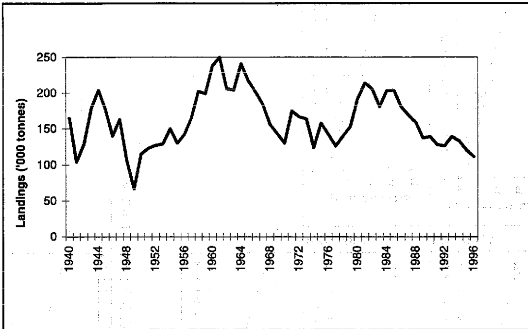
Figure 8.2.1 - Total landings of sardine in Divisions VIIIc and IXa from 1940-1996
