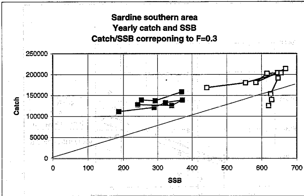
Figure 8.16.2 Yearly SSB and catch. Open symbols : Before 1985 Filled symbols: After 1985 - assumed separable selection pattern
