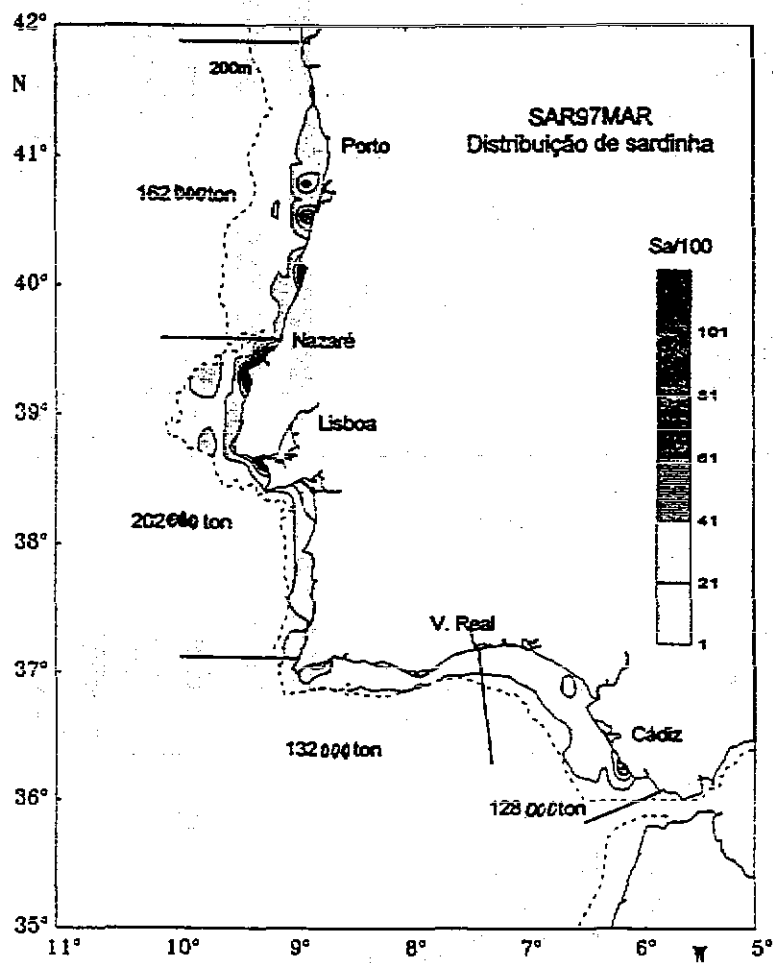
Figure 8.5.2 - Sardine - March 1997 acoustic surveys. Relative abundance distribution.
