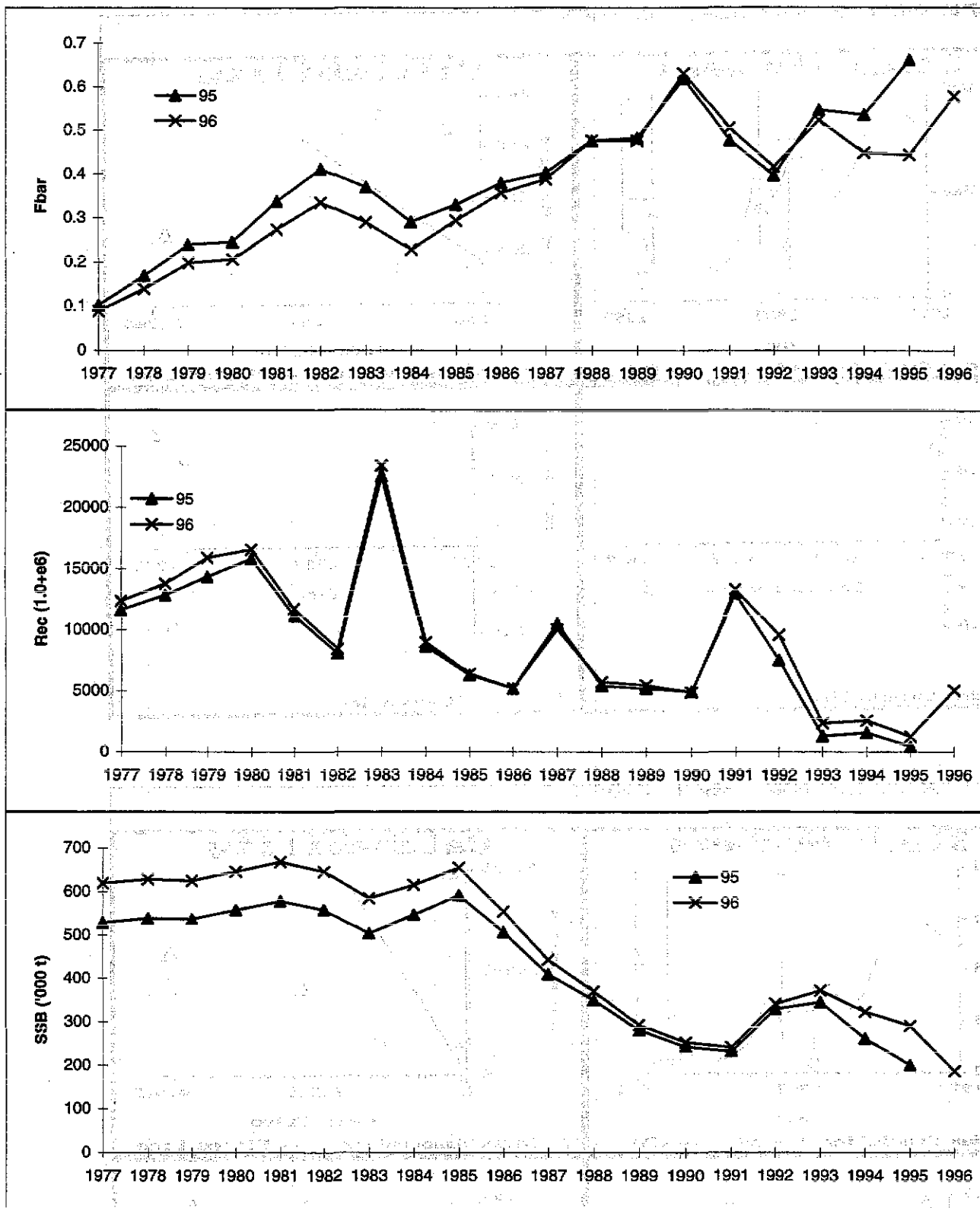
Figure 8.10.2: Fbar, Recruitment and SSB predictions in 1996 and 1997 assessments
