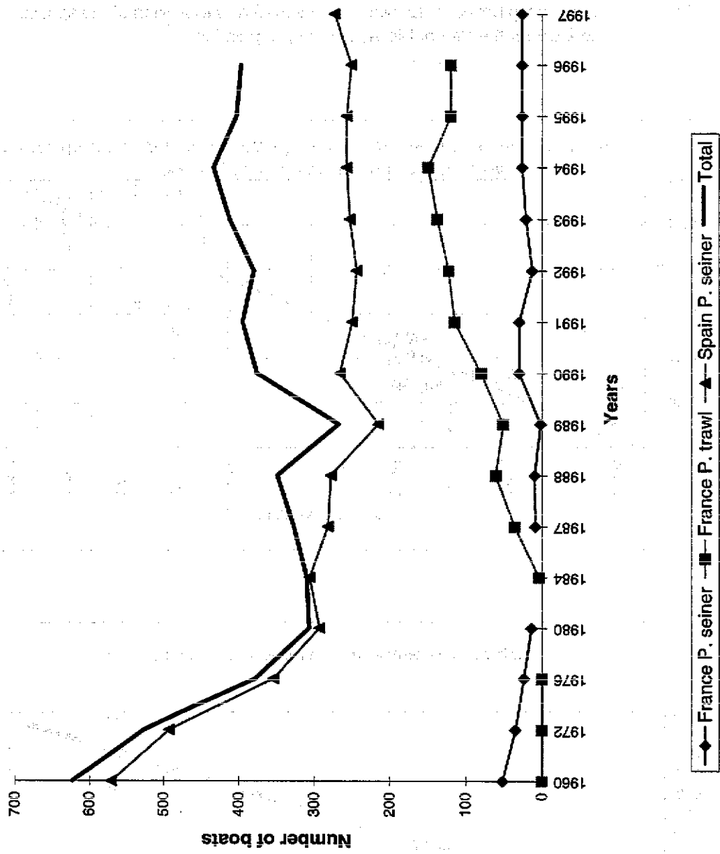
Figure 10.1.3: Evolution of the fleets fishing for anchovy in the Bay of Biscay
