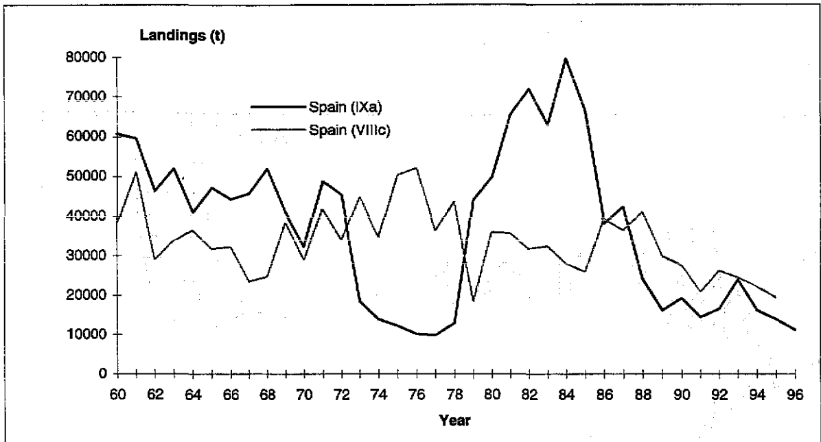
Figure 8.2.3 - Annual Spanish landings by ICES Division.
