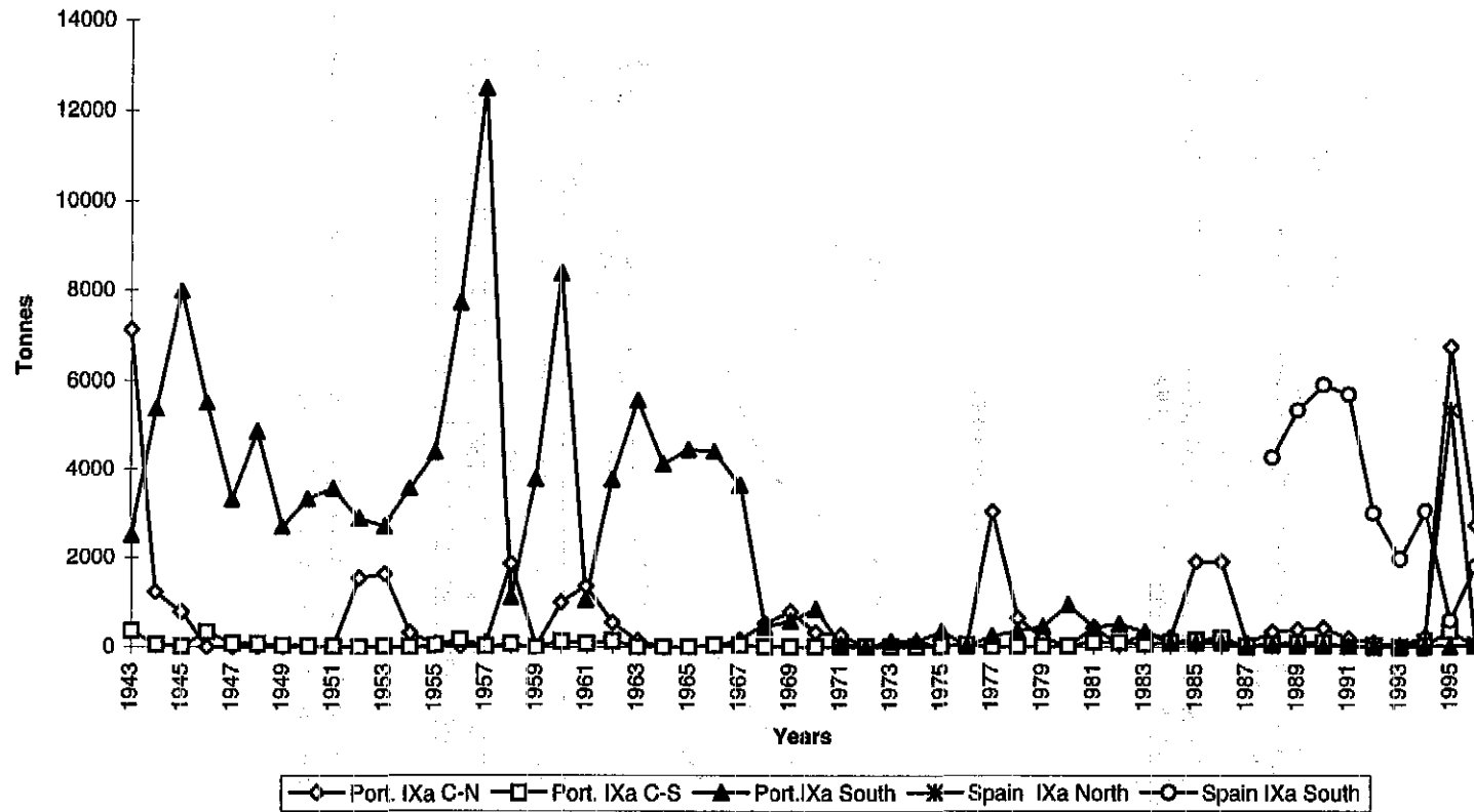
Figure 11.1.1: Portuguese and Spanish annual landings of ANCHOVY in Division IXa since 1943.
