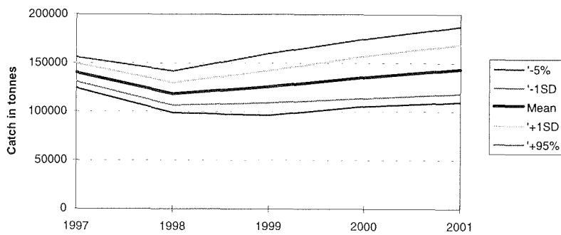
Figure 5.8A Quantiles of the catch in distribution, F_{new\_size}=0.33
