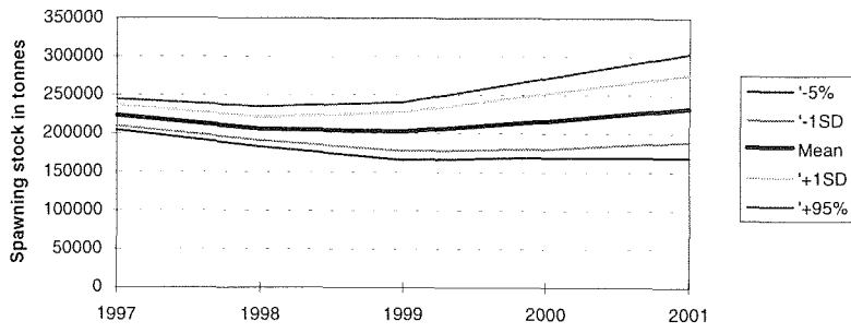
Figure 5.7A Quantiles of the SSB distribution, F_{new\_size}=0.33
