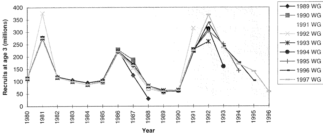
Figure 5.3C. North-East Arctic Saithe - Retrospective analysis
