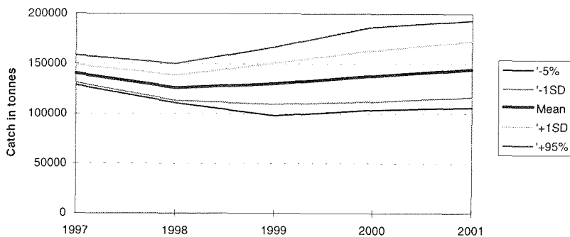
Figure 5.8B Quantiles of the catch indistribution, F_{new\_size}=0.36
