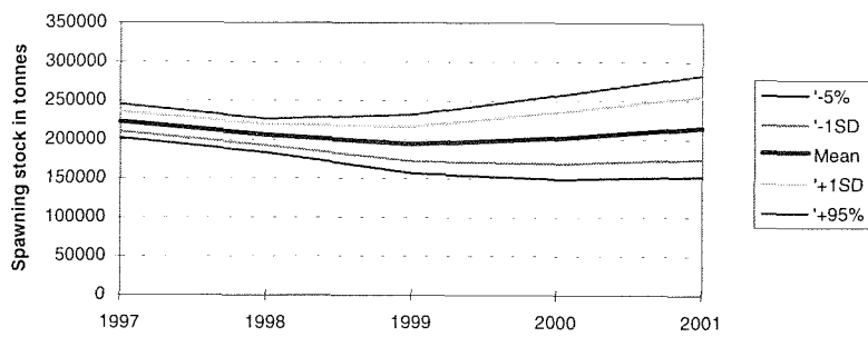
Figure 5.7B Quantiles of the SSB distribution, F_{new\_size}=0.36
