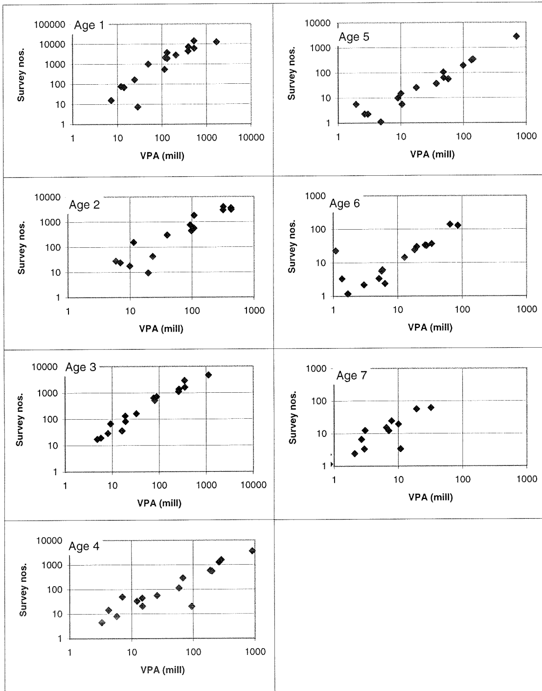
NE Arctic Haddock abundance index from the Norwegian bottom trawl survey plotted again VPA results on stock number at age
