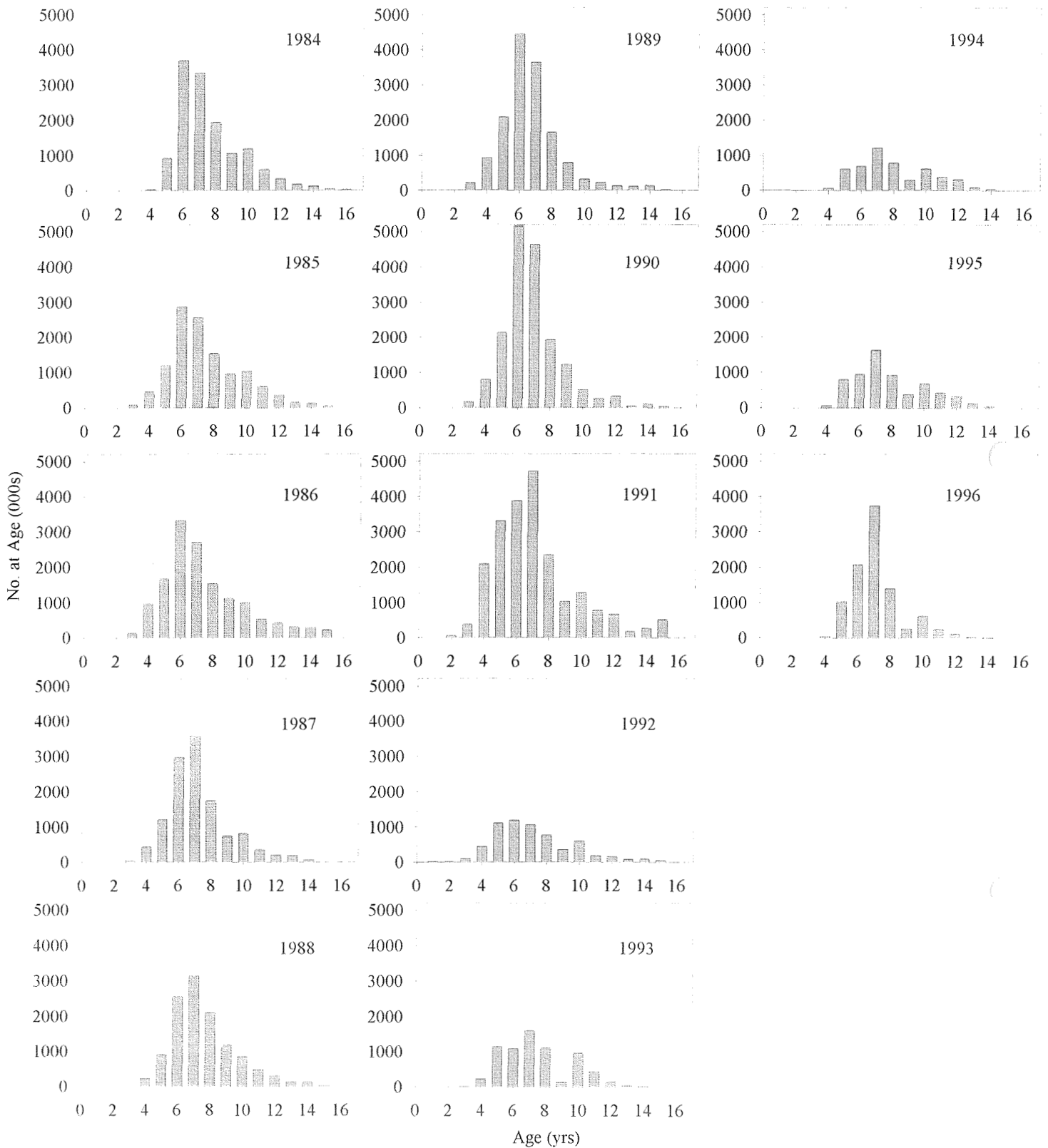
Figure 8.3 Catch numbers at age (000s) of Greenland halibut from the commercial fishery in ICES Regions I and II.
