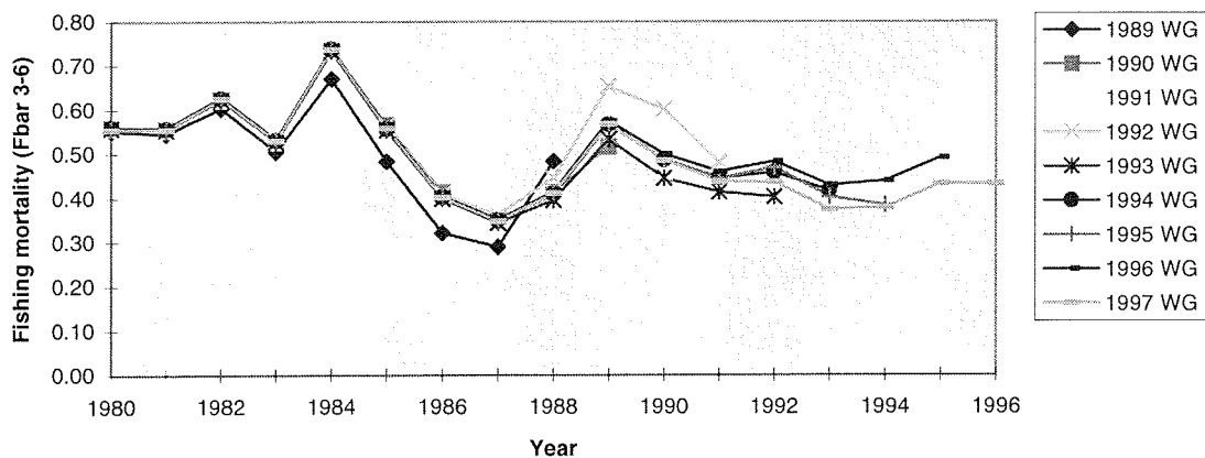
Figure 5.3A. North-East Arctic Saithe - Retrospective analysis
