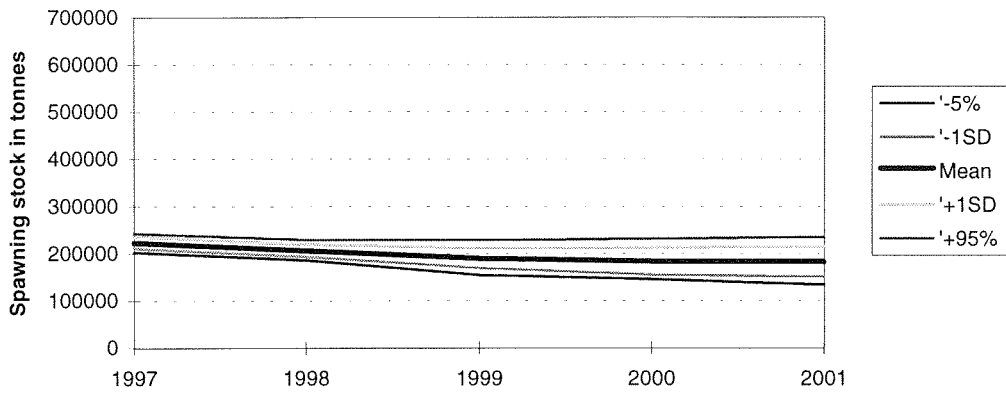
Figure 5.5D Quantiles of the SSB distribution, F_{sq}=0.4325
