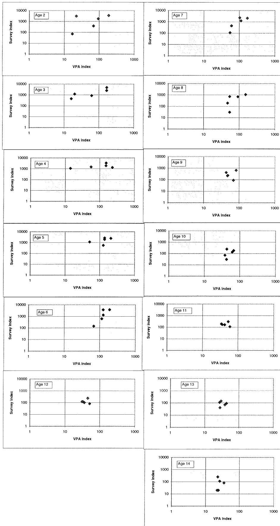
Figure 6.3D. Sebastes mentella in Sub-areas I and II. Norwegian bottom trawl survey (Barents Sea) vs VPA
