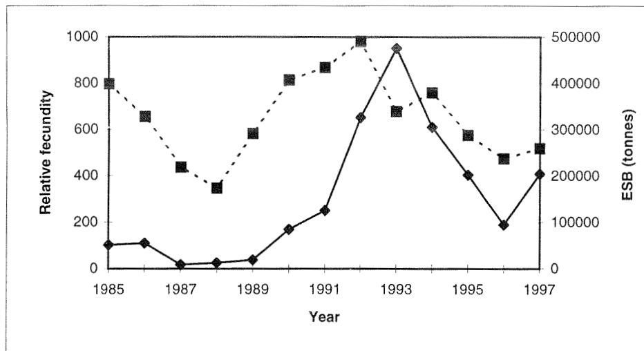
Figure 3.10: Relative fecundity of the stock (dashed line) and effective spawner biomass (solid line) for survey time period (1985-97).
