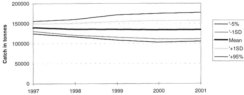
Figure 5.6D Quantiles of the catch distribution, F_{sq}=0.4325
