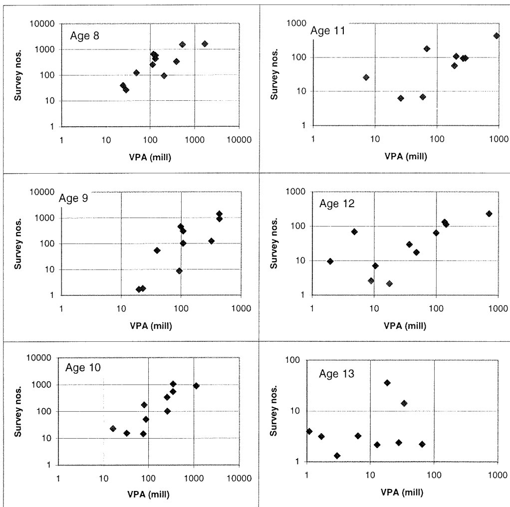
NE Arctic Haddock abundance index from the Norwegian bottom trawl commercial fleet plotted against VPA results on stock number at age
