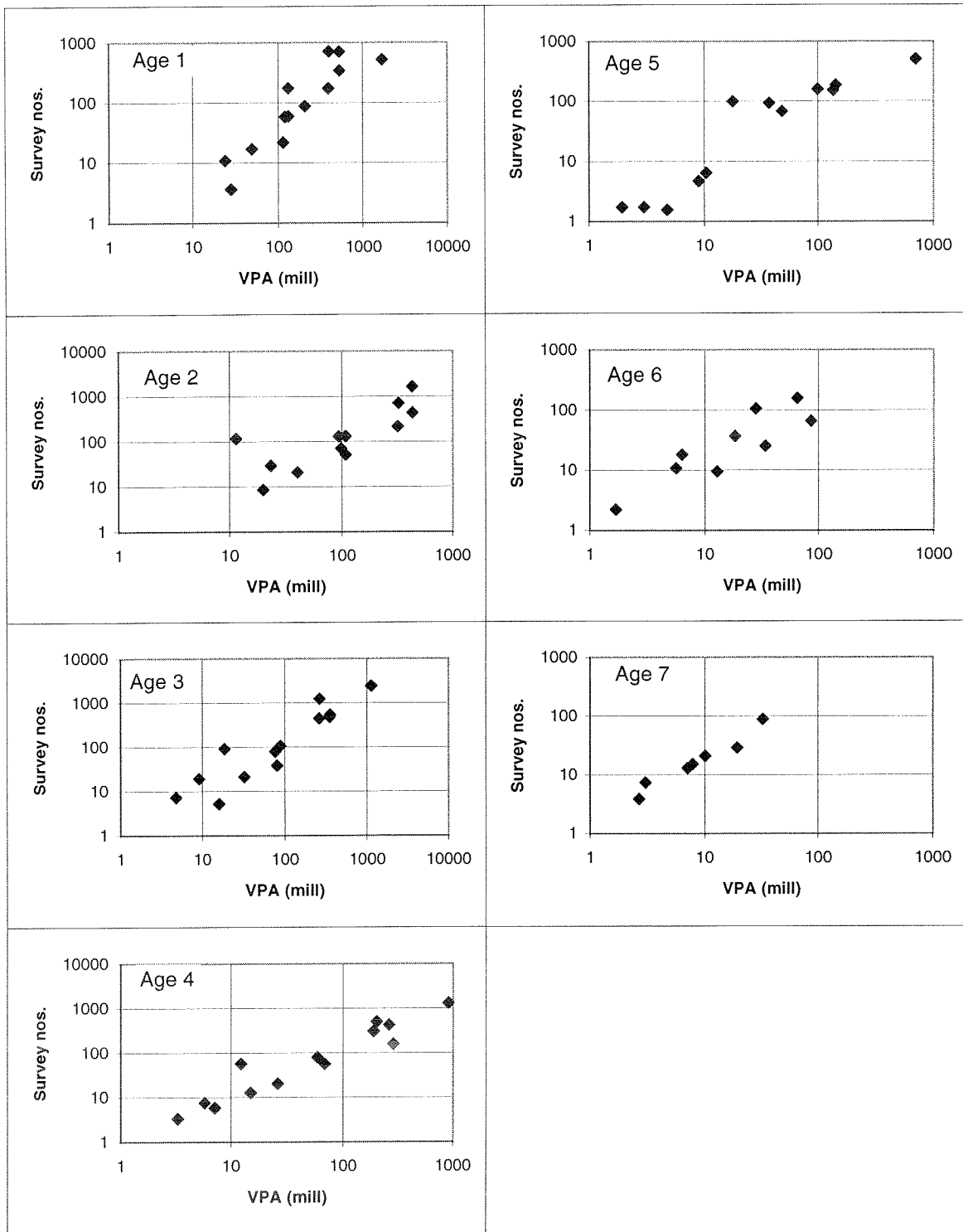
NE Arctic Haddock abundance index from the Russian bottom trawl survey plotted again VPA results on stock number at age
