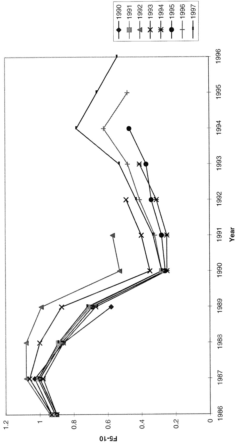
Fig. 3.5A Retrospective analysis NEA cod. qage = 4
