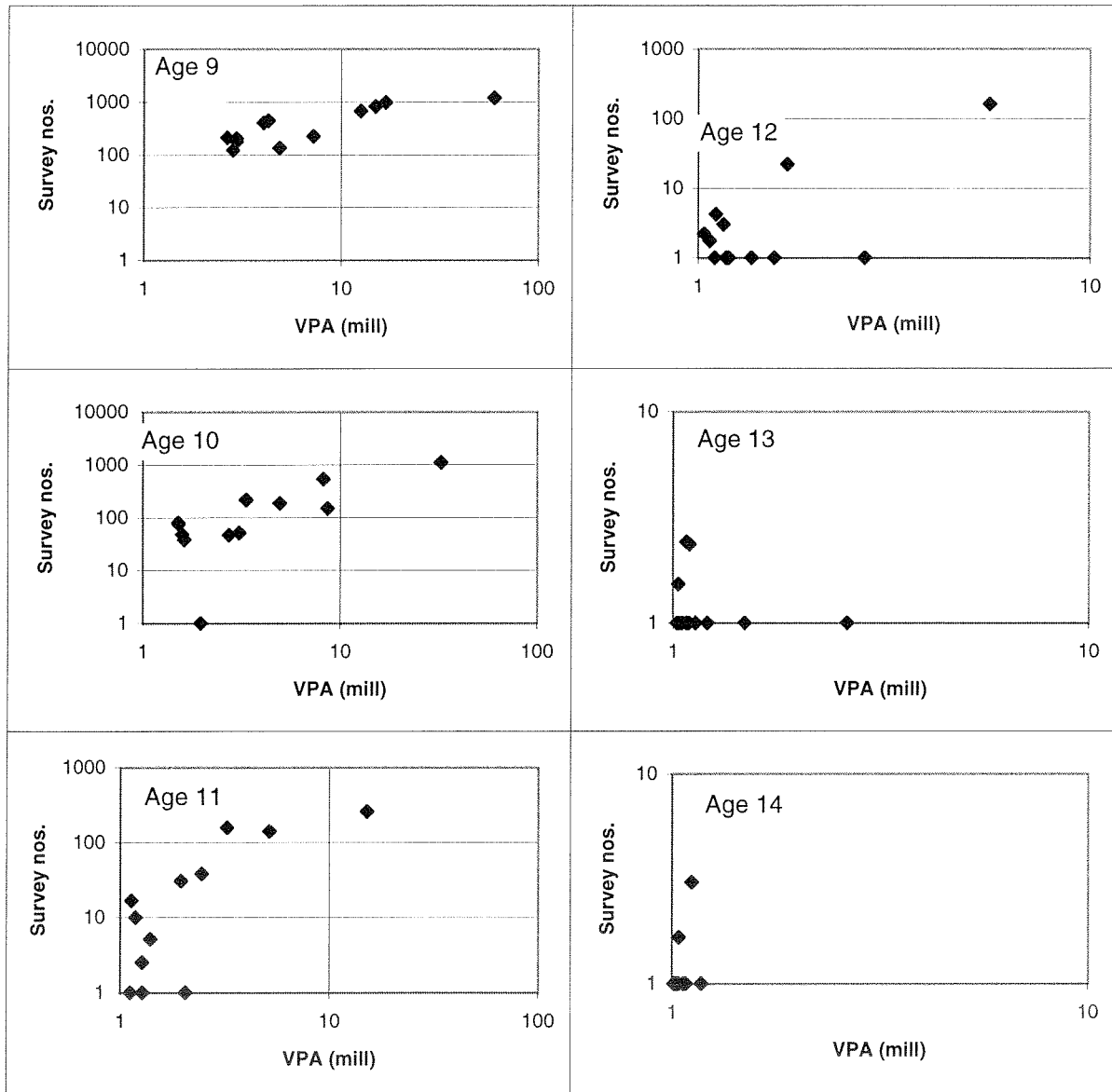
Figure 3.2 D. (FLT 53) NE Arctic Cod abundance index from the Russian trawl, catch and effort commercial fleet plotted against VPA results on stock number at age
