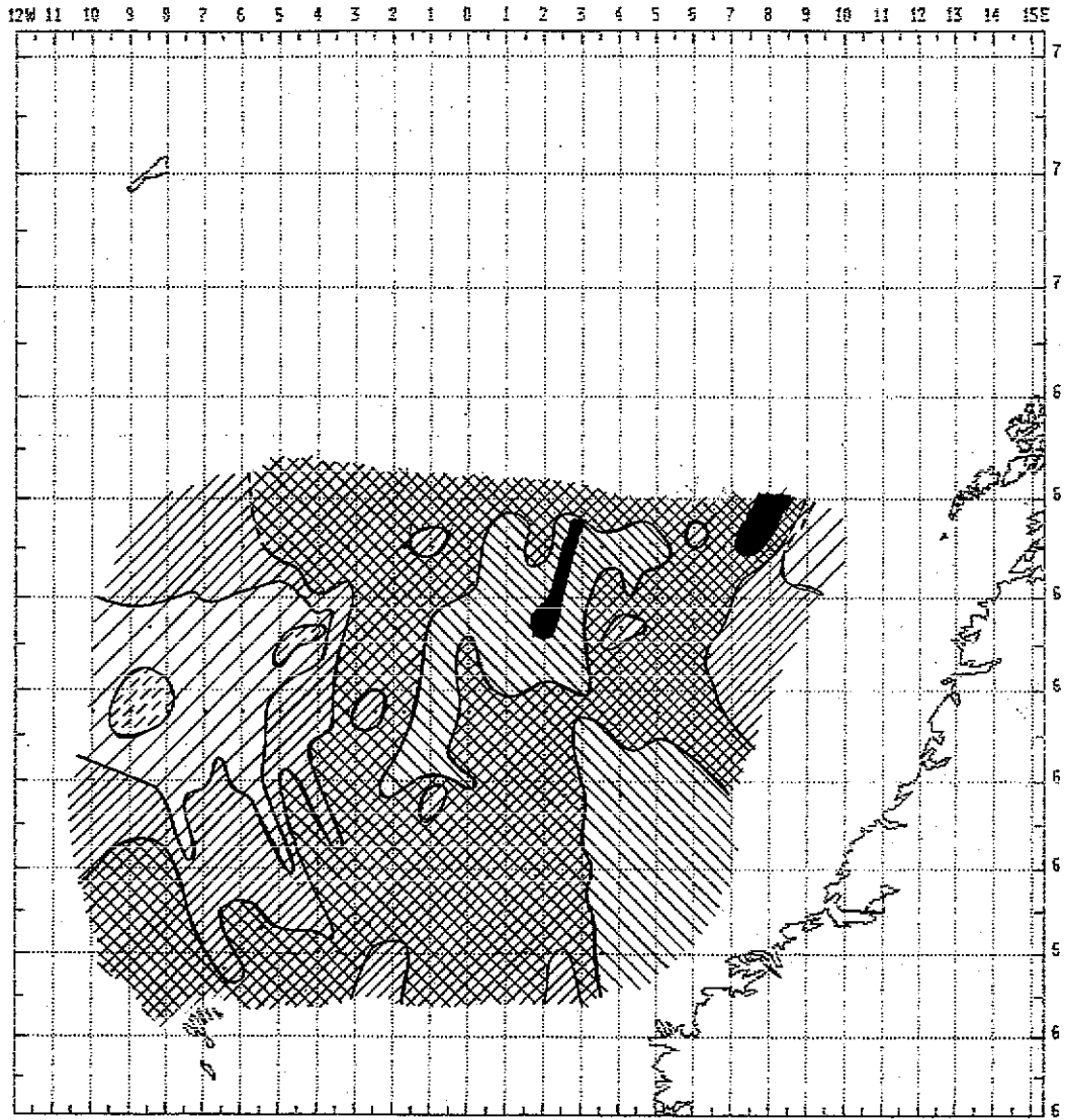
Fig. 14 Plankton biomass distribution 0-50 m layer in the Norwegian sea in June 1998. Jedy net's catches
