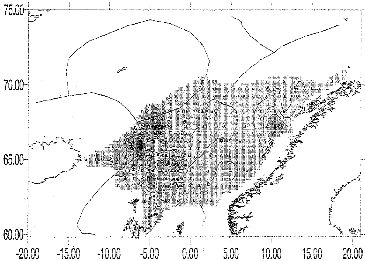
Figure 13. Zooplankton biomass in mg dryweight per m 2 in upper 200 m, May 1997. Sampling positions indicated.
