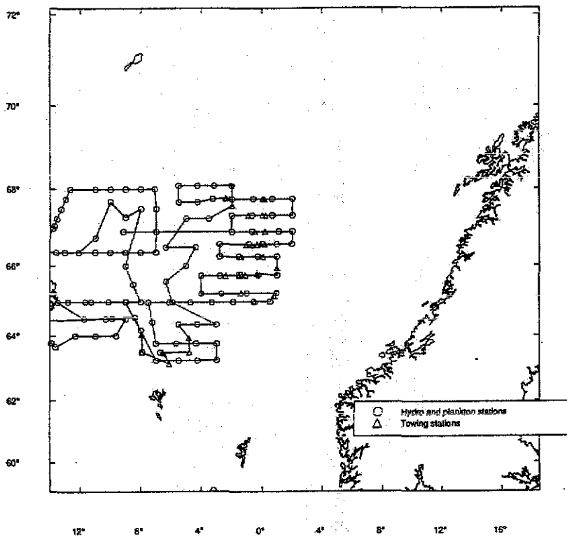
Figure 2. Survey transects of R/V «Arni Fridriksson» and R/V "Bjarni Sæmundsson", May 1998.
