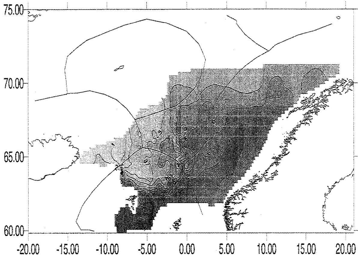
Figure 11. Temperatures in 50 m, May 1997.
