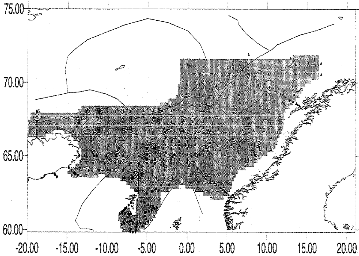
Figure 12b Zooplankton biomass in mg dryweight per m 2 in upper 200 m, May 1998. Sampling positions indicated.
