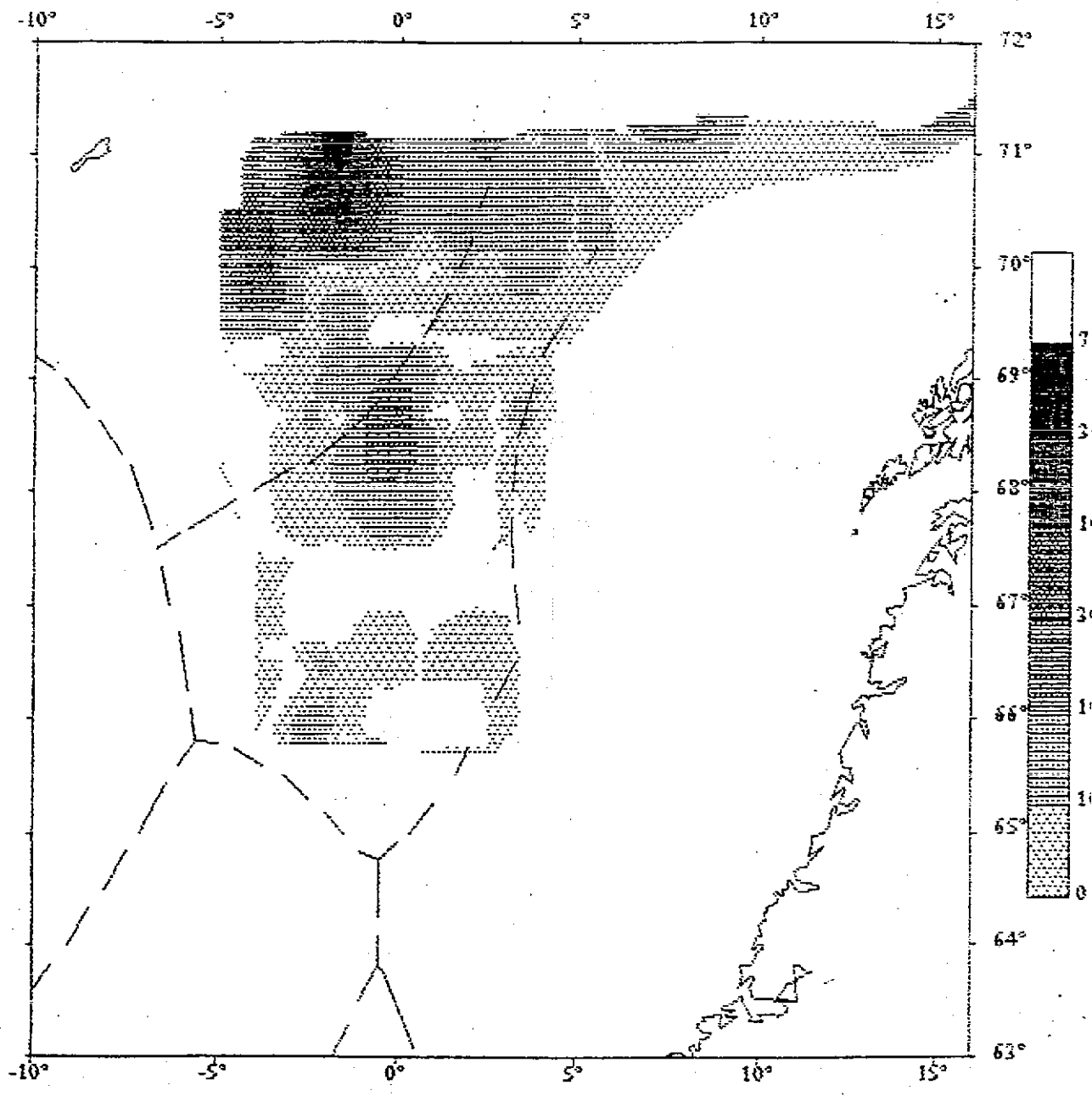
25 Fig. Distribution of Herring in the Norwegian Sea in the Norwegian Sea in July 1998, Sa refer to integrator values.
